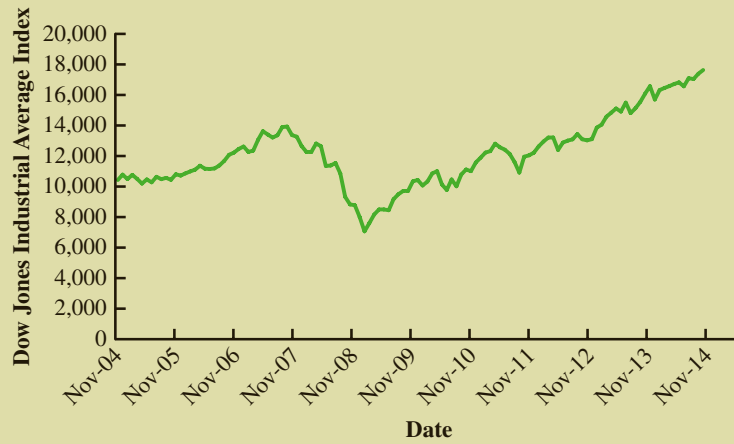
(A) Dow Jones Industrial Average Index
