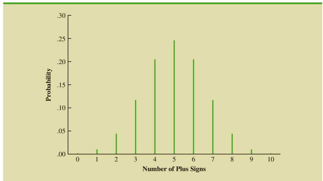
FIGURE 18.1 BINOMIAL SAMPLING DISTRIBUTION FOR THE NUMBER OF PLUS SIGNS WHEN n = 10 AND p = .50
