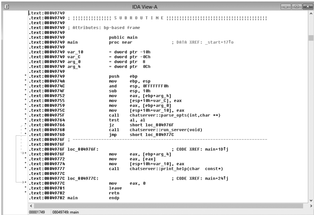
Figure 6-9: Disassembly with debug symbols
