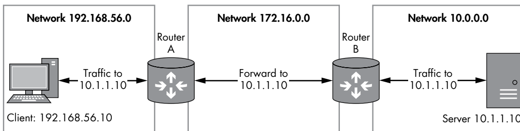
Figure 4-1: An example of routed traffic
