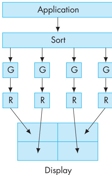
FIGURE 11.27 Sort-first rendering.
