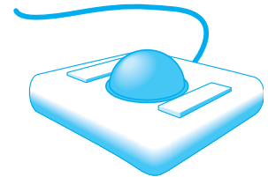
FIGURE 1.7 Trackball.
