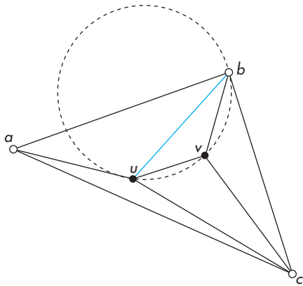
FIGURE 10.56 Mesh after flipping.
