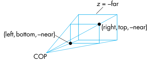
FIGURE 4.40 OpenGL perspective.
