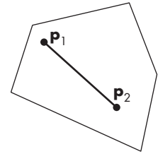
FIGURE 2.11 Convexity.
