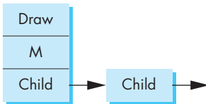
FIGURE 8.11 Node representation.
