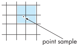
FIGURE 7.20 Texels used with linear filtering.
