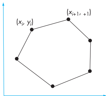
FIGURE 6.48 Computing the area of a polygon.
