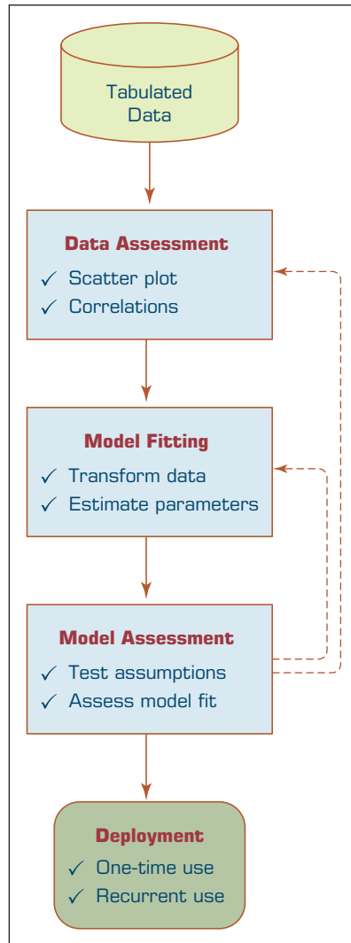
FIGURE 2.14 A Process Flow for Developing Regression Models.
