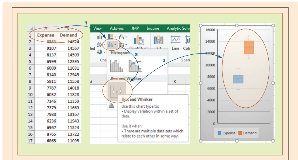
FIGURE 2.12 Creating a Box-and-Whiskers Plot in Excel 2016.
