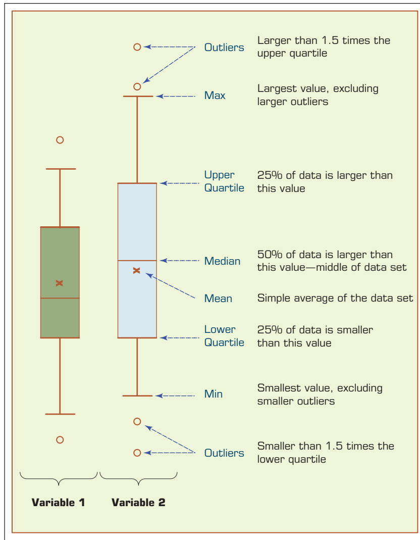
FIGURE 2.8 Understanding the Specifics about Box-and-Whiskers Plots.
