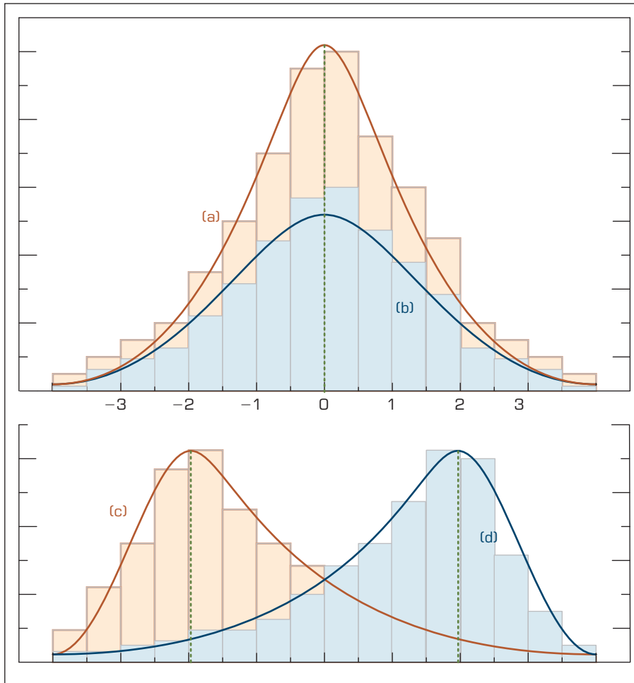
FIGURE 2.9 Relationship between Dispersion and Shape Properties.
