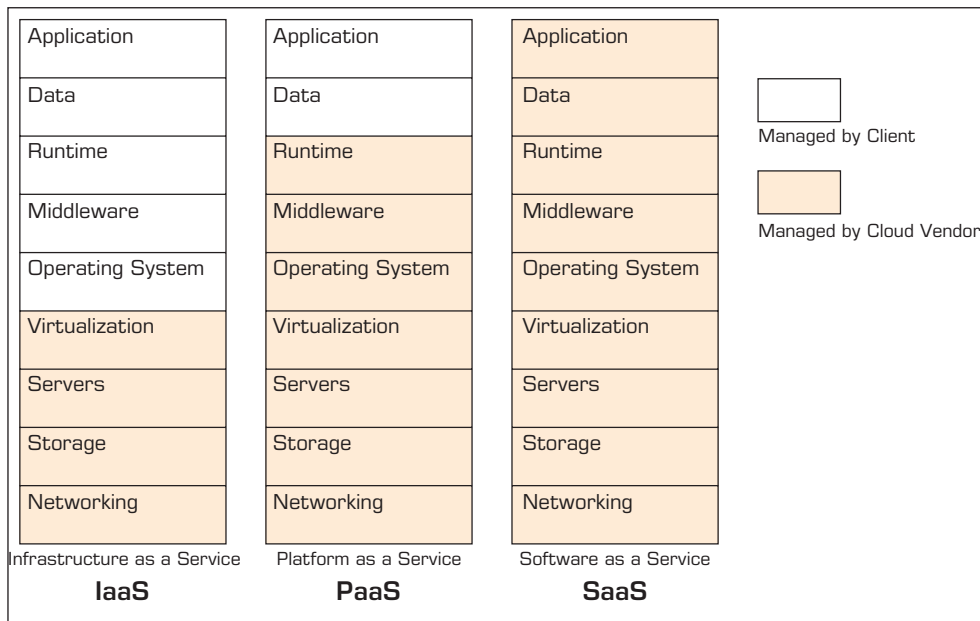
FIGURE 8.5 Technology Stack as a Service for Different Types of Cloud Offerings.
