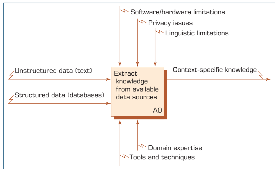
FIGURE 5.5 Context Diagram for the Text Mining Process.
