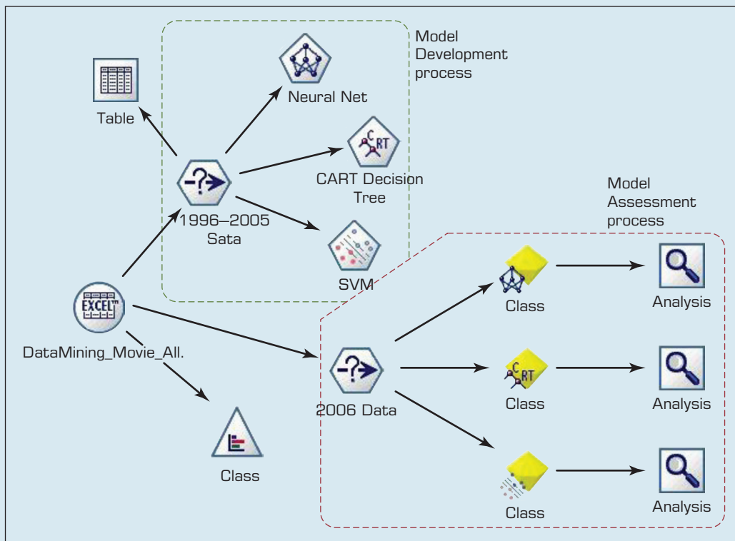
FIGURE 4.16 Process Flow Screenshot for the Box-Office Prediction System. Source: Used with permission from IBM SPSS.
