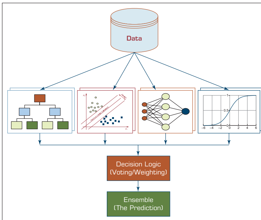
FIGURE 4.12 Graphical Illustration of a Heterogeneous Ensemble.
