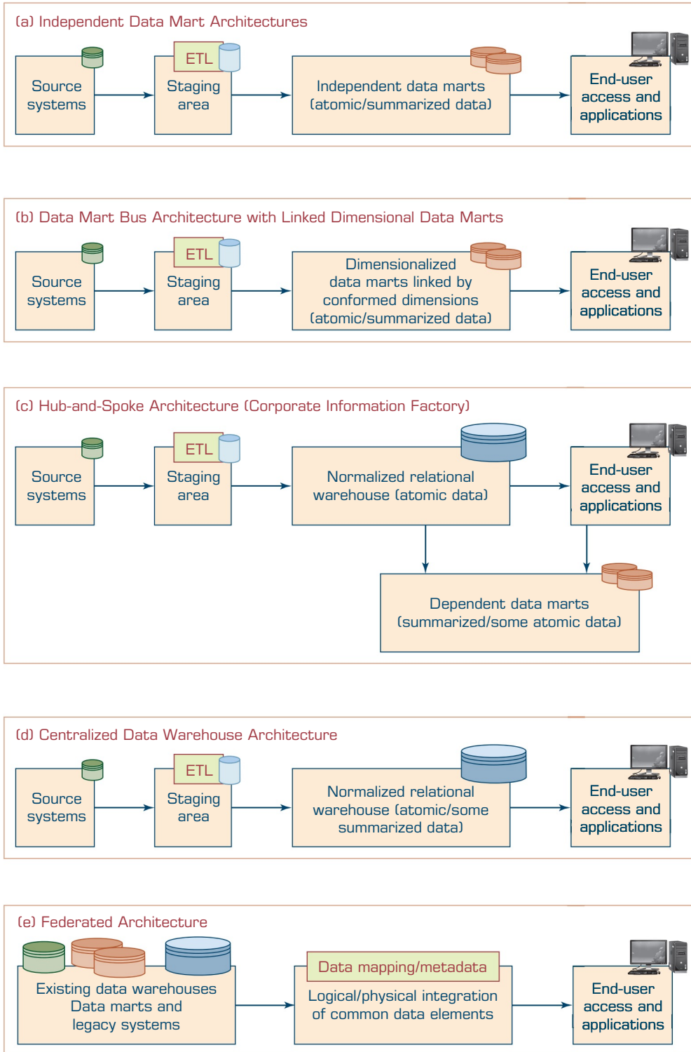
FIGURE 3.8 Alternative Data Warehouse Architectures. Source: Adapted from Ariyachandra, T., & Watson, H. (2006b). Which data warehouse architecture is most successful? Business Intelligence Journal , 11(1), 4–6.
