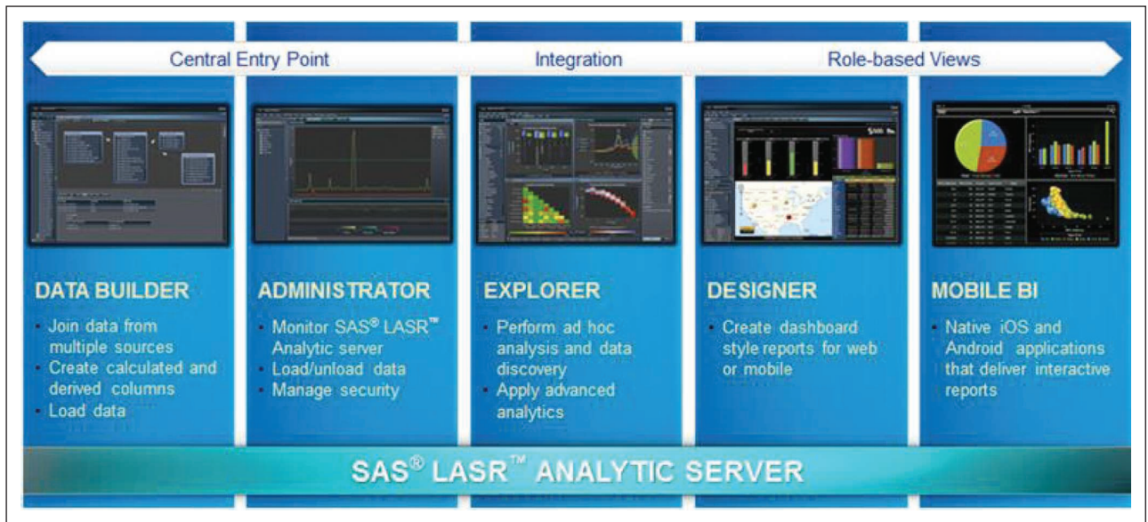
FIGURE 2.25 An Overview of SAS Visual Analytics Architecture. Source: SAS.com.
