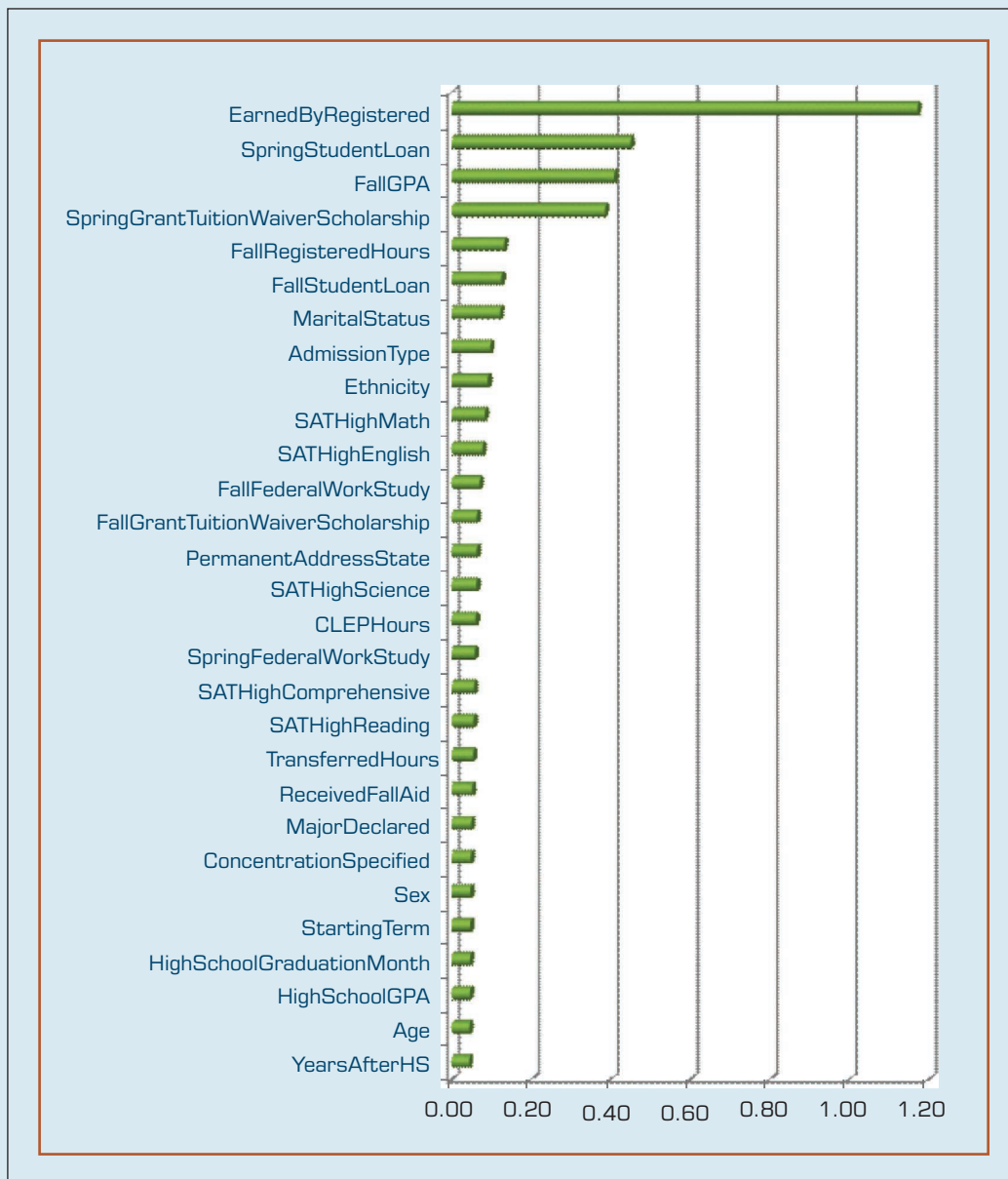
FIGURE 2.6 Sensitivity-Analysis-Based Variable Importance Results.
