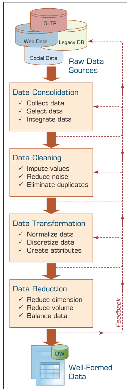
FIGURE 2.3 Data Preprocessing Steps.
