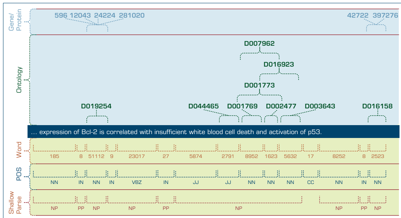
FIGURE 5.4 Multilevel Analysis of Text for Gene/Protein Interaction Identification. Source: Based on Nakov, P., Schwartz, A., Wolf, B., & Hearst, M. A. (2005). Supporting annotation layers for natural language processing. Proceedings of the Association for Computational Linguistics (ACL) , Interactive Poster and Demonstration Sessions, Ann Arbor, MI. Association for Computational Linguistics, 65–68.
