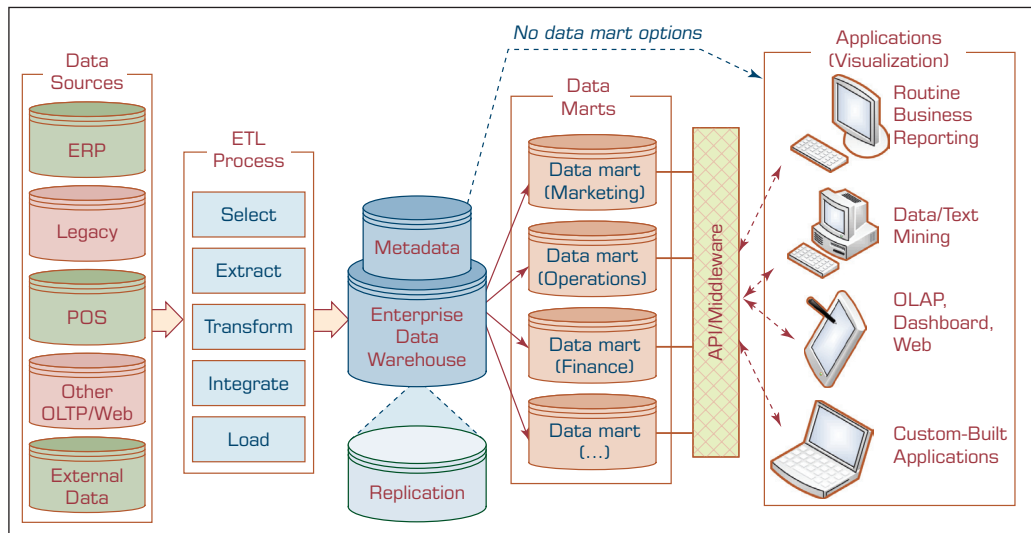
FIGURE 3.4 A Data Warehouse Framework and Views.
