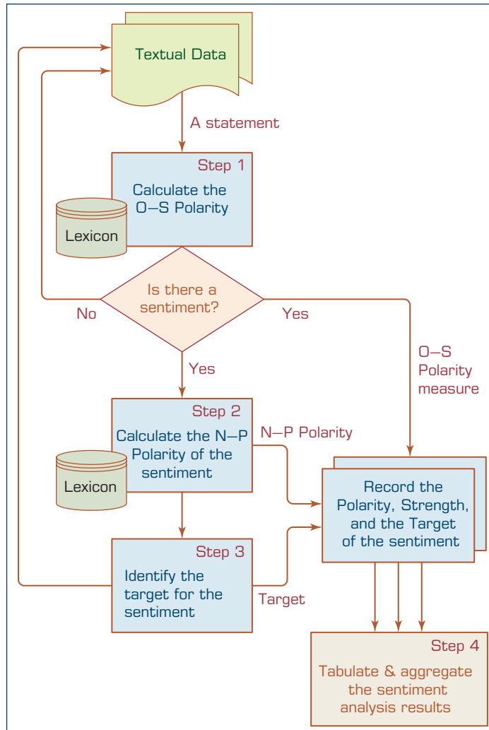
FIGURE 5.9 A Multistep Process to Sentiment Analysis.
