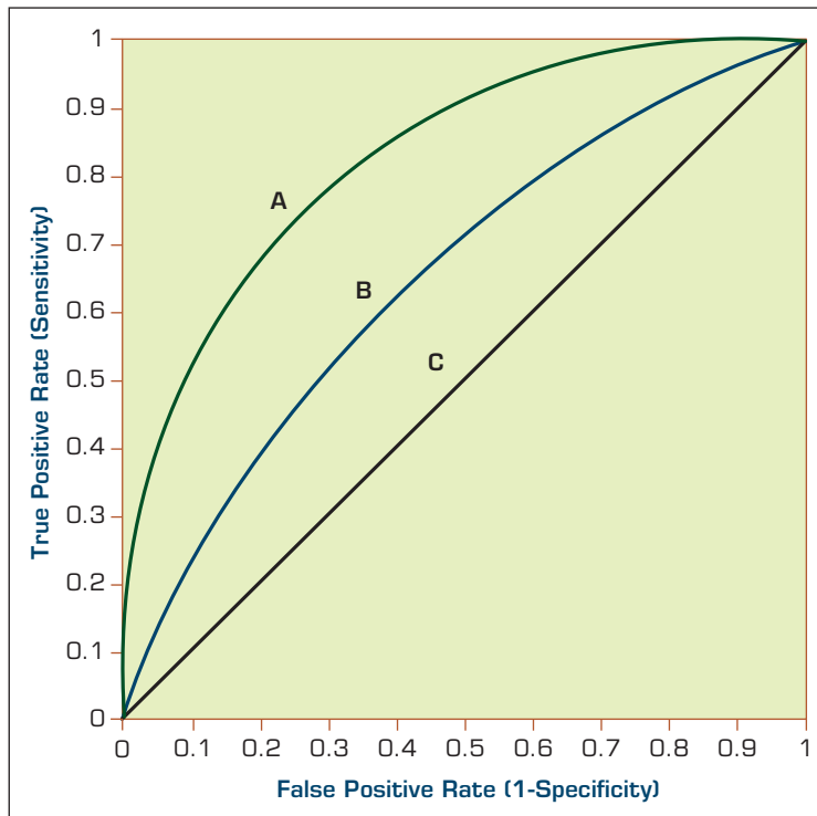
FIGURE 4.11 A Sample ROC Curve.
