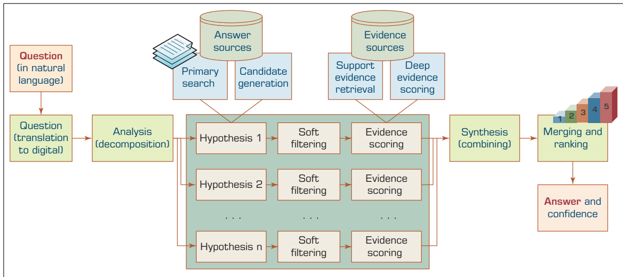
FIGURE 5.1 A High-Level Depiction of DeepQA Architecture.
