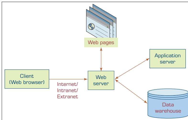
FIGURE 3.7 Architecture of Web-Based Data Warehousing.
