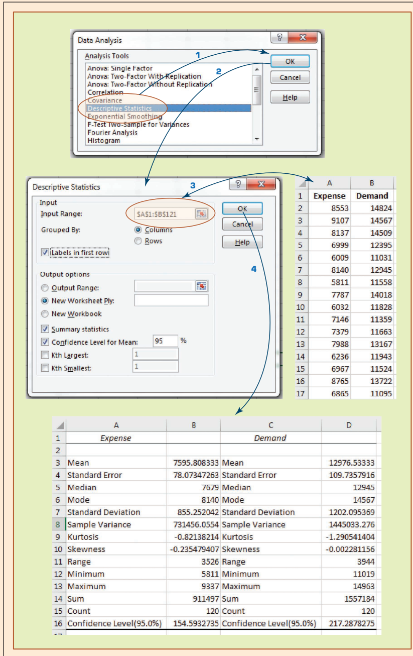
FIGURE 2.11 Obtaining Descriptive Statistics in Excel.
