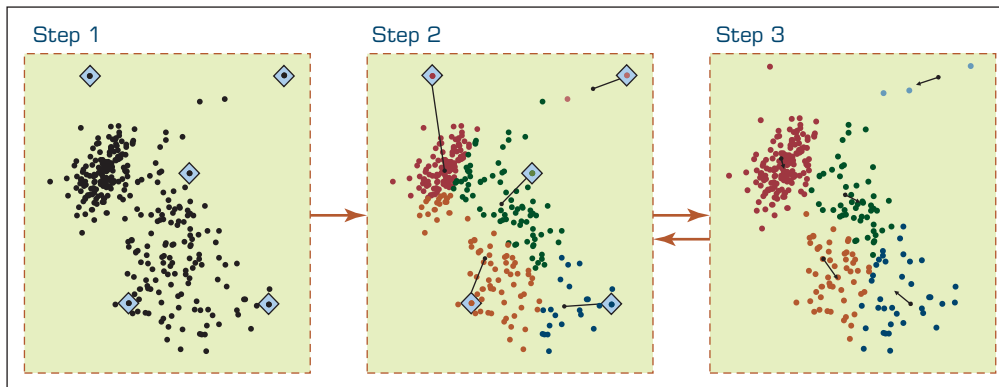
FIGURE 4.13 A Graphical Illustration of the Steps in the k -Means Algorithm.
