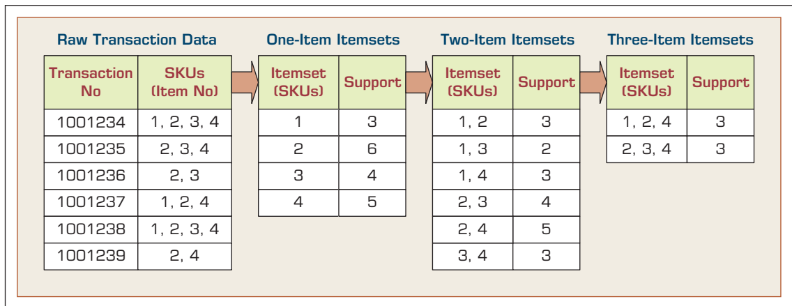
FIGURE 4.14 Identification of Frequent Itemsets in the Apriori Algorithm.
