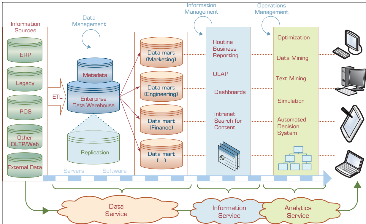
FIGURE 8.4 Conceptual Architecture of a Cloud-Oriented Support System. Source: Based on Demirkan, H., & Delen, D. (2013, April). Leveraging the capabilities of service-oriented decision support systems: Putting analytics and Big Data in cloud. Decision Support Systems , 55(1), 412–421.
