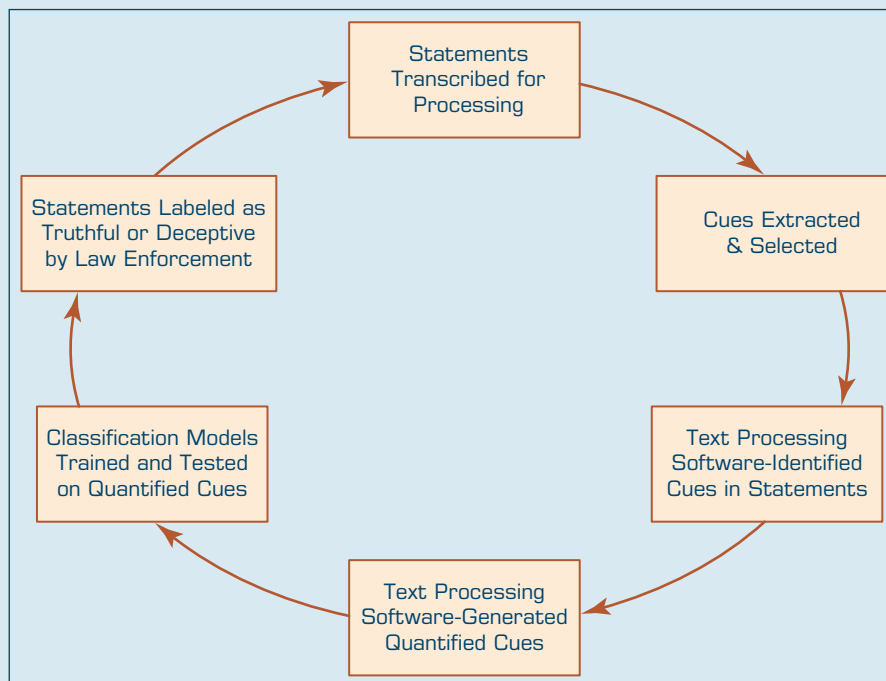
FIGURE 5.3 Text-Based Deception-Detection Process. Source: Fuller, C. M., Biros, D., & Delen, D. (2008, January). Exploration of feature selection and advanced classification models for high-stakes deception detection. Proceedings of the 41st Annual Hawaii International Conference on System Sciences (HICSS) , Big Island, HI: IEEE Press, 80–99.
