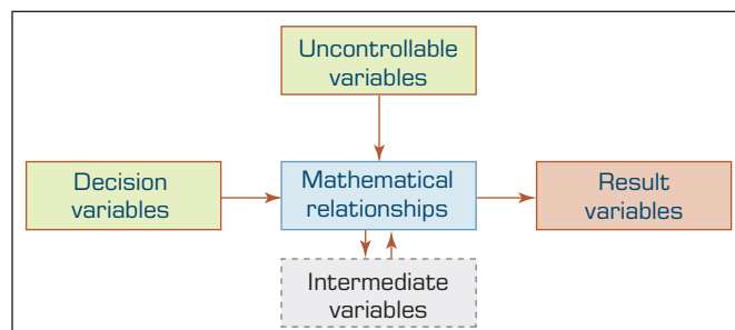
FIGURE 6.1 The General Structure of a Quantitative Model.
