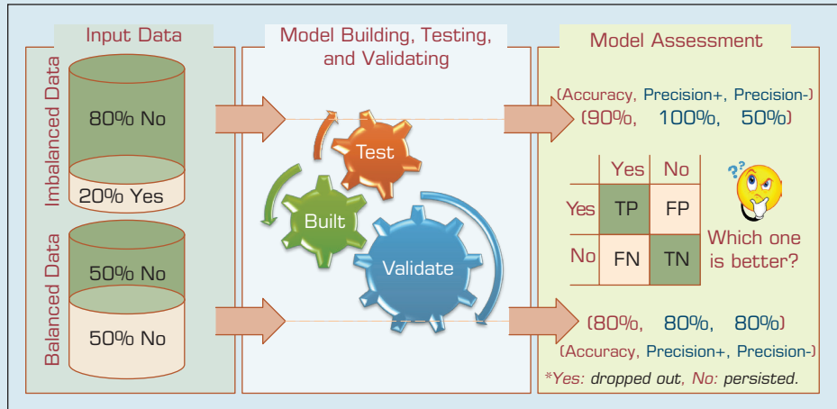
FIGURE 2.5 A Graphical Depiction of the Class Imbalance Problem.
