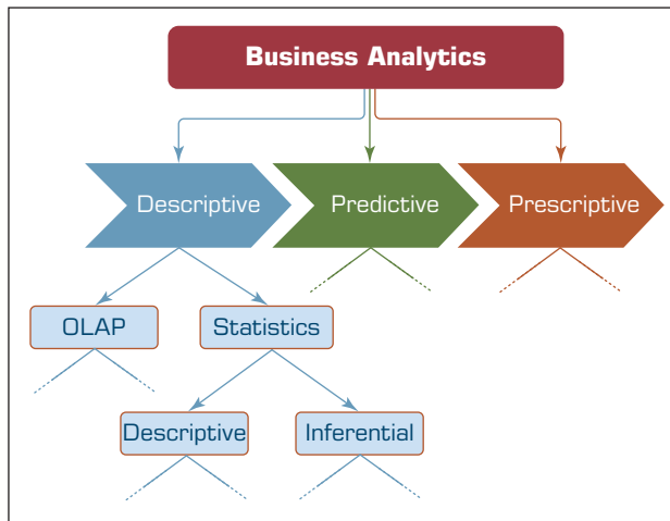
FIGURE 2.7 Relationship between Statistics and Descriptive Analytics.
