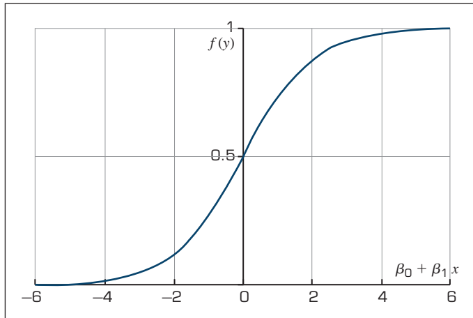
FIGURE 2.15 The Logistic Function.
