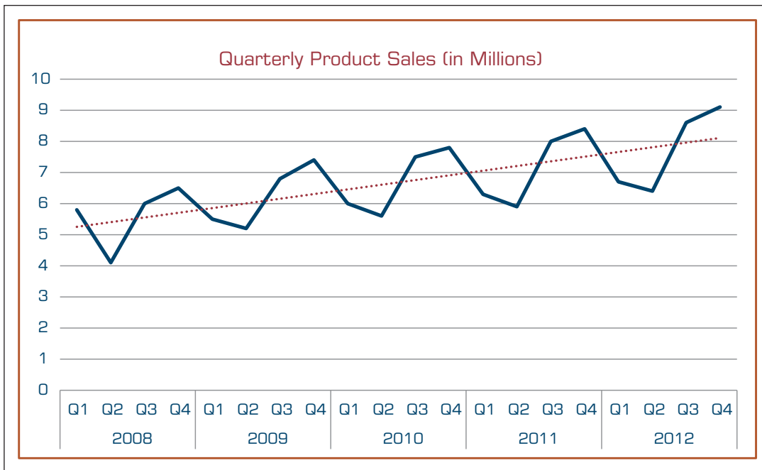
FIGURE 2.17 A Sample Time Series of Data on Quarterly Sales Volumes.
