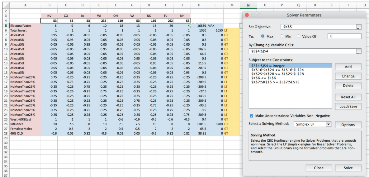
FIGURE 6.8 Model for Election Resource Allocation—Standard Version.
