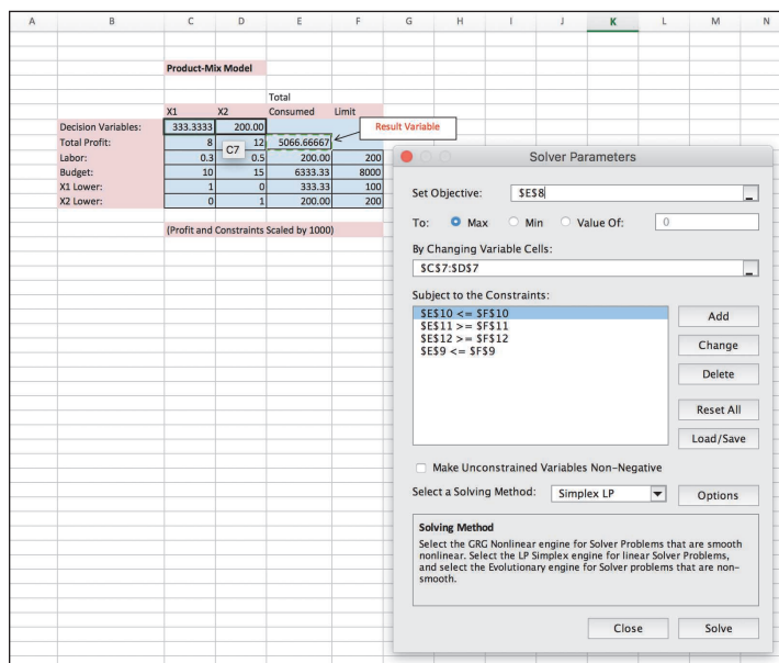
FIGURE 6.6 Excel Solver Solution to the Product-Mix Example.
