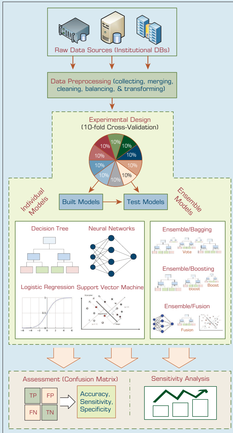
FIGURE 2.4 An Analytics Approach to Predicting Student Attrition.
