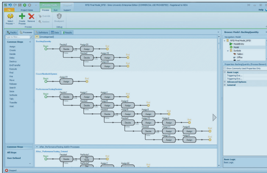
FIGURE 6.14 Process View of the Simulation Model.
