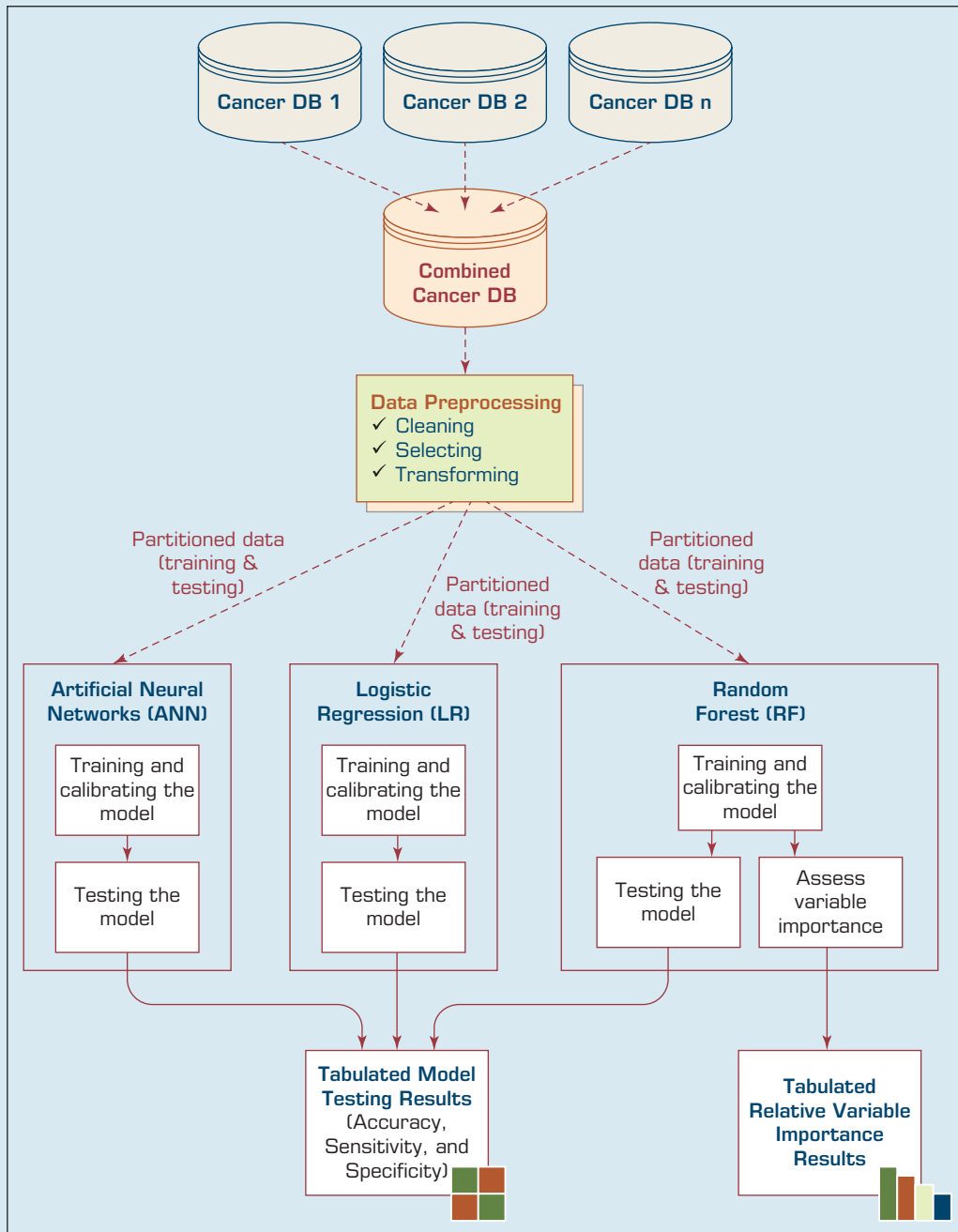
FIGURE 4.4 A Data Mining Methodology for Investigation of Comorbidity in Cancer Survivability.
