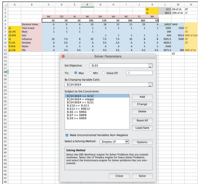
FIGURE 6.9 A Compact Formulation for Election Resource Allocation.
