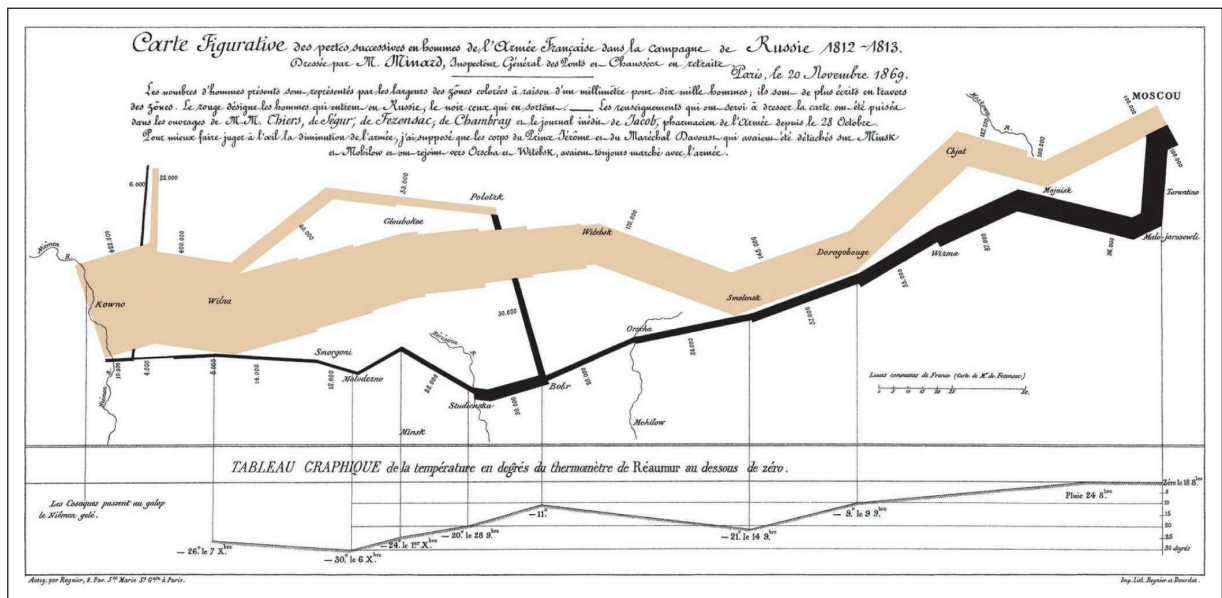
FIGURE 2.20 Decimation of Napoleon's Army during the 1812 Russian Campaign.
