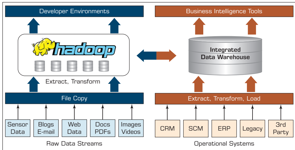
FIGURE 7.8 Coexistence of Hadoop and Data Warehouses. Source: Teradata Corp.
