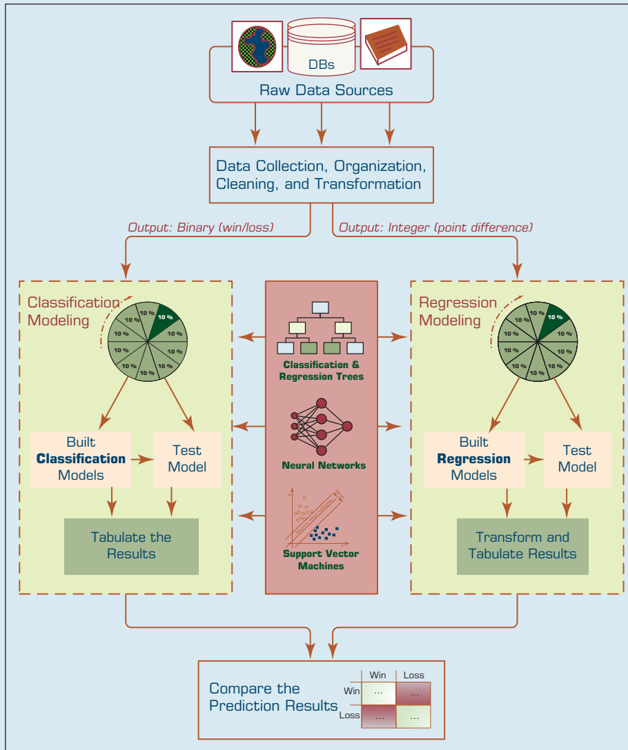
FIGURE 2.16 The Graphical Illustration of the Methodology Employed in the Study.
