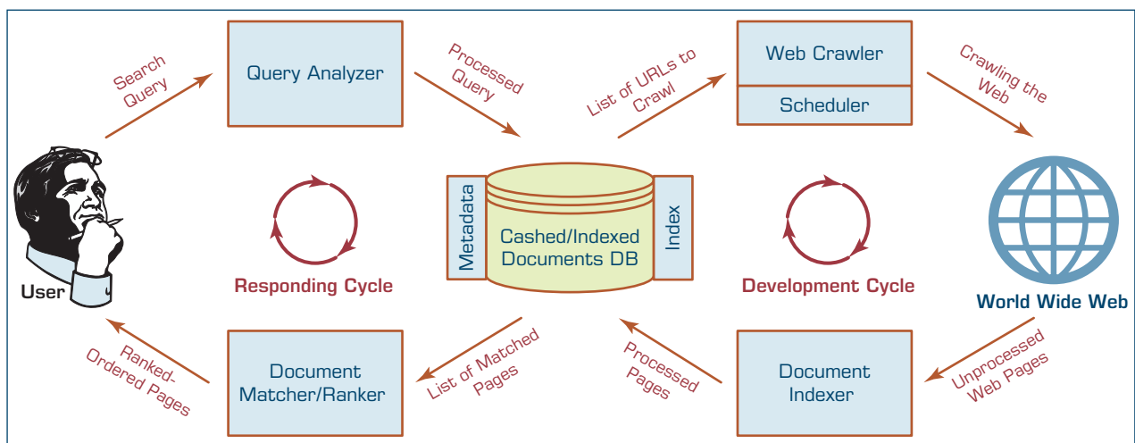
FIGURE 5.12 Structure of a Typical Internet Search Engine.
