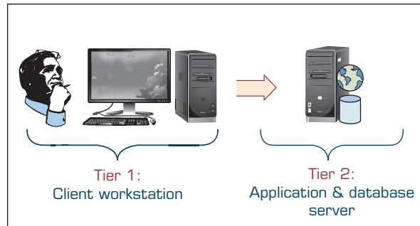
FIGURE 3.6 Architecture of a Two-Tier Data Warehouse.
