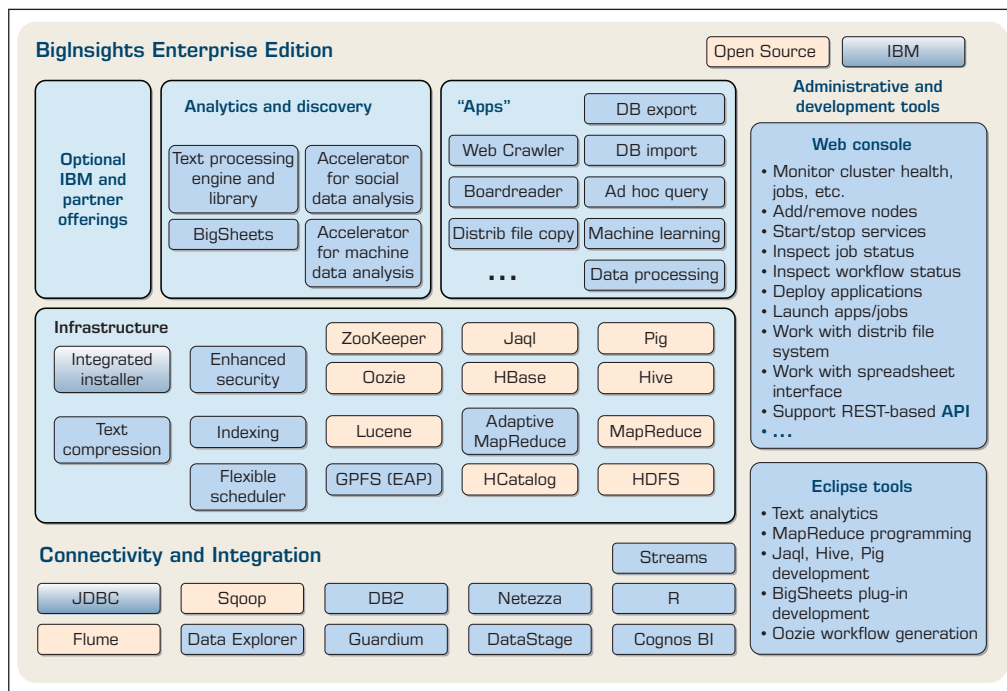
FIGURE 7.9 IBM InfoSphere Architecture.
