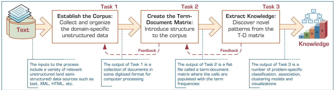
FIGURE 5.6 The Three-Step/Task Text Mining Process.
