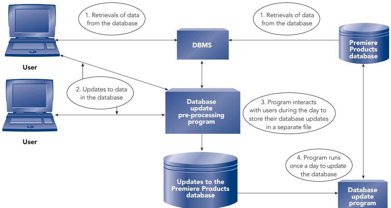
FIGURE 7-7 Delaying updates to the Premiere Products database to avoid the lost update problem
