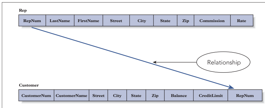
FIGURE 1-4 One-to-many relationship
