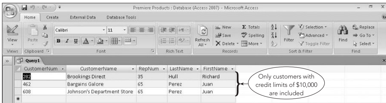
FIGURE 2-32 Query results
