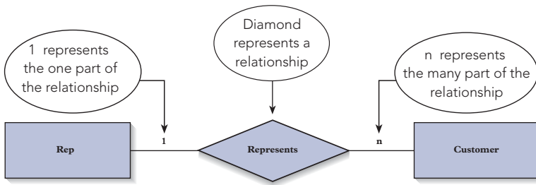
FIGURE 6-34 One-to-many relationship
