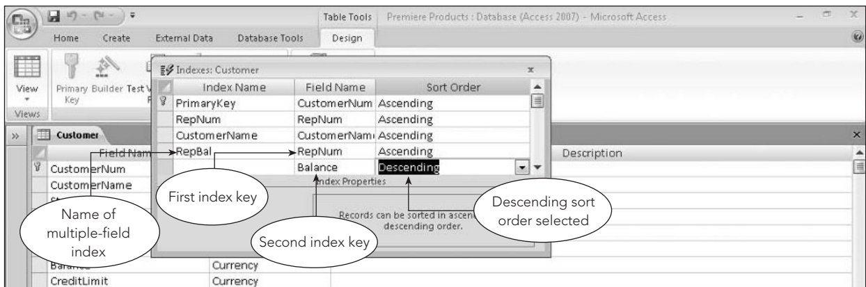
FIGURE 4-14 Creating a multiple-field index in Access
