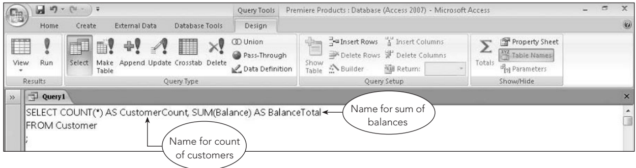
FIGURE 3-38 SQL query to perform calculations and rename columns
