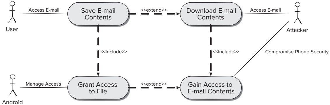
FIGURE 18.3 Misuse case (exploited by DroidCleaner): Data in an e-mail stored on the smartphone is stolen
