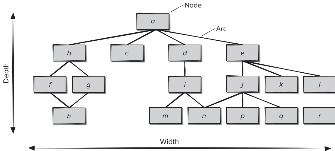
FIGURE 23.1 Morphology metrics
