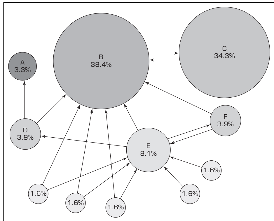
FIGURE 8.3 A Graphical Example for the PageRank Algorithm.
