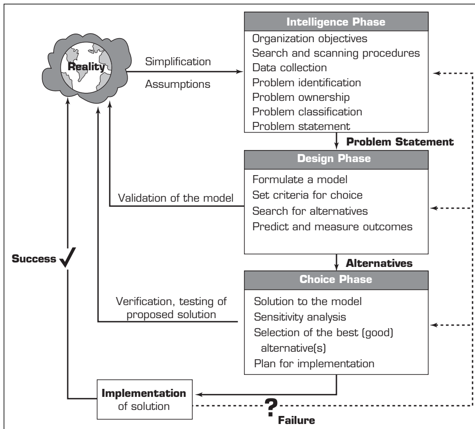
FIGURE 2.1 The Decision-Making/Modeling Process.
