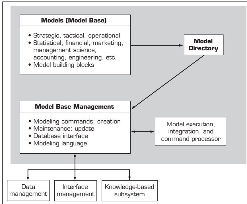
FIGURE 2.6 Structure of the Model Management Subsystem.
