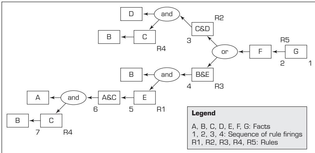
FIGURE 11.6 A Graphical Depiction of Backward Chaining.
