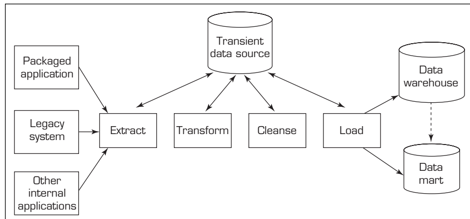
FIGURE 3.9 The ETL Process.
