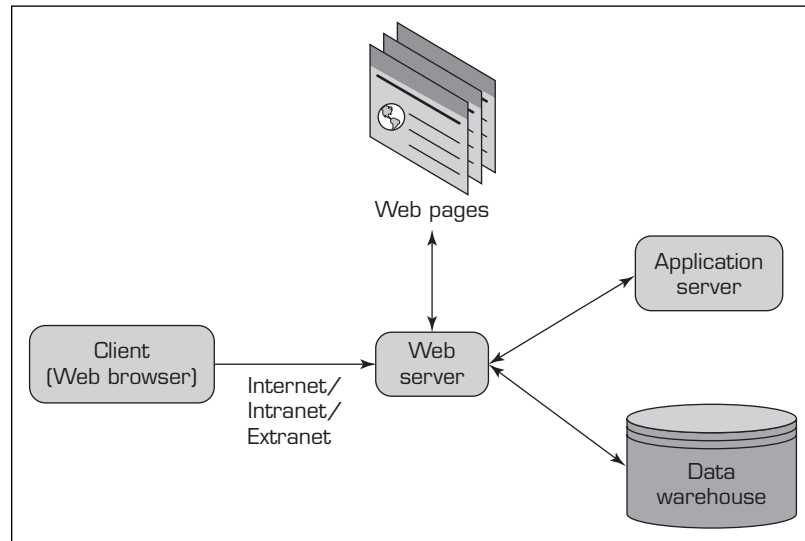
FIGURE 3.6 Architecture of Web-Based Data Warehousing.
