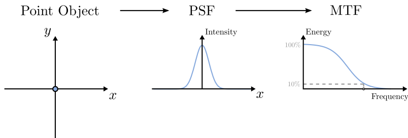
Figure 8.21: If we could scan an ideal point object, the resulting reconstructed image would be the PSF of the system. The Fourier transform of the PSF is the MTF, which shows the relative contrasts achievable for varying object frequencies. In practice, this measurement is typically performed using thin wire phantoms.
