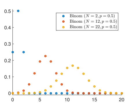
(b) Mass distribution functions of binomial distributions with varying number of trials N and fixed probability p = 0.5 .
