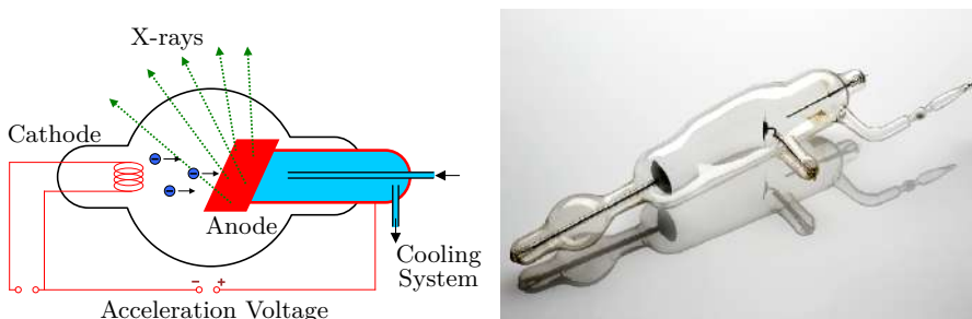
Figure 7.7: Vacuum X-ray tube: The image on the left shows a schematic how electrons are accelerated from the cathode to the anode to generate X-ray photons. The image on the right shows a historic vacuum X-ray tube. Image provided by Science Museum, London, Wellcome Images under Creative Commons by-nc-nd 2.0 UK .
