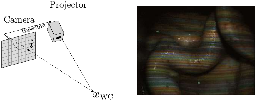
Figure 4.5: The illustration on the left hand side describes a structured light setup with one camera and one projector that generates a known pattern onto the scene. The projection of this point onto the image plane results in a pixel index i . Together with the projection pattern the 3-D world \mathbf{x}_{WC} can be reconstructed using triangulation. The right hand side image shows a projection on animal organs.
