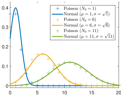
(a) Mass distribution functions of Poisson distributions with varying expectation value N_0 , plus their Gaussian counterparts.
