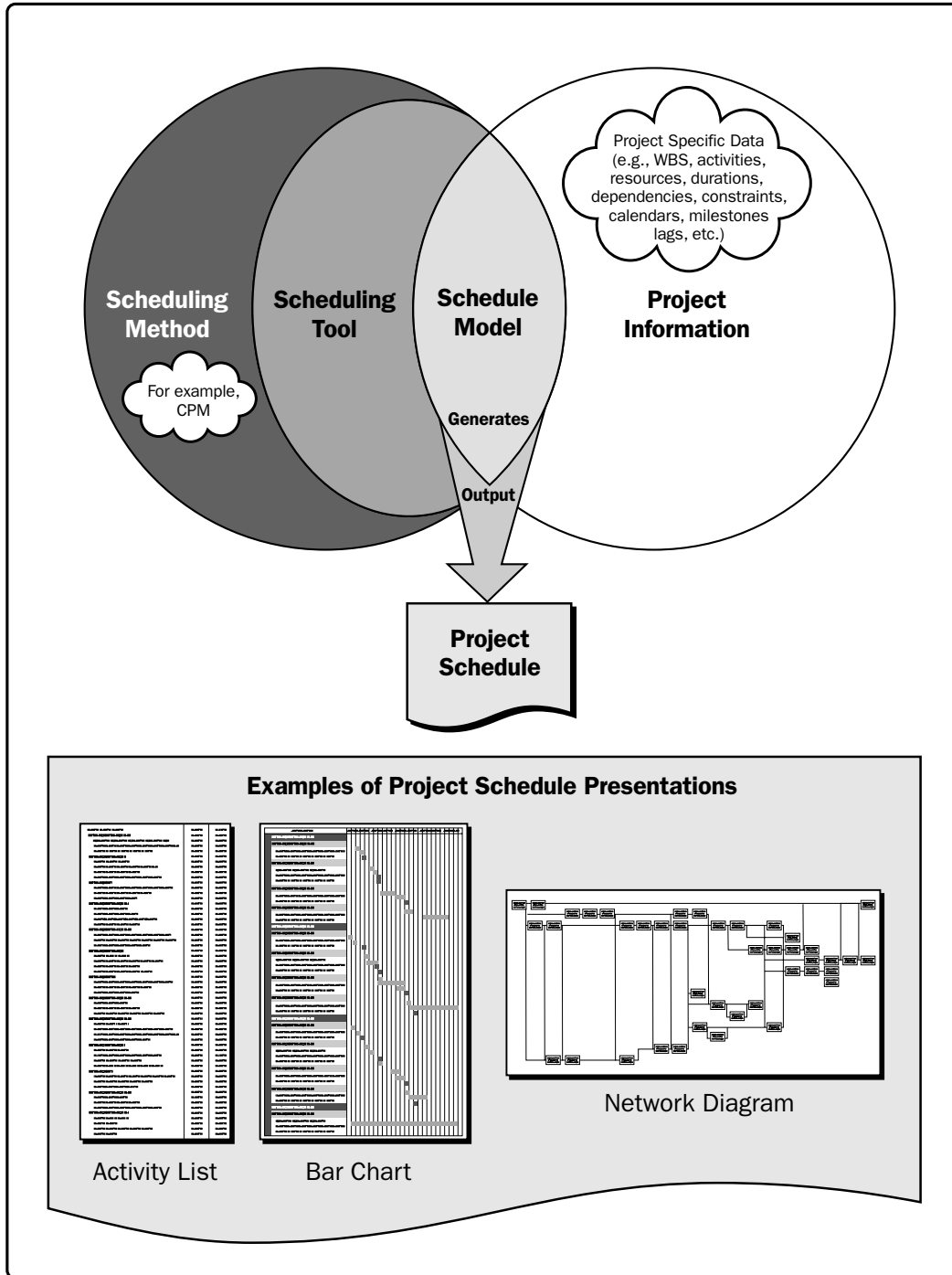
Figure 6-2. Scheduling Overview
