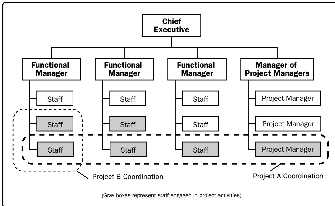
Figure 2-6. Composite Organization
