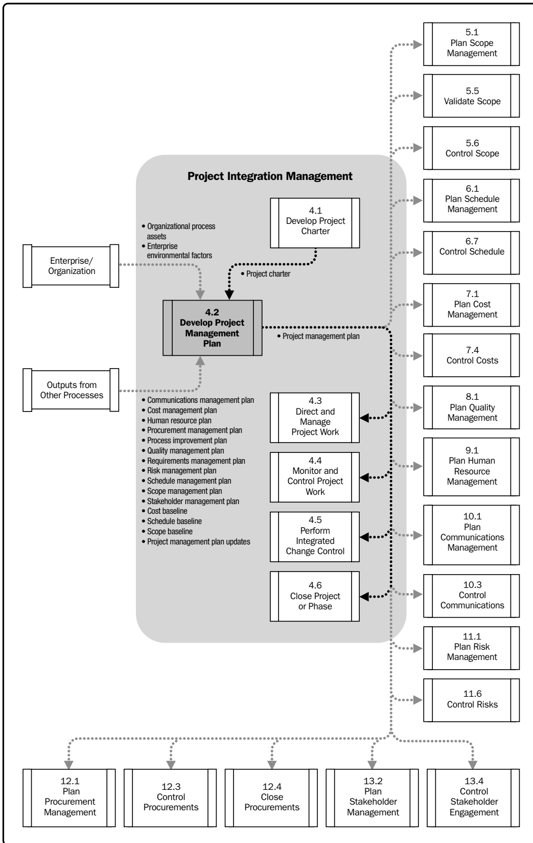
Figure 4-5. Develop Project Management Plan Data Flow Diagram
