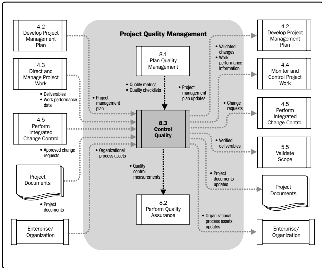
Figure 8-12. Control Quality Data Flow Diagram
