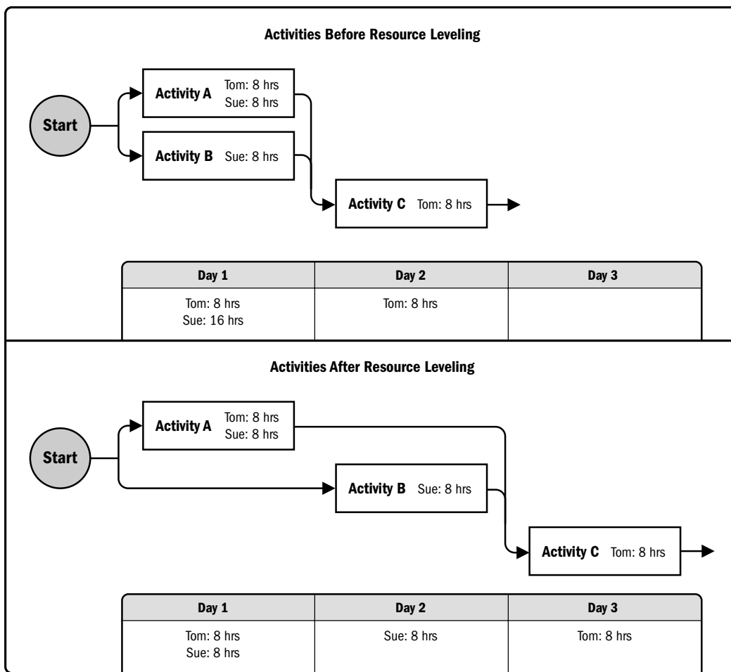
Figure 6-20. Resource Leveling
