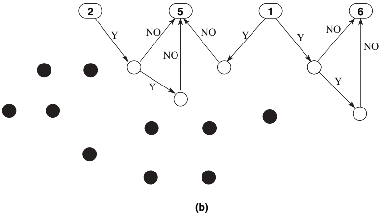
FIGURE 3.57: The effects of pruning in the first iteration: Some nodes (in black) and links are removed from consideration.
