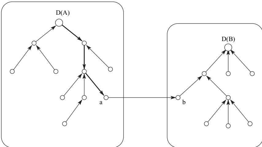
FIGURE 3.50: Absorption. To make the districts of A be rooted in D(B) , the logical direction of the links (in bold) from the downtown to the exit point of A has been “flipped.”
