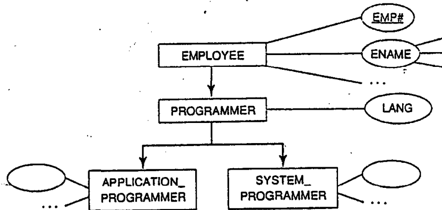
Fig. 14.3 Example of an entity type hierarchy
