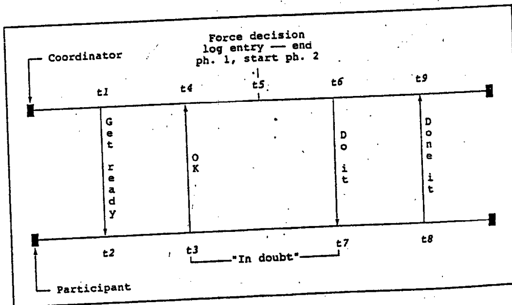
Fig. 21.5 Two-phase commit
