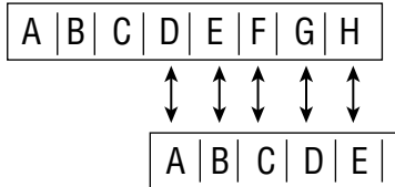
Figure 7-1 Caesar's cipher.
