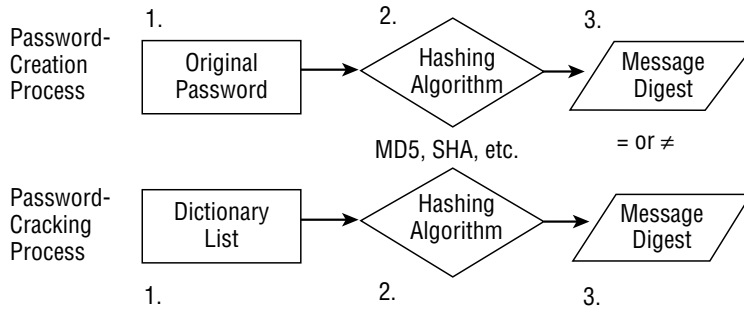
Figure 5-7 Password-cracking process.
