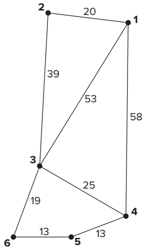
Figure 17.8 Link impedance values between cities on a road network.
