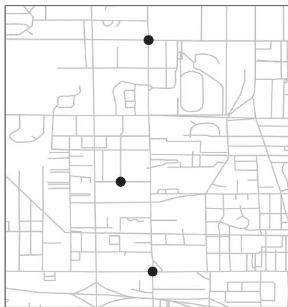
Figure 16.6 An example of intersection matching.
