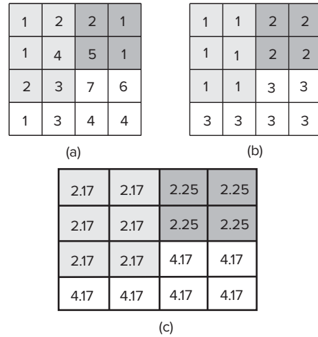
Figure 12.11 The cell values in (c) are the zonal means derived from an input raster (a) and a zonal raster (b). For example, 2.17 is the mean of [1, 1, 2, 2, 4, 3] for zone 1.
