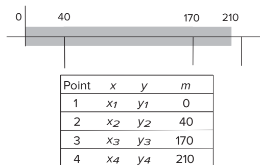
Figure 16.7 An example of a geodatabase route feature class.
