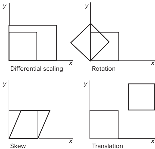
Figure 6.2 Differential scaling, rotation, skew, and translation in the affine transformation.
