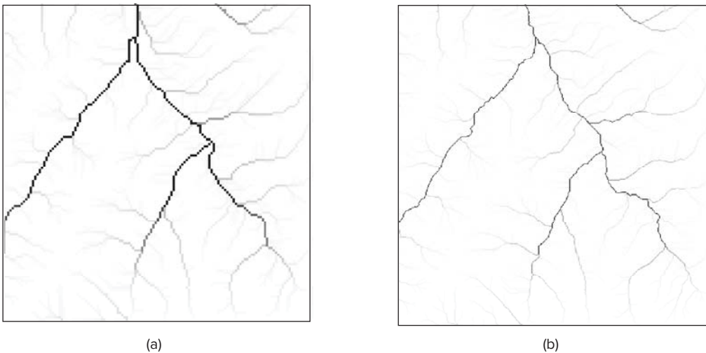
Figure 14.19 Stream networks derived from the DEMs in Figure 14.18. The stream network derived from the 30-meter DEM (a) has fewer details than that from the 10-meter DEM (b).
