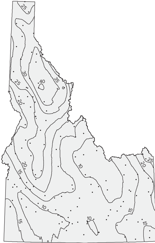
Figure 15.22 An isohyet map created by universal kriging with the linear drift and the spherical model.
