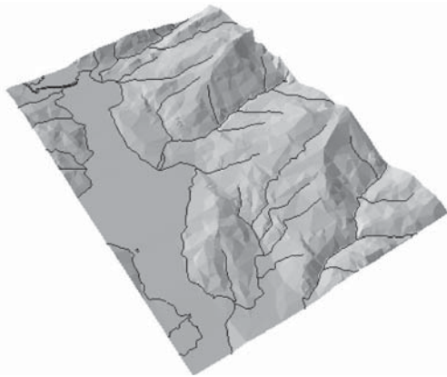
Figure 13.9 Draping of streams and shorelines on a 3-D surface.
