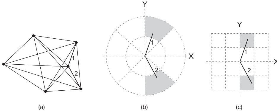
Figure 15.15 A common method for binning pairs of sample points by direction, such as 1 and 2 in (a), is to use the radial sector (b). Geostatistical Analyst in ArcGIS uses grid cells instead (c).
