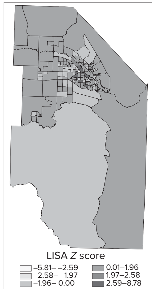
Figure 11.20 Z scores for the Local Indicators of Spatial Association (LISA) by block group in Ada County, Idaho.
