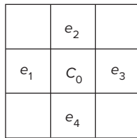
Figure 13.16 Ritter’s algorithm for computing slope and aspect at C_0 uses the four immediate neighbors of C_0 .
