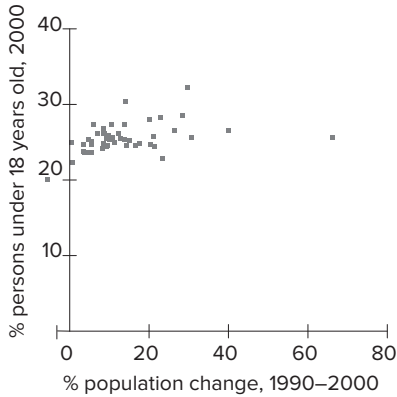
Figure 10.4 A scatterplot plotting percent persons under 18 years old in 2000 against percent population change, 1990–2000. A weak positive relationship is present between the two variables.
