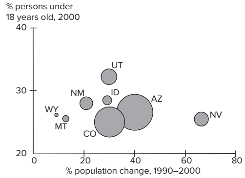
Figure 10.5 A bubble plot showing percent population change 1990–2000, percent persons under 18 years old in 2000, and state population in 2000.
