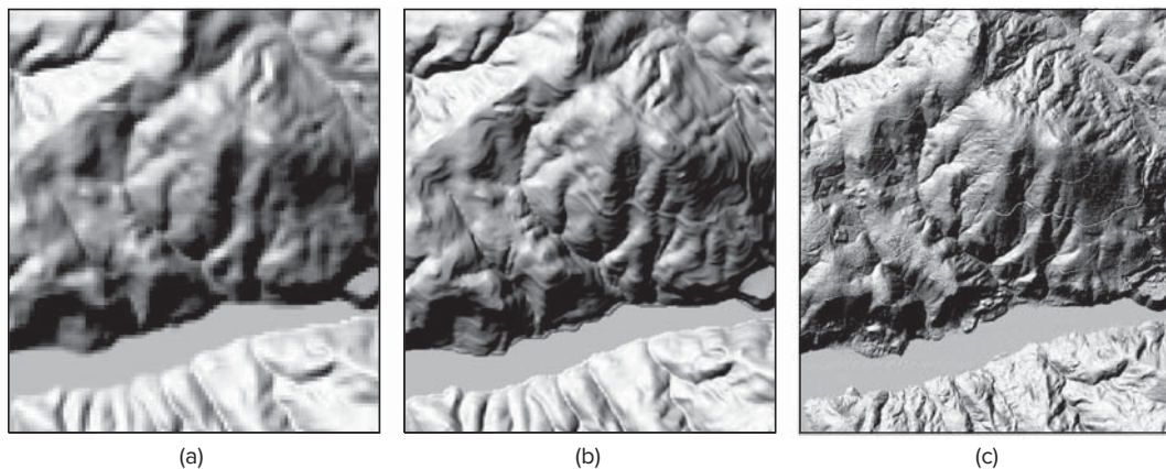
Figure 13.19 DEMs at three different resolutions: USGS 30-meter DEM (a), USGS 10-meter DEM (b), and 1.83-meter DEM derived from LiDAR data (c).
