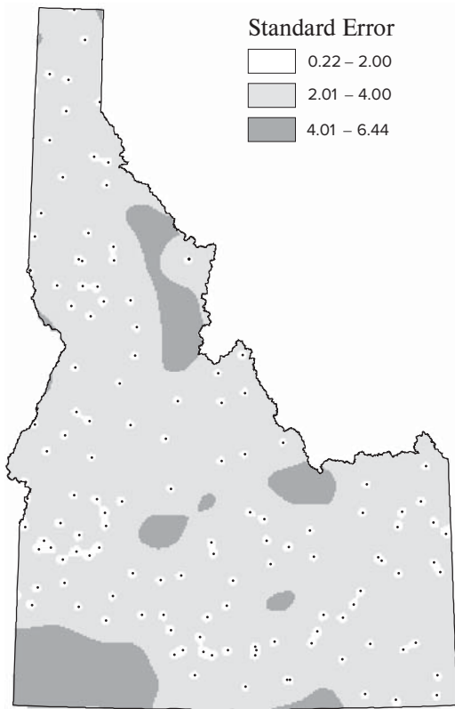
Figure 15.21 Standard errors of the annual precipitation surface in Figure 15.20.
