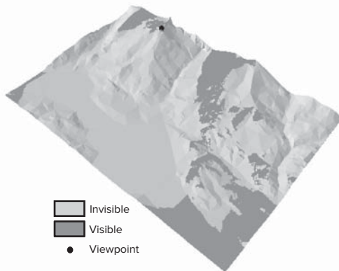
Figure 14.1 A viewshed example.
