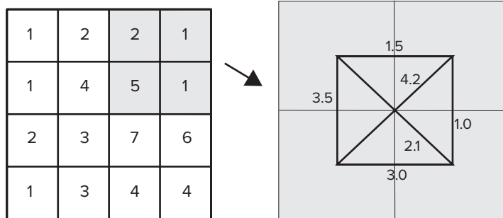
Figure 17.2 The cost distance of a lateral link is the average of the costs in the linked cells, for example, (1 + 2)/2 = 1.5 . The cost distance of a diagonal link is the average cost times 1.414, for example, 1.414 \times [(1 + 5)/2] = 4.2 .
