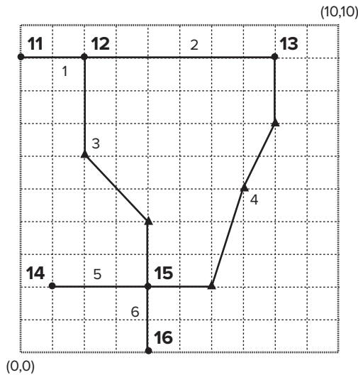
Figure 3.10 The data structure of a line coverage.
