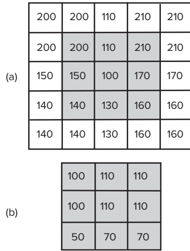
Figure 12.8 The cell values in (b) are the neighborhood range statistics of the shaded cells in (a) using a 3-by-3 neighborhood. For example, the upper-left cell in the output raster has a cell value of 100, which is calculated from (200 - 100) .
