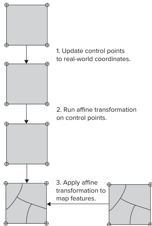
Figure 6.3 A geometric transformation typically involves three steps. Step 1 updates the control points to real-world coordinates. Step 2 uses the control points to run an affine transformation. Step 3 creates the output by applying the transformation equations to the input features.
