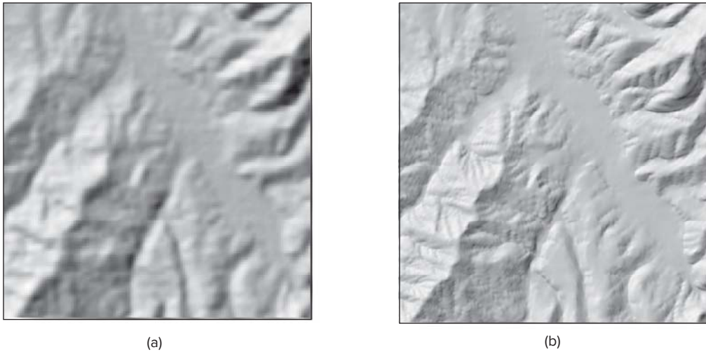
Figure 14.18 DEMs at a 30-meter resolution (a) and a 10-meter resolution (b).
