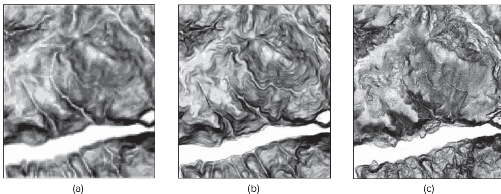
Figure 13.20 Slope layers derived from the three DEMs in Figure 13.19. The darkness of the symbol increases as the slope becomes steeper.
