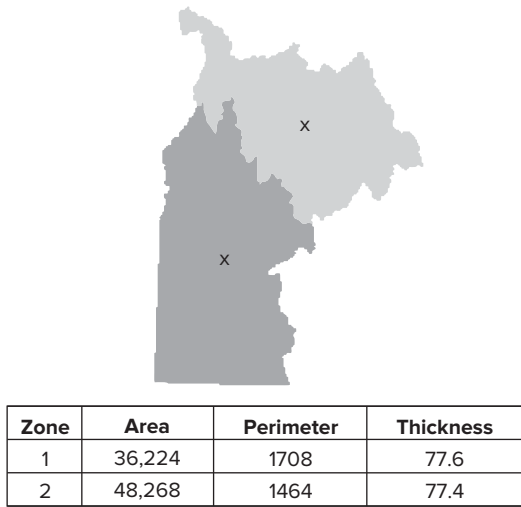
Figure 12.10 Thickness and centroid for two large watersheds (zones). Area is measured in square kilometers, and perimeter and thickness are measured in kilometers. The centroid of each zone is marked with an x.
