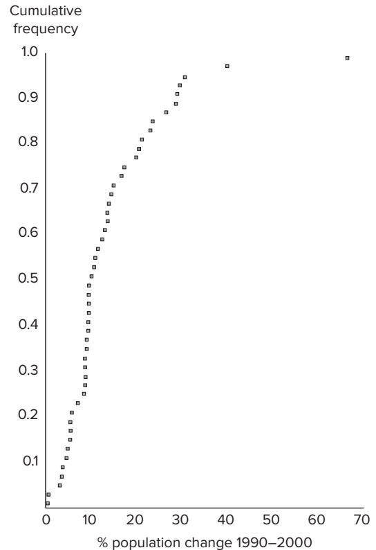
Figure 10.3 A cumulative distribution graph.
