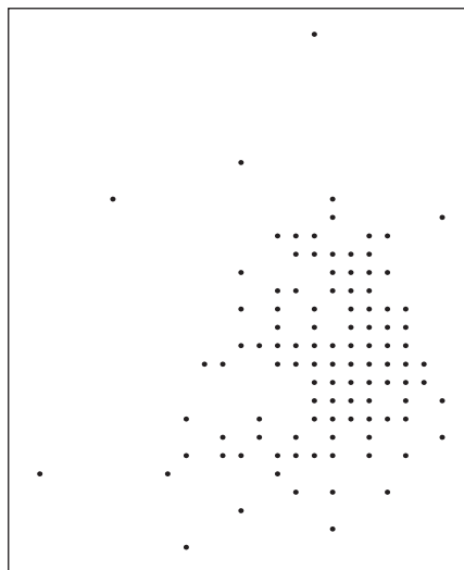
Figure 11.16 A point pattern showing deer locations.
