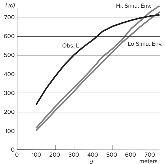
Figure 11.17 The computed L(d) and the lower and upper simulation envelopes.
