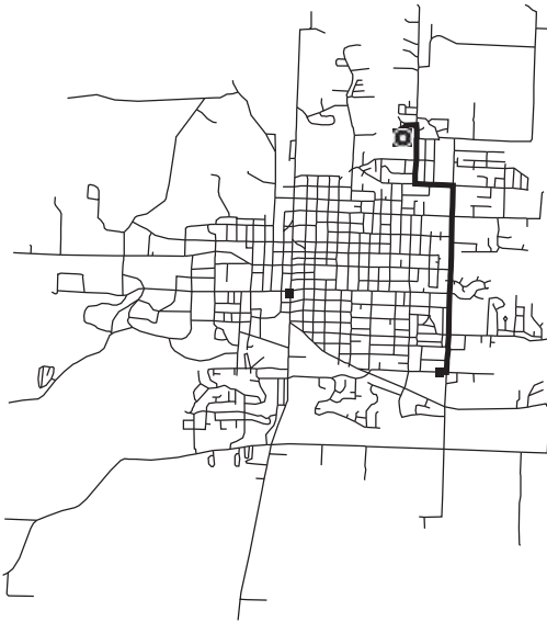
Figure 17.9 Shortest path from a street address to its closest fire station, shown by the square symbol.
