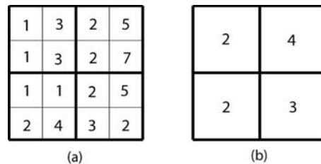
Figure 12.17 An Aggregate operation creates a lower-resolution raster (b) from the input (a). The operation uses the mean statistic and a factor of 2 (i.e., a cell in b covers 2-by-2 cells in a). For example, the cell value of 4 in (b) is the mean of {2, 2, 5, 7} in (a).
