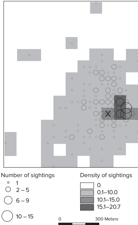
Figure 15.9 Deer sightings per hectare calculated by the kernel density estimation method. The letter X marks the cell, which is used as an example in Box 15.2.
