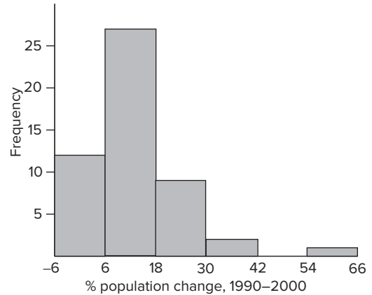
Figure 10.2 A histogram (bar chart).
