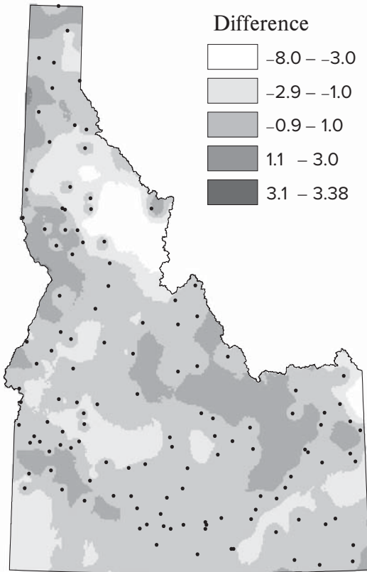
Figure 15.24 Differences between the interpolated surfaces from ordinary kriging and inverse distance squared.
