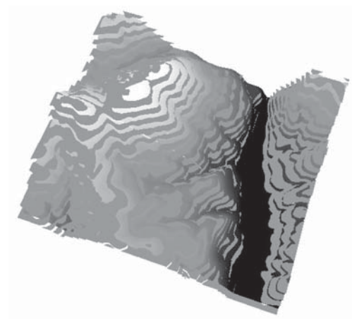
Figure 13.10 A 3-D perspective view of elevation zones.
