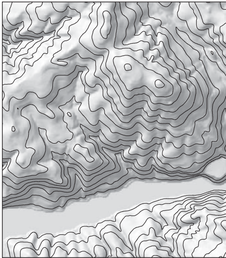
Figure 13.2 A contour line map.
