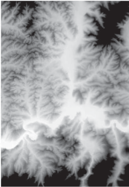
Figure 9.7 Map showing raster-based elevation data. Cells with higher elevations have darker shades.
