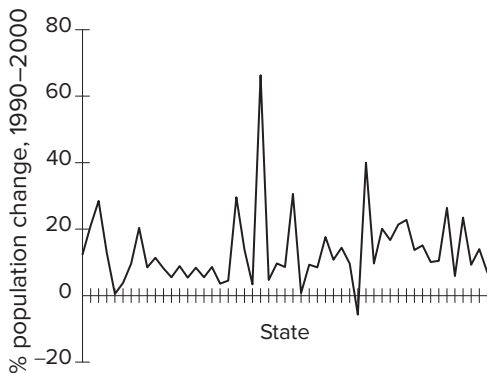
Figure 10.1 A line graph.
