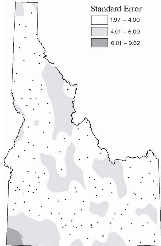
Figure 15.23 Standard errors of the annual precipitation surface in Figure 15.22.
