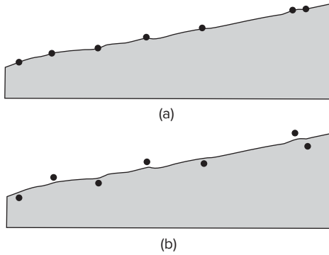
Figure 15.2 Exact interpolation (a) and inexact interpolation (b).
