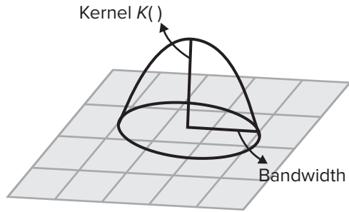
Figure 15.8 A kernel function, which represents a probability density function, looks like a “bump” above a grid.
