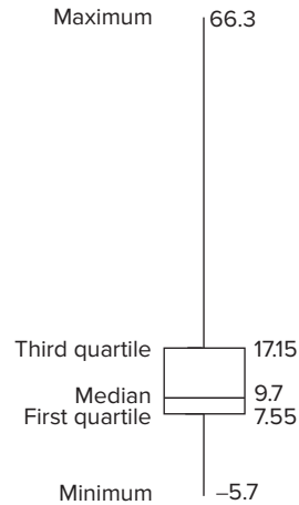
Figure 10.6 A boxplot showing the statistics of percent population change, 1990–2000.
