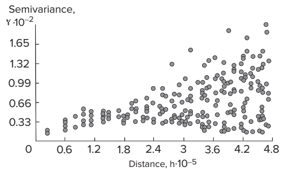
Figure 15.16 A semivariogram after binning by distance.
