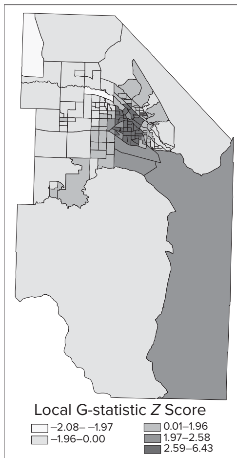
Figure 11.21 Z scores for the local G-statistics by block group in Ada County, Idaho.
