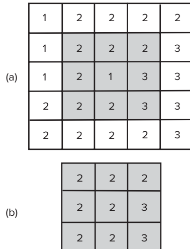
Figure 12.9 The cell values in (b) are the neighborhood majority statistics of the shaded cells in (a) using a 3-by-3 neighborhood. For example, the upper-left cell in the output raster has a cell value of 2 because there are five 2s and four 1s in its neighborhood.
