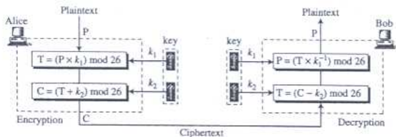
Figure 3.11 Affine cipher
