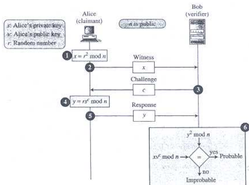
Figure 14.13 Fiat-Shamir protocol
