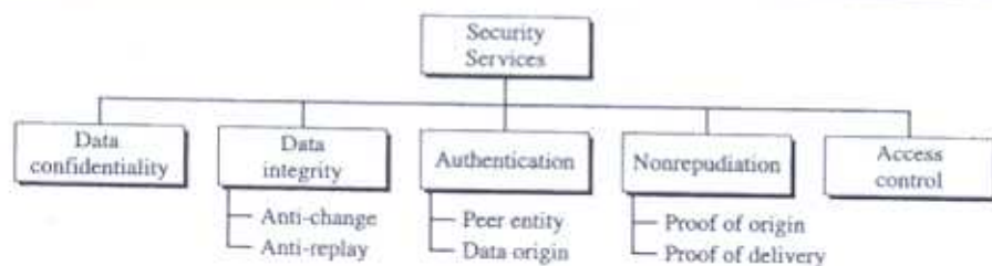
Figure 1.3 Security services
