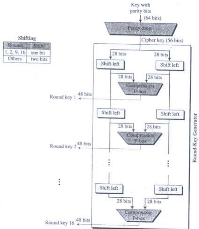
Figure 6.10 Key generation
