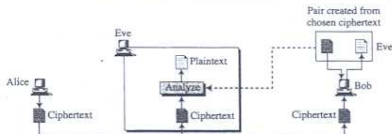
Figure 3.7 Chosen-ciphertext attack
