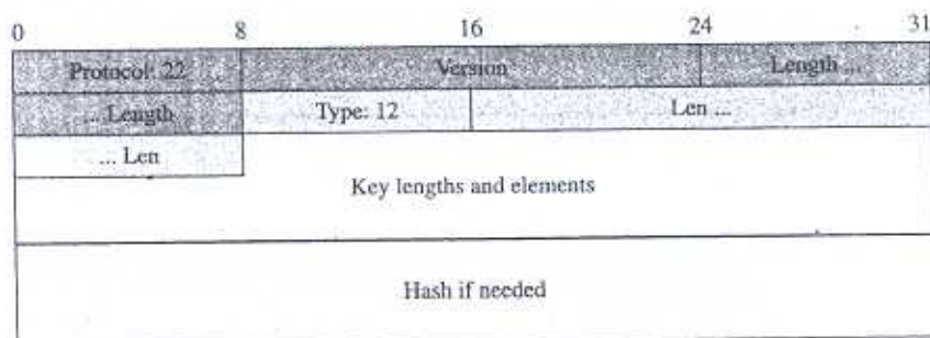
Figure 17.31 ServerKeyExchange message
