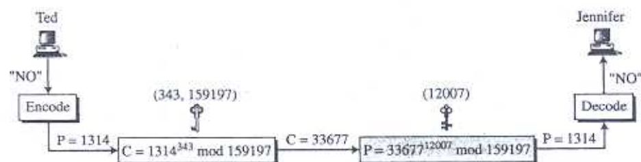
Figure 10.7 Encryption and decryption in Example 10.7
