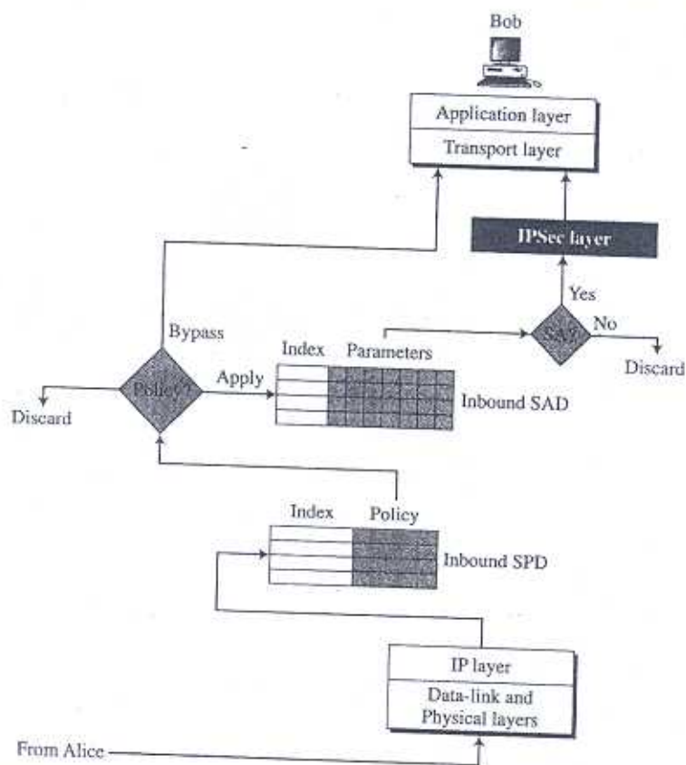
Figure 18.14 Inbound processing
