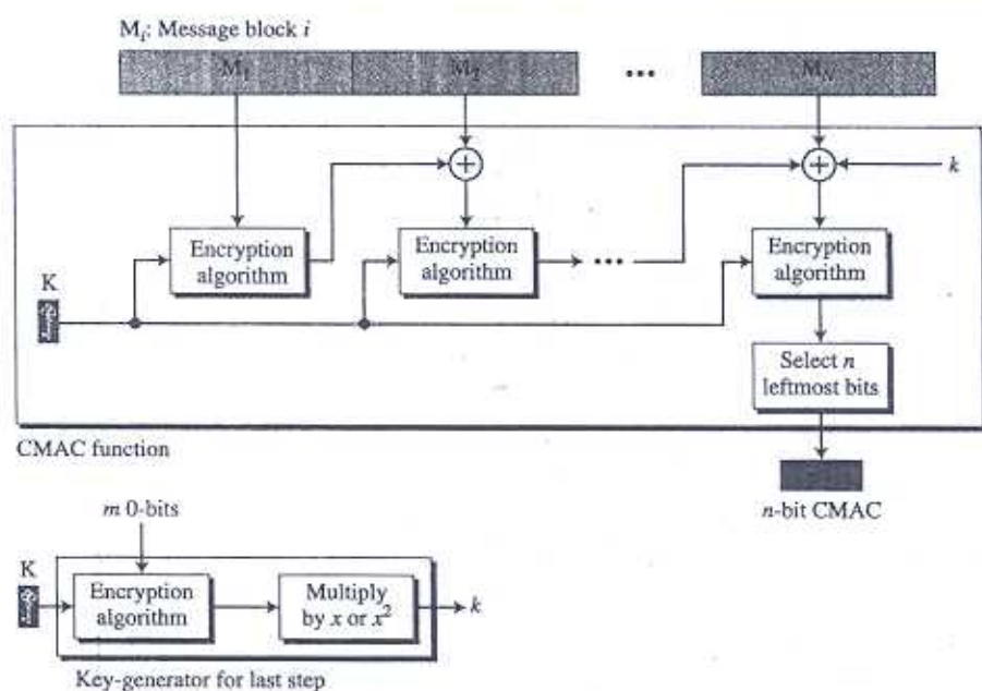
Figure 11.13 CMAC
