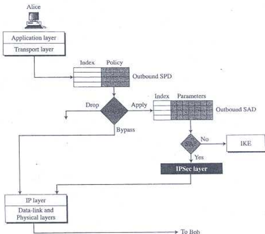
Figure 18.13 Outbound processing
