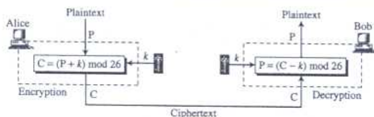
Figure 3.9 Additive cipher
