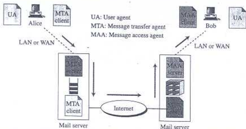
Figure 16.1 E-mail architecture
