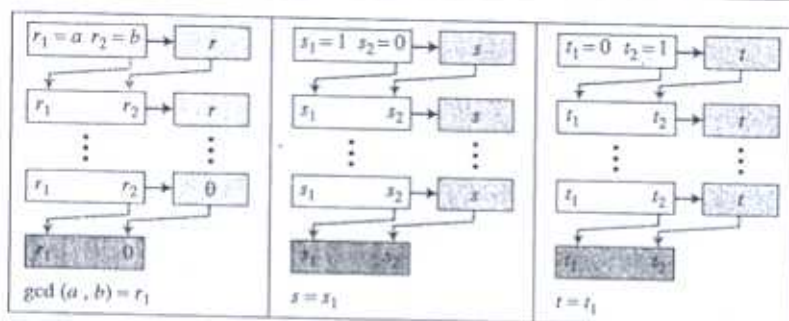
Figure 2.8 Extended Euclidean algorithm
