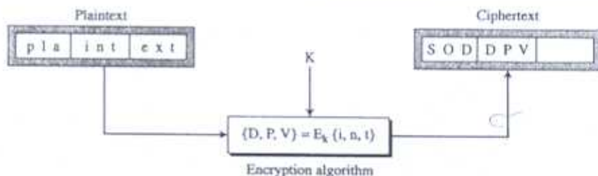
Figure 3.27 Block cipher
