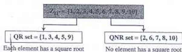
Figure 9.4 Division of Z_{11}^* elements into QRs and QNRs
