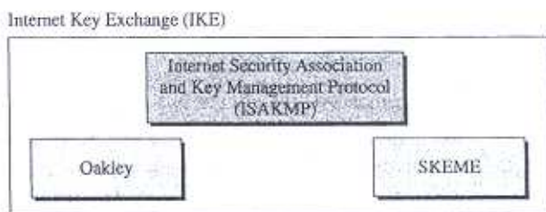
Figure 18.15 IKE components
