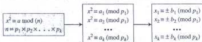
Figure 9.5 Decomposition of congruence modulo a composite
