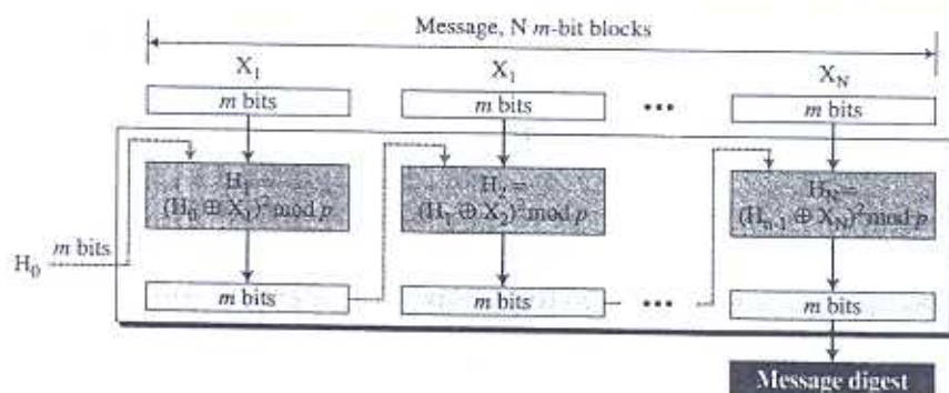
Figure 11.16 Exercise 26
