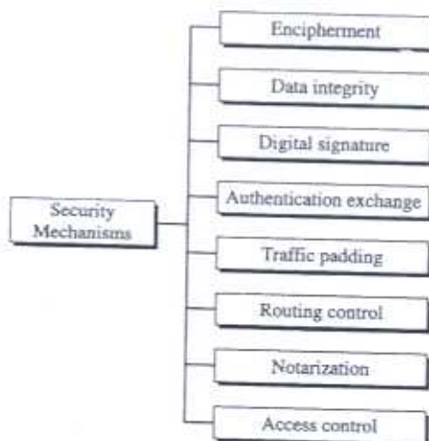
Figure 1.4 Security mechanisms
