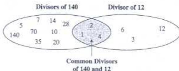
Figure 2.6 Common divisors of two integers
