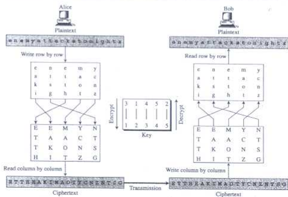
Figure 3.21 Example 3.27
