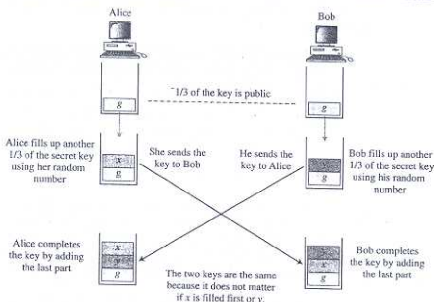
Figure 15.10 Diffie-Hellman idea
