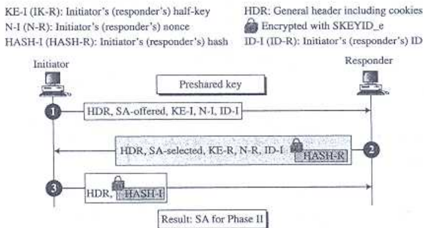
Figure 18.24 Aggressive mode, preshared-key method
