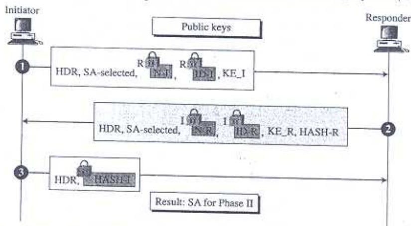
Figure 18.26 Aggressive mode, revised public-key method
