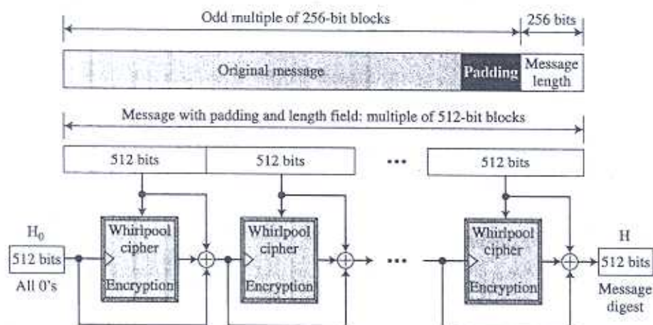
Figure 12.12 Whirlpool hash function
