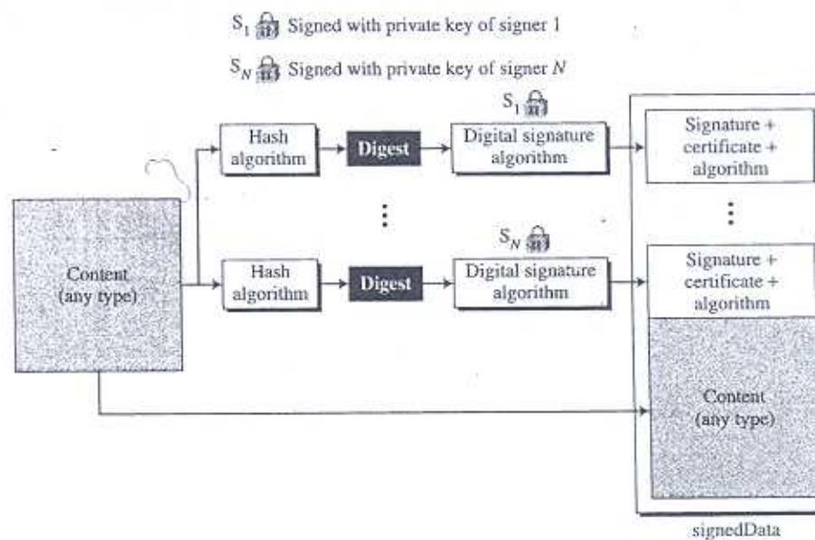
Figure 16.27 Signed-data content type
