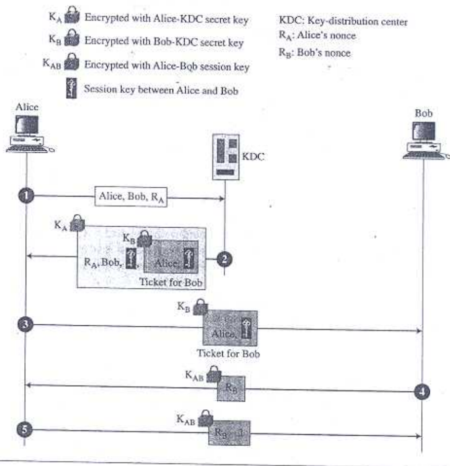
Figure 15.5 Needham-Schroeder protocol
