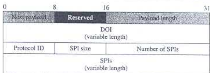
Figure 18.42 Delete payload
