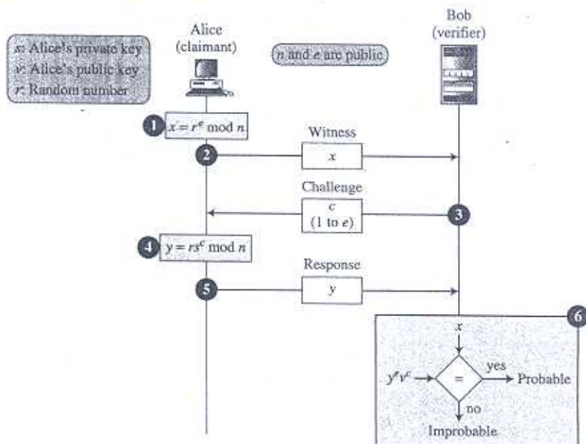
Figure 14.16 Guillou-Quisquater protocol
