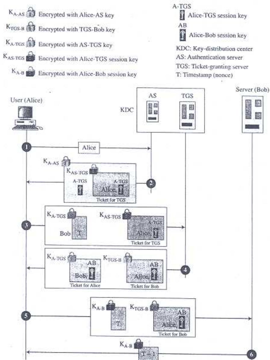
Figure 15.8 Kerberos example
