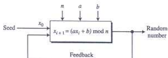
Figure K.2 Linear congruential pseudorandom number generator
