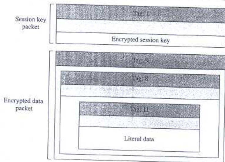
Figure 16.20 Encrypted message
