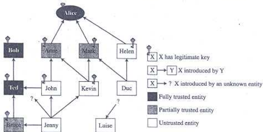
Figure 16.9 Trust model
