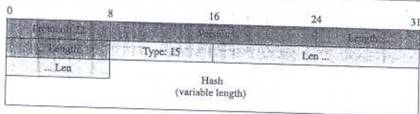
Figure 17.34 CertificateVerify message
