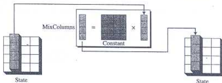
Figure 7.13 MixColumns transformation
