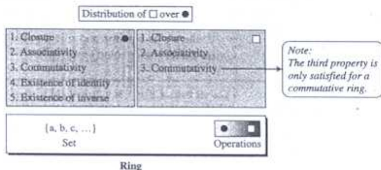
Figure 4.4 Ring
