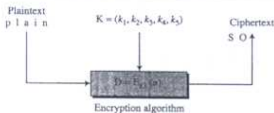
Figure 3.26 Stream cipher
