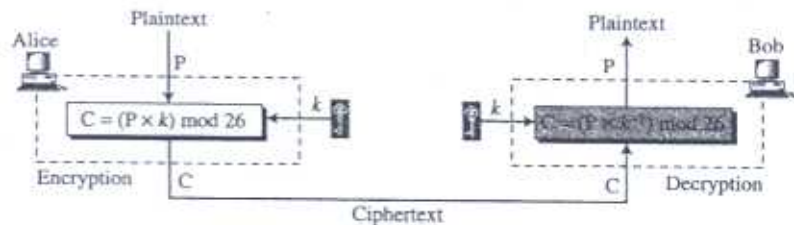
Figure 3.10 Multiplicative cipher
