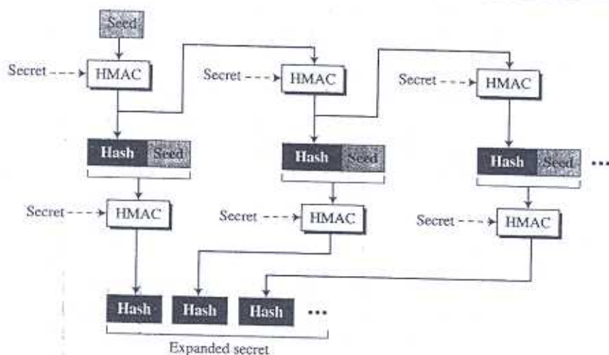
Figure 17.40 Data-expansion function
