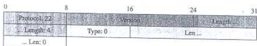
Figure 17.27 HelloRequest message
