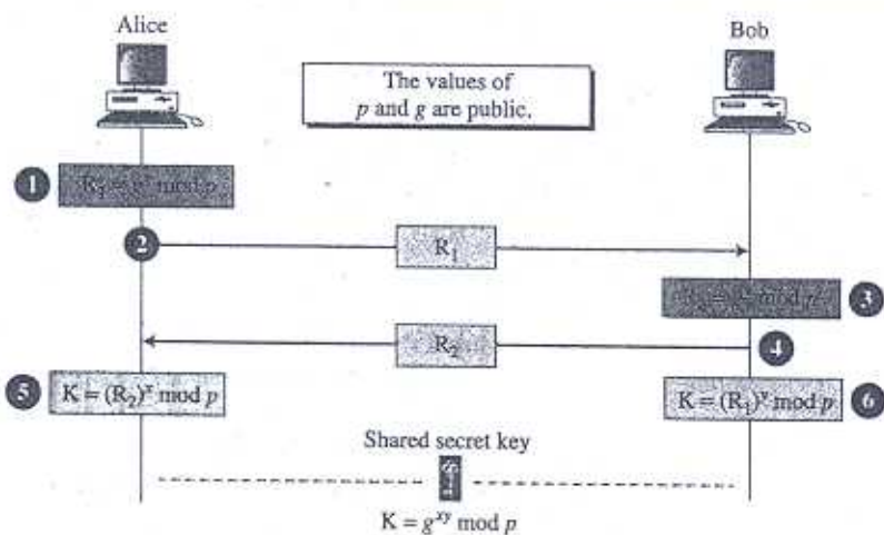
Figure 15.9 Diffie-Hellman method
