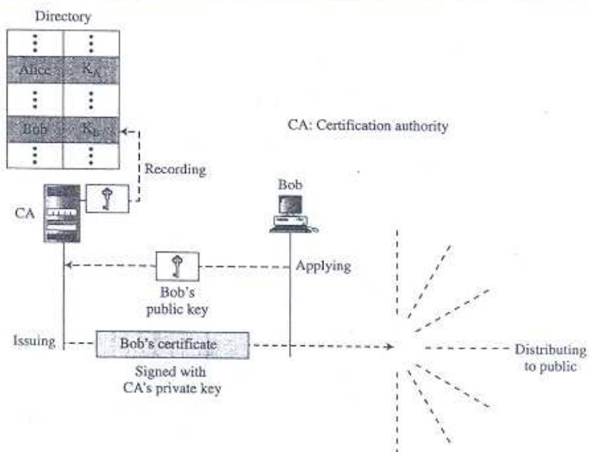
Figure 15.16 Certification authority
