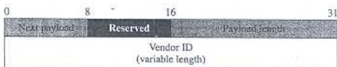
Figure 18.43 Vendor payload
