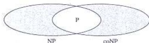
Figure L.1 Classes P, NP, and coNP
