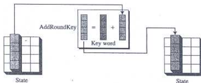
Figure 7.15 AddRoundKey transformation
