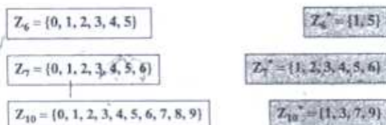
Figure 2.17 Some Z_n and Z_n^* sets
