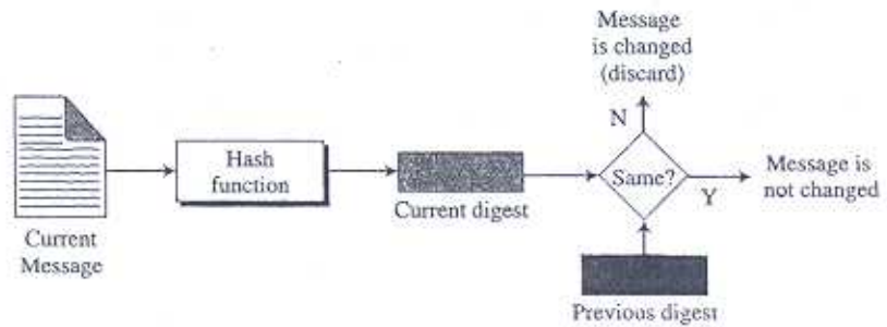
Figure 11.2 Checking integrity
