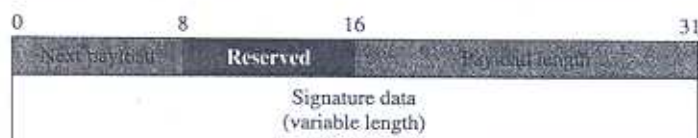
Figure 18.39 Signature payload
