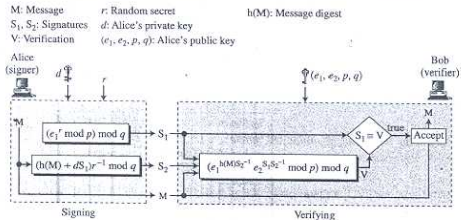
Figure 13.14 DSS scheme
