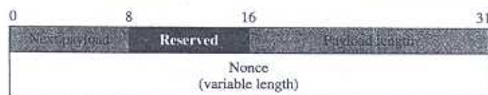
Figure 18.40 Nonce payload
