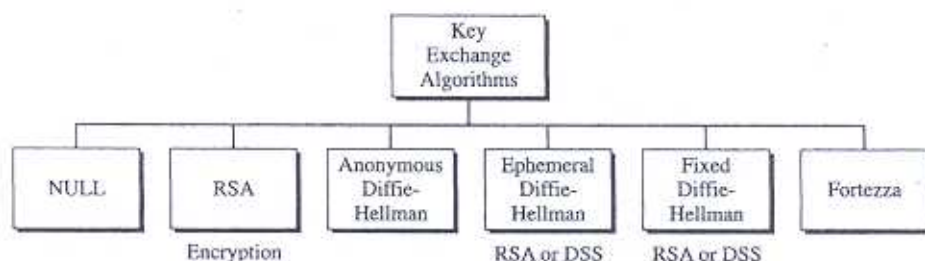
Figure 17.2 Key-exchange methods
