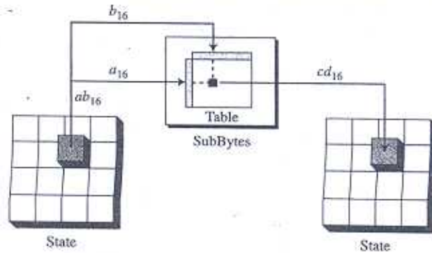
Figure 7.6 SubBytes transformations
