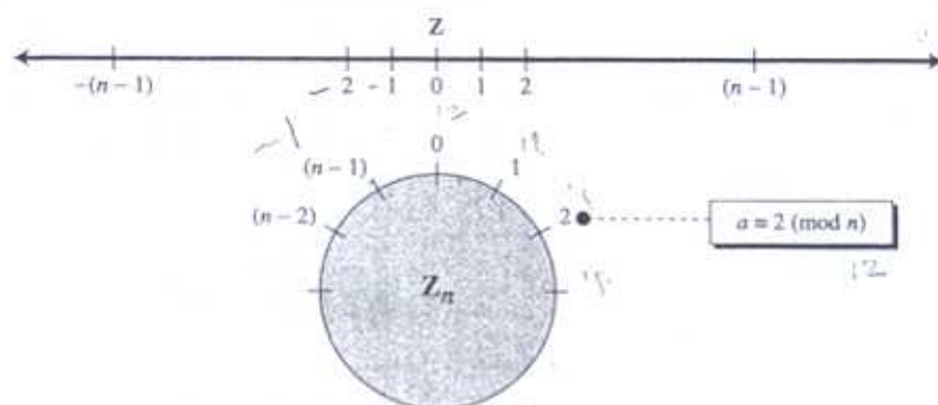
Figure 2.12 Comparison of Z and Z_n using graphs
