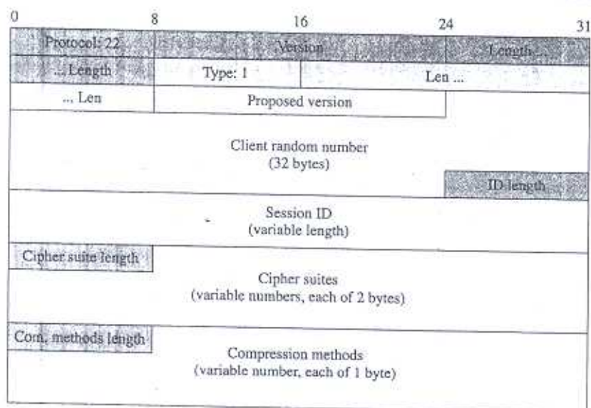
Figure 17.28 ClientHello message
