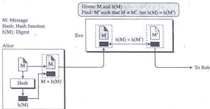
Figure 11.5 Second preimage
