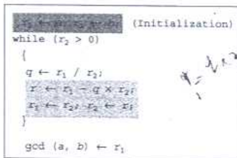
b. Algorithm
