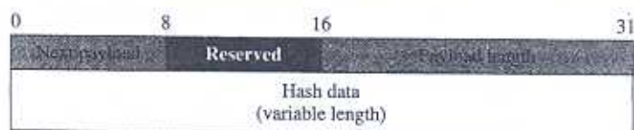
Figure 18.38 Hash payload
