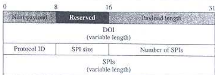
Figure 18.42 Delete payload
