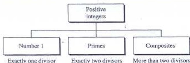
Figure 9.1 Three groups of positive integers
