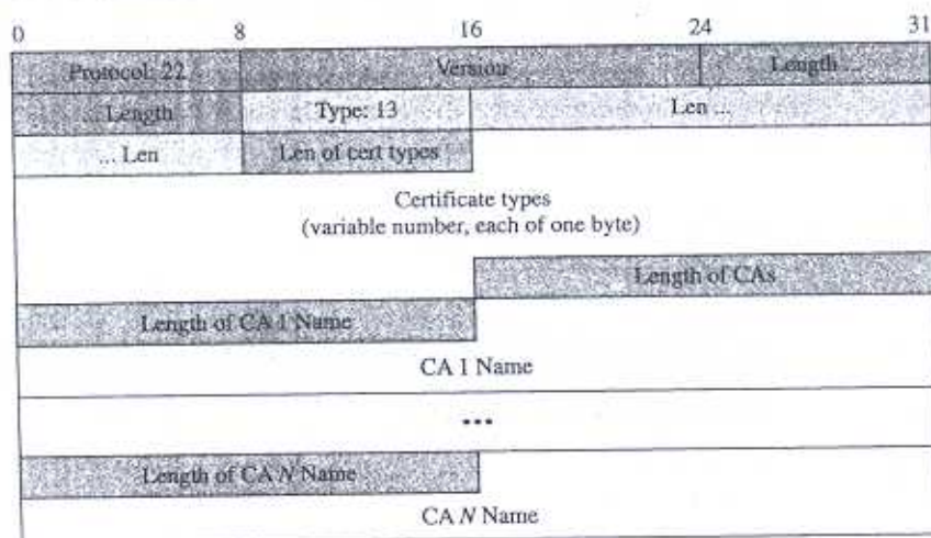
Figure 17.32 CertificateRequest message
