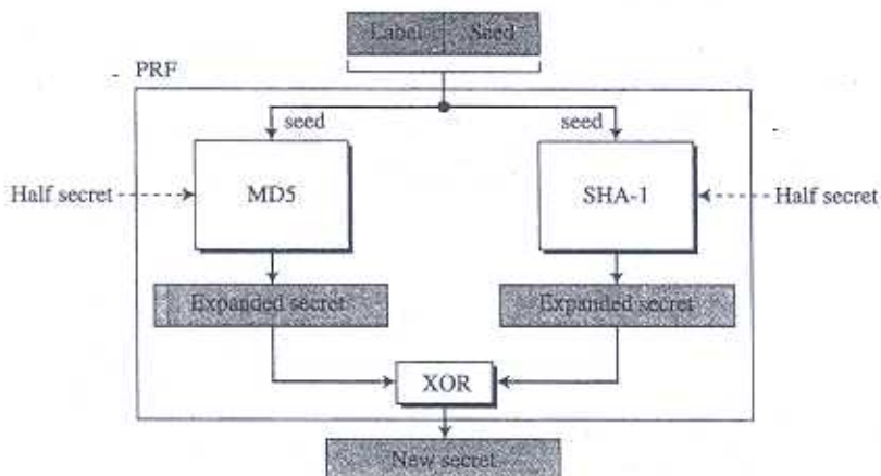
Figure 17.41 PRF
