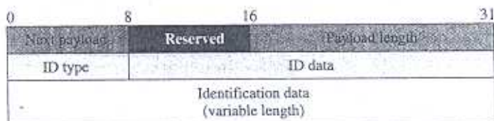
Figure 18.35 Identification payload
