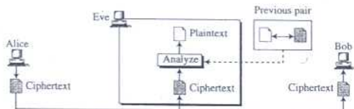
Figure 3.5 Known-plaintext attack
