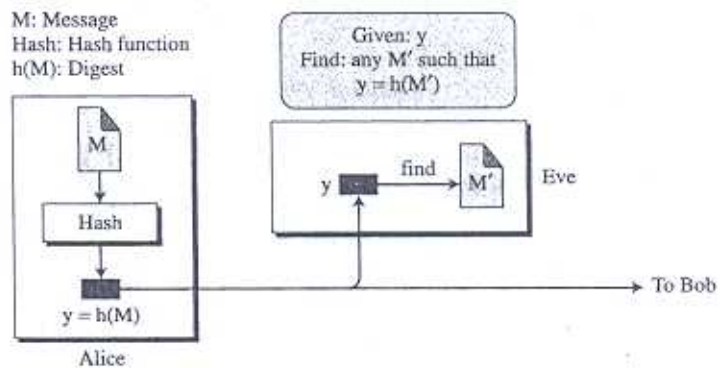
Figure 11.4 Preimage
