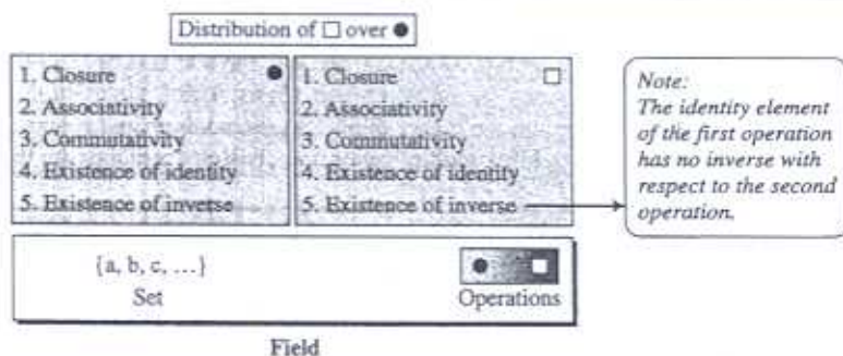
Figure 4.5 Field
