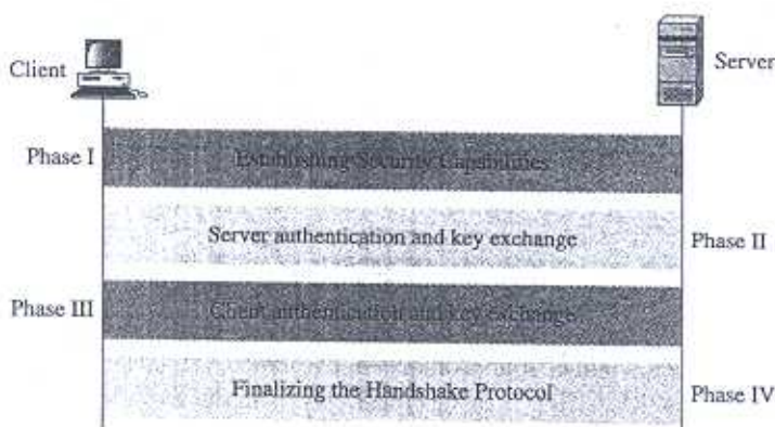
Figure 17.13 Handshake Protocol
