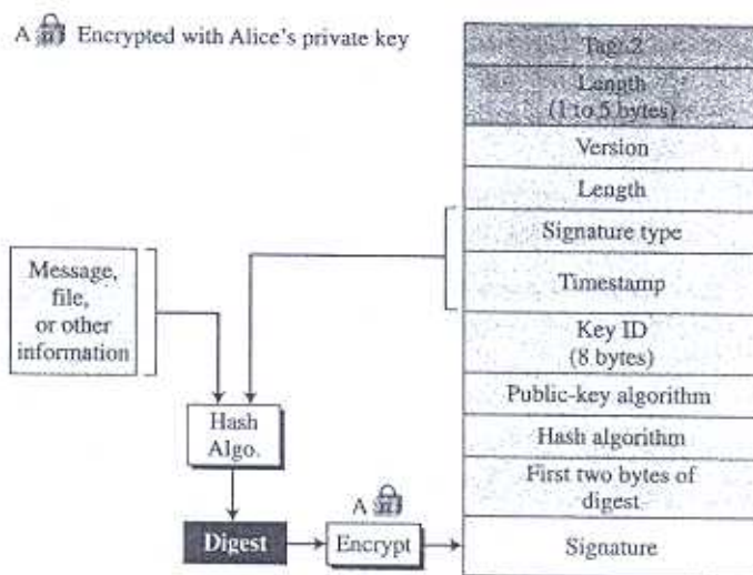
Figure 16.16 Signature packet
