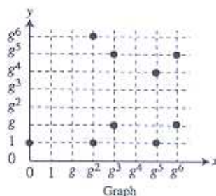
Figure 10.15 Points on an elliptic curve over GF(2^n)
