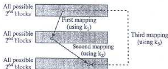
Figure 6.13 Composition of mapping
