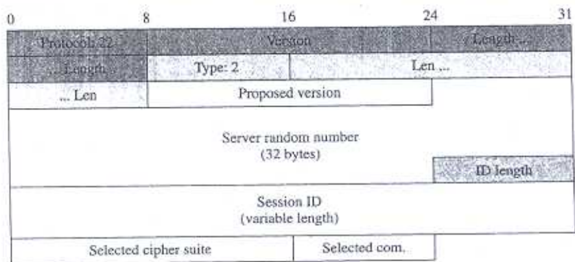
Figure 17.29 ServerHello message
