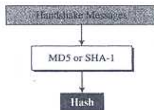
Figure 17.44 Hash for CertificateVerify message in TLS
