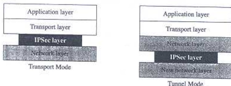
Figure 18.6 Transport mode versus tunnel mode
