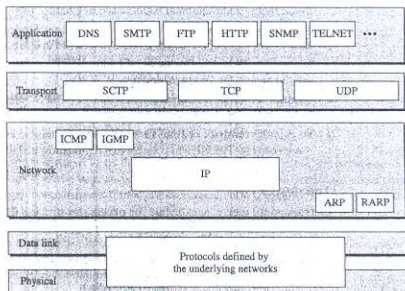
Figure C.1 TCP/IP protocol suite
