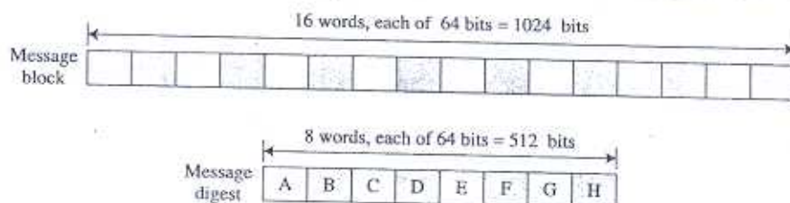
Figure 12.8 A message block and the digest as words
