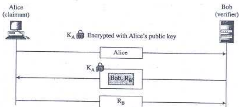
Figure 14.9 Unidirectional, asymmetric-key authentication
