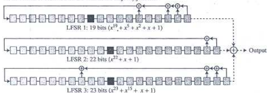
Figure 8.12 Three LFSR's in A5/1
