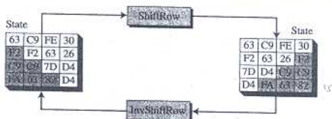
Figure 7.10 ShiftRows transformation in Example 7.4
