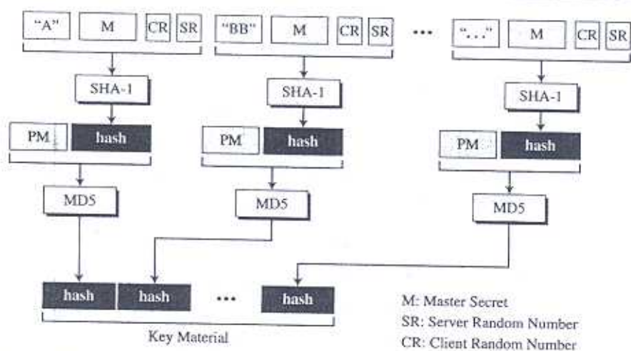
Figure 17.9 Calculation of key material from master secret
