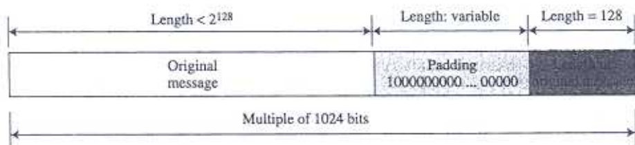
Figure 12.7 Padding and length field in SHA-512
