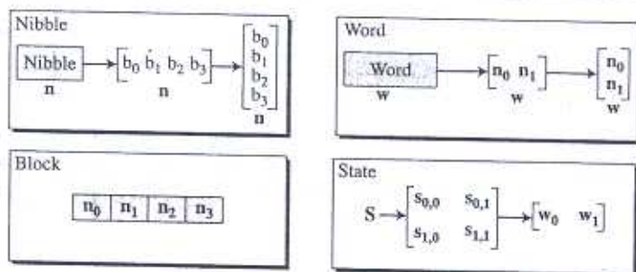
Figure P.3 Data units used in S-AES
