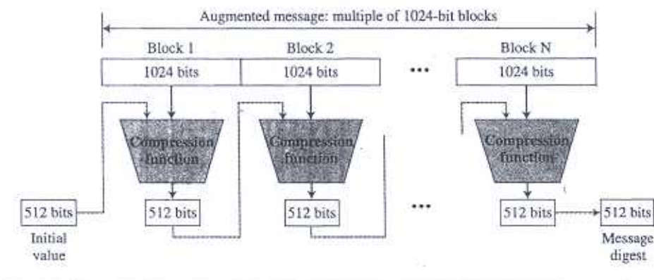
Figure 12.6 Message digest creation SHA-512
