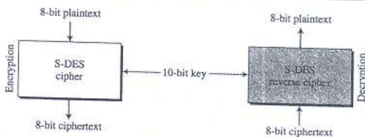
Figure O.1 Encryption and decryption with S-DES
