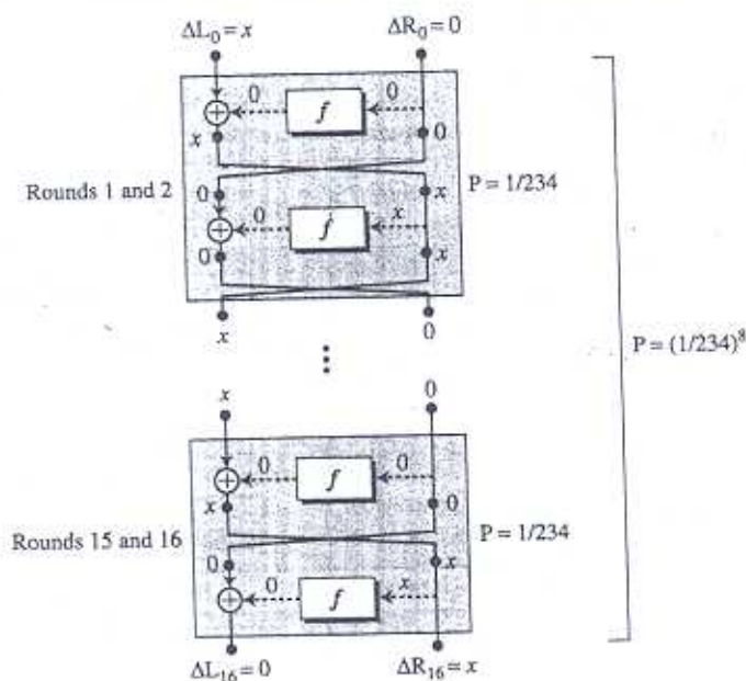
Figure N.4 A sixteen-round characteristic for differential cryptanalysis
