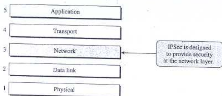
Figure 18.1 TCP/IP protocol suite and IPsec
