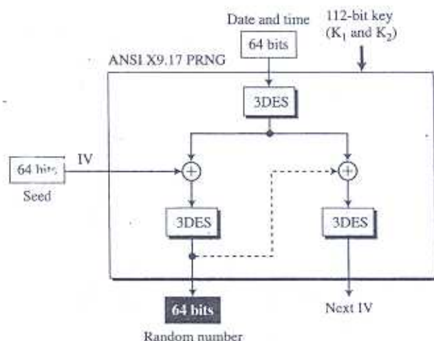
Figure K.4 ANSI X9.17 pseudorandom number generator
