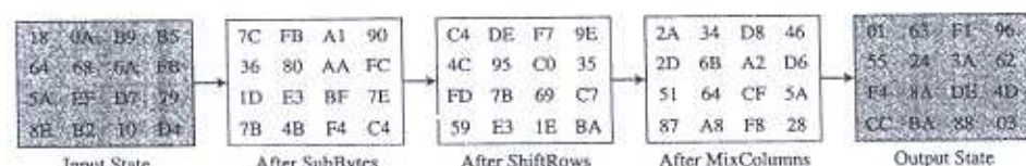
Figure 7.21 State in a single round
