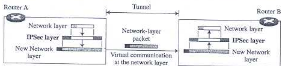
Figure 18.5 Tunnel mode in action
