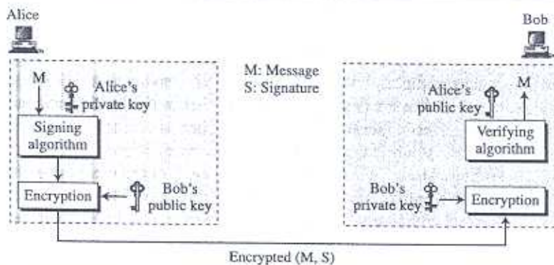
Figure 13.5 Adding confidentiality to a digital signature scheme
