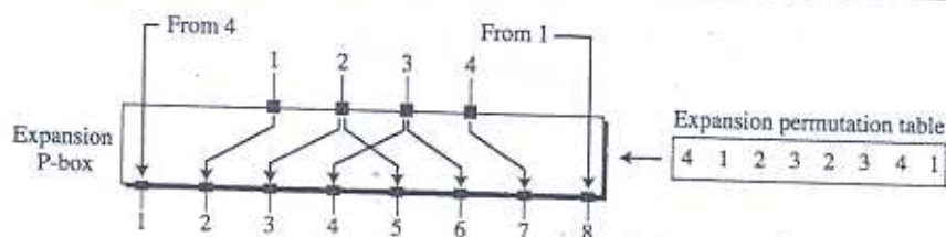
Figure O.5 Expansion P-box
