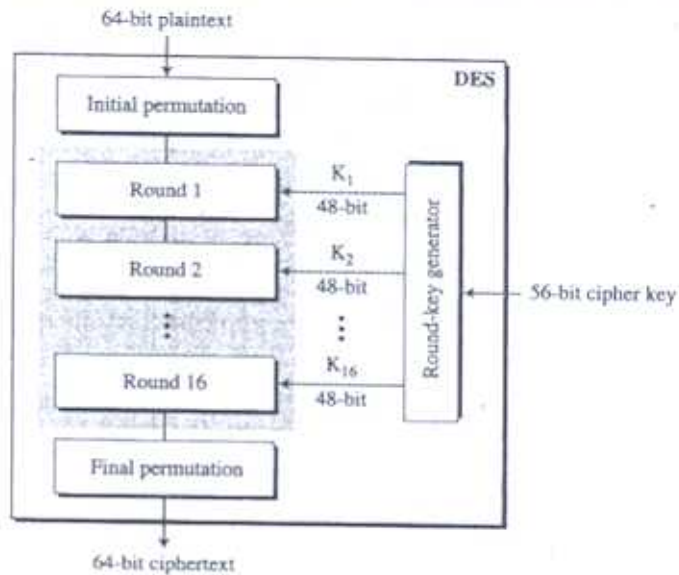
Figure 6.2 General structure of DES
