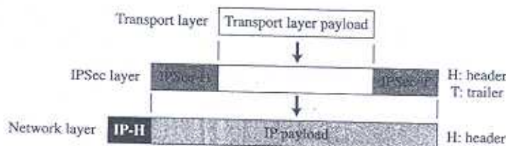
Figure 18.2 IPsec in transport mode
