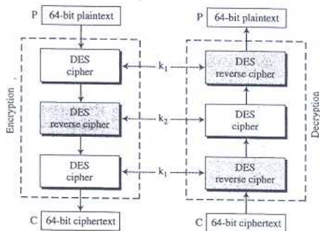
Figure 6.16 Triple DES with two keys
