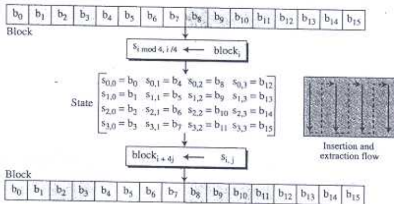
Figure 7.3 Block-to-state and state-to-block transformation
