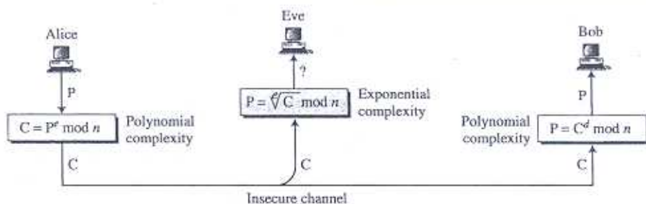
Figure 10.5 Complexity of operations in RSA
