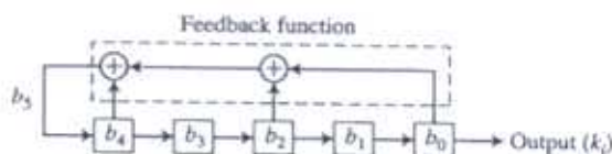
Figure 5.24 LFSR for Example 5.18
