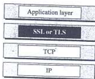
Figure 17.1 Location of SSL and TLS in the Internet model
