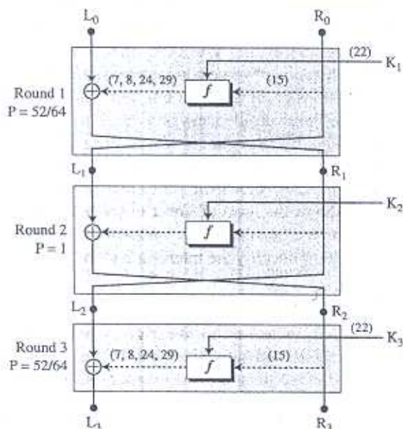
Figure N.7 A three-round characteristic for linear cryptanalysis
