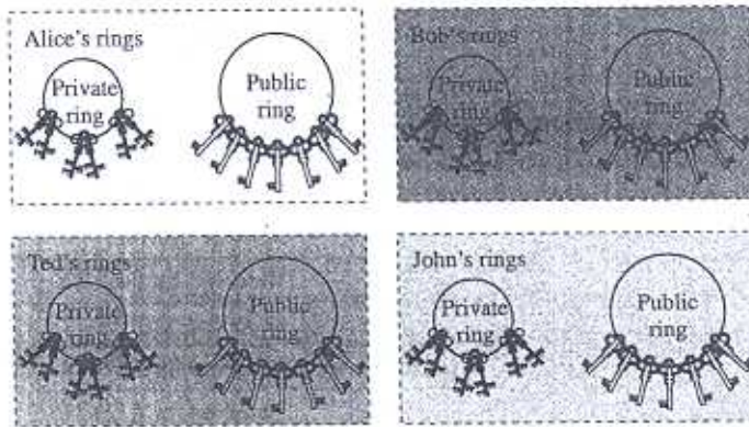
Figure 16.6 Key rings in PGP
