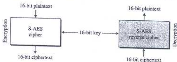
Figure P.1 Encryption and decryption with S-AES
