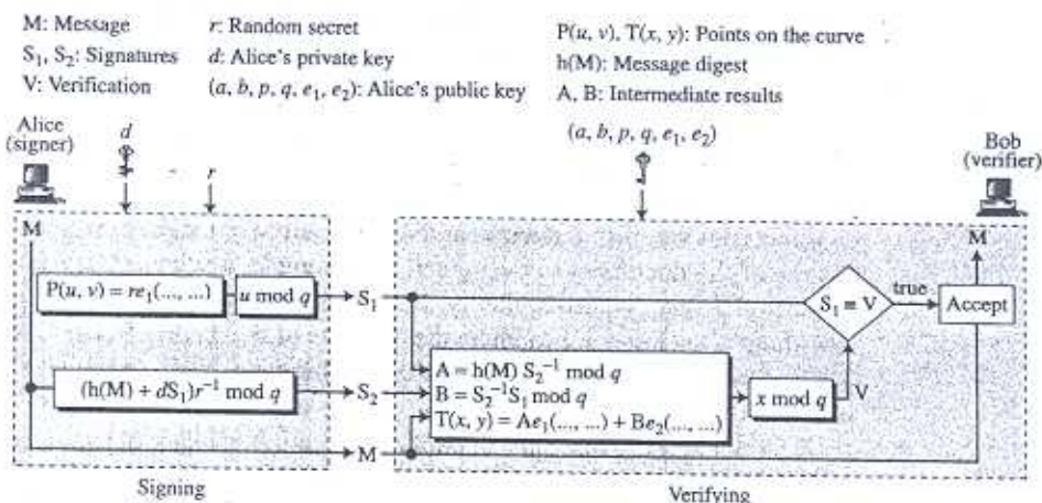
Figure 13.16 The ECDSS scheme
