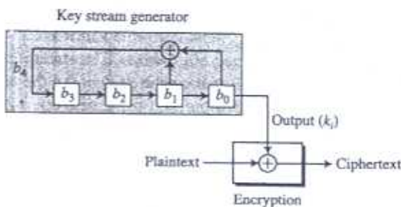
Figure 5.25 LFSR for Example 5.19
