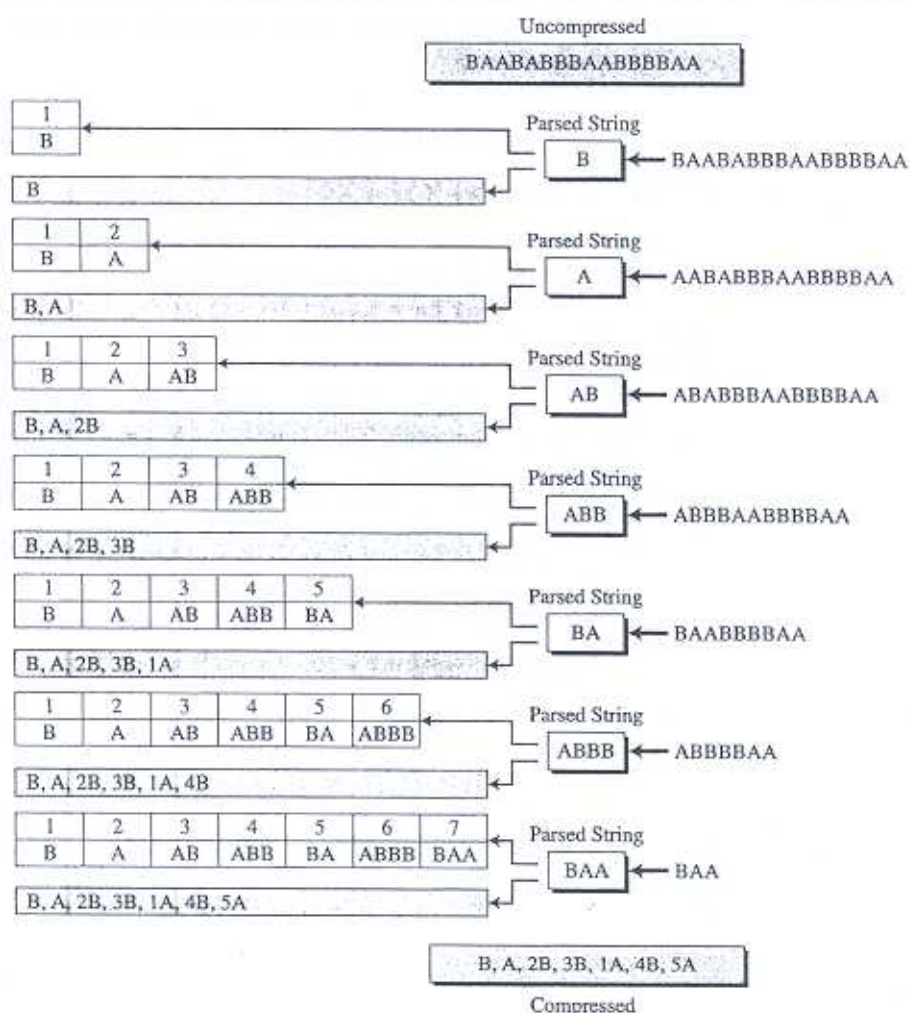
Figure M.1 Example of LZ77 encoding
