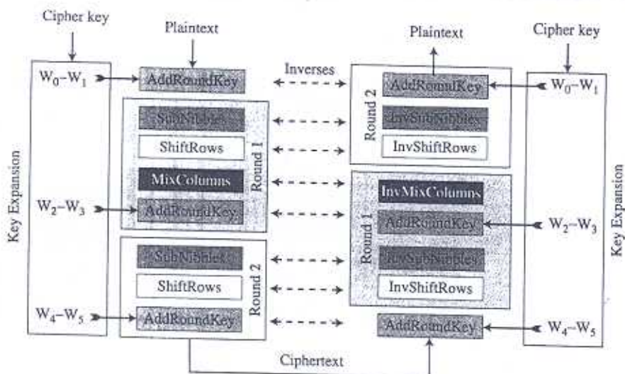
Figure P.15 Cipher and inverse cipher of the original design
