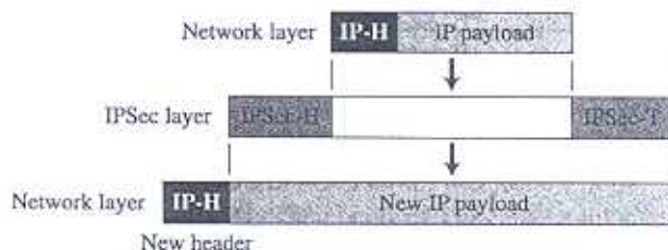
Figure 18.4 IPSec in tunnel mode
