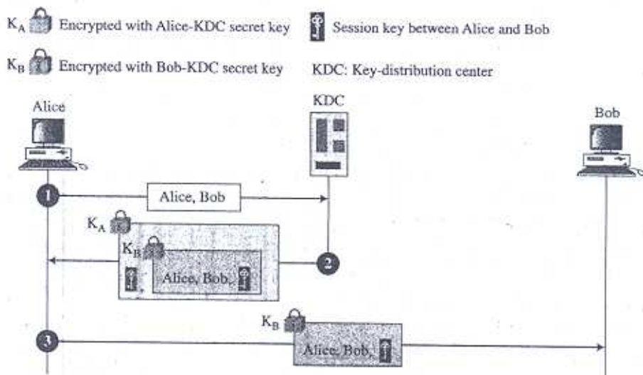
Figure 15.4 First approach using KDC
