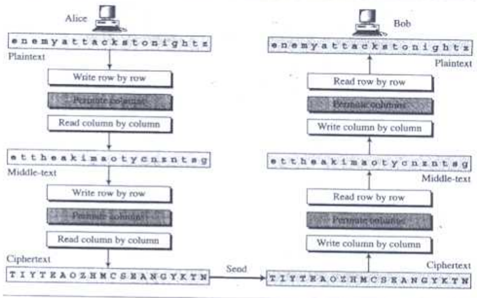
Figure 3.25 Double transposition cipher
