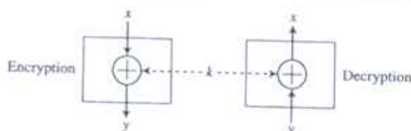
Figure 5.9 Invertibility of the exclusive-or operation
