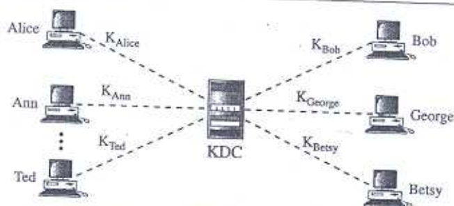
Figure 15.1 Key-distribution center (KDC)
