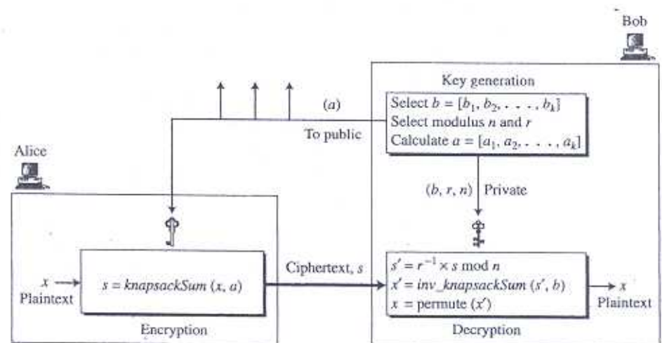
Figure 10.4 Secret communication with knapsack cryptosystem
