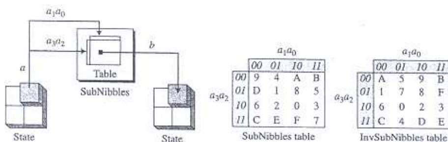
Figure P.7 SubNibbles transformations
