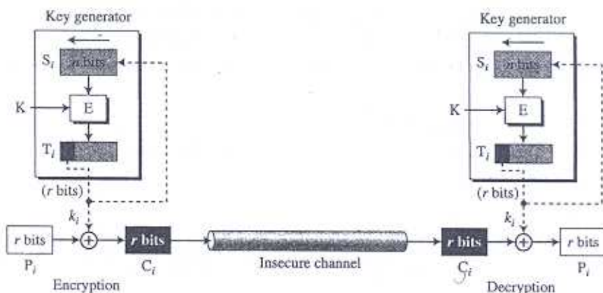
Figure 8.7 Output feedback (OFB) mode as a stream cipher
