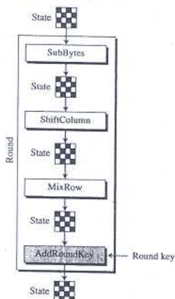
Figure 12.15 Structure of each round in the Whirlpool cipher
