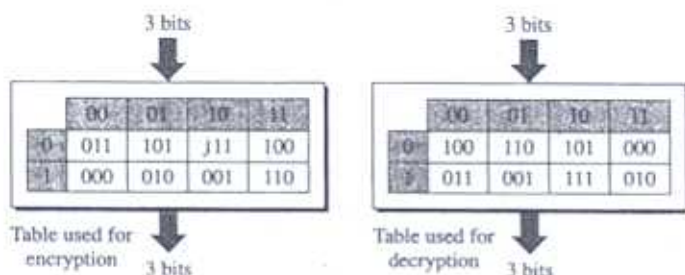
Figure 5.8 S-box tables for Example 5.11
