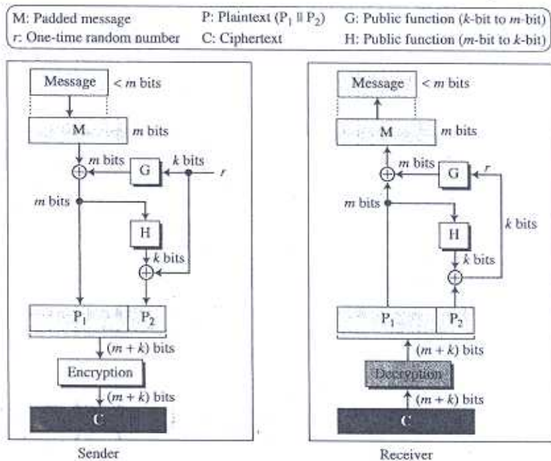
Figure 10.9 Optimal asymmetric encryption padding (OAEP)
