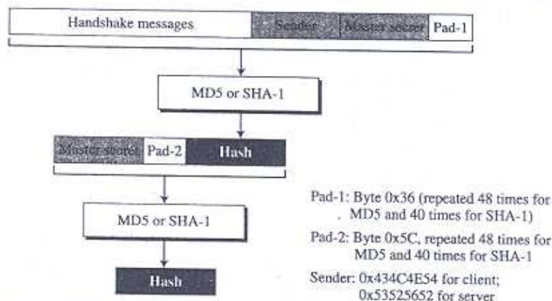
Figure 17.38 Hash calculation for Finished message
