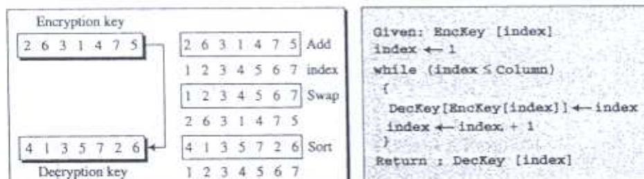
Figure 3.23 Key inversion in a transposition cipher
