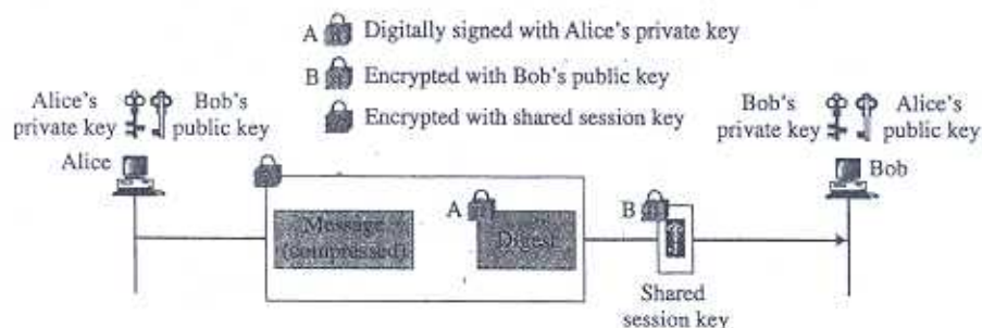
Figure 16.5 A confidential message
