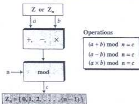
Figure 2.13 Binary operations in Z_n
