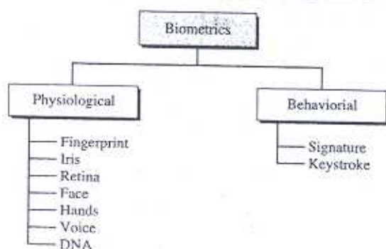
Figure 14.17 Biometrics
