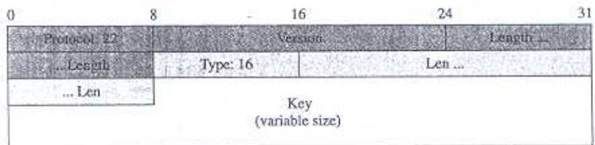
Figure 17.36 ClientKeyExchange message
