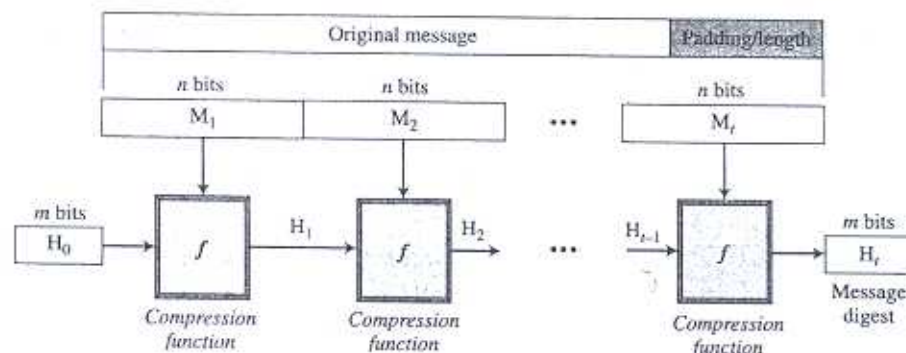
Figure 12.1 Merkle-Damgard scheme
