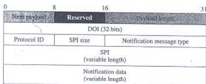
Figure 18.41 Notification payload
