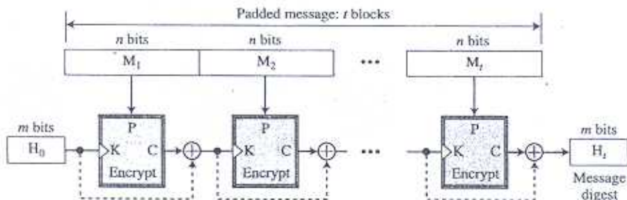
Figure 12.4 Matyas-Meyer-Oseas scheme
