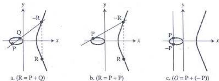
Figure 10.13 Three adding cases in an elliptic curve
