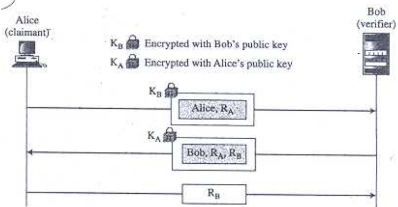
Figure 14.10 Bidirectional, asymmetric-key
