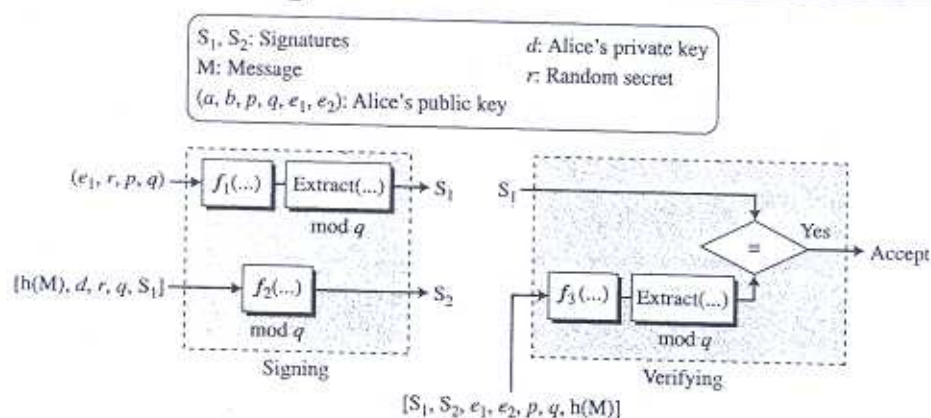
Figure 13.15 General idea behind the ECDSS scheme
