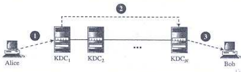
Figure 15.2 Flat multiple KDCs
