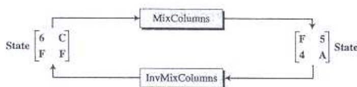
Figure P.12 The MixColumns transformation in Example 7.5
