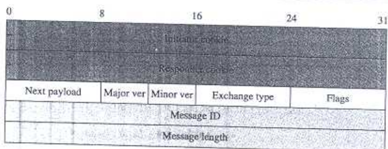
Figure 18.29 ISAKMP general header
