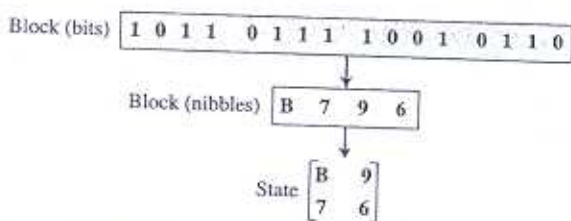
Figure P.5 Changing ciphertext to a state
