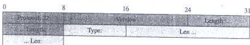
Figure 17.26 Generic header for Handshake Protocol
