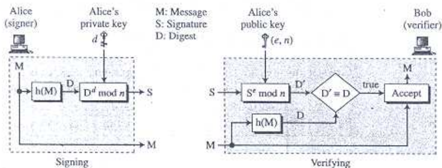
Figure 13.8 The RSA signature on the message digest
