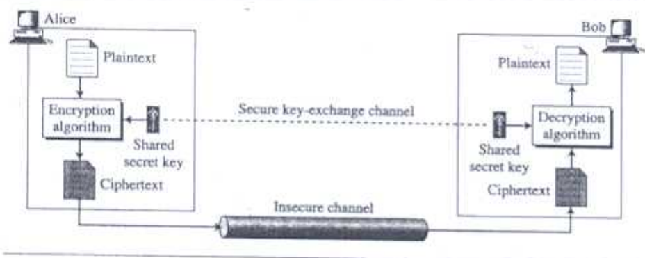
Figure 3.1 General idea of symmetric-key cipher
