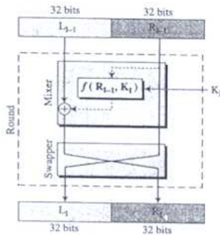
Figure 6.4 A round in DES (encryption site)
