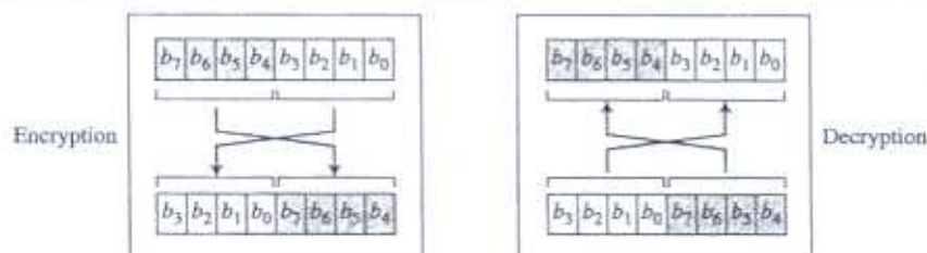
Figure 5.11 Swap operation on an 8-bit word
