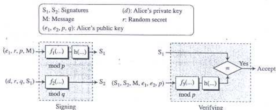
Figure 13.11 General idea behind the Schnorr digital signature scheme
