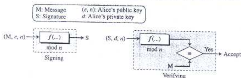
Figure 13.6 General idea behind the RSA digital signature scheme
