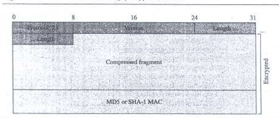
Figure 17.39 Record Protocol message for application data
