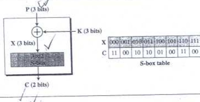
Figure 5.19 Diagram for Example 5.14
