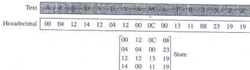
Figure 7.4 Changing ciphertext to state
