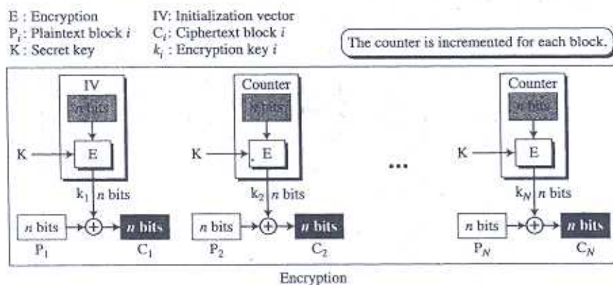
Figure 8.8 Encryption in counter (CTR) mode
