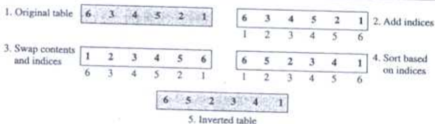
Figure 5.6 Inverting a permutation table
