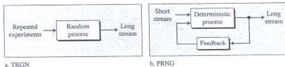
Figure K.1 TRNG and PRNG
