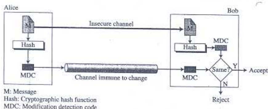
Figure 11.9 Modification detection code (MDC)
