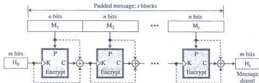
Figure 12.5 Miyaguchi-Preneel scheme
