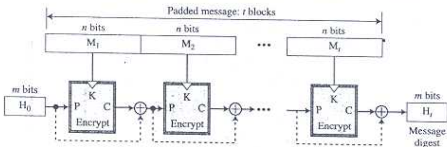
Figure 12.3 Davies-Meyer scheme
