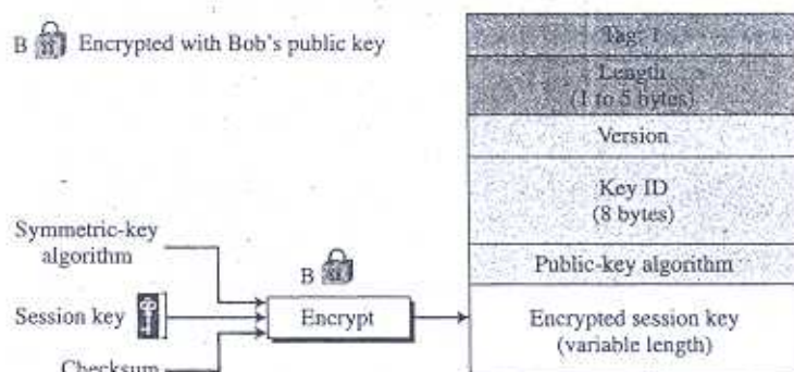
Figure 16.17 Session-key packet
