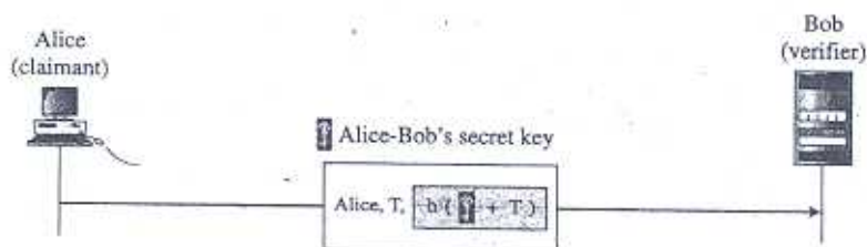
Figure 14.8 Keyed-hash function
