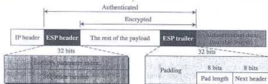
Figure 18.8 ESP
