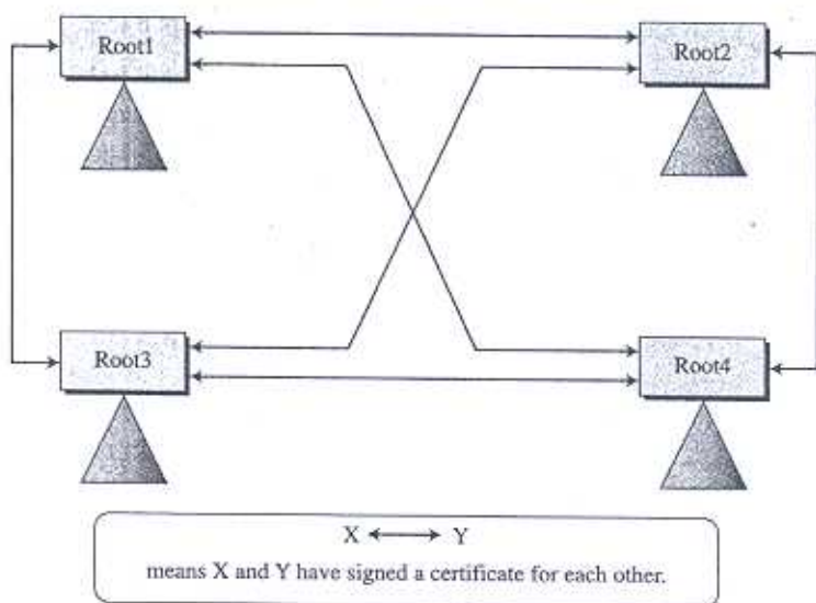
Figure 15.21 Mesh model
