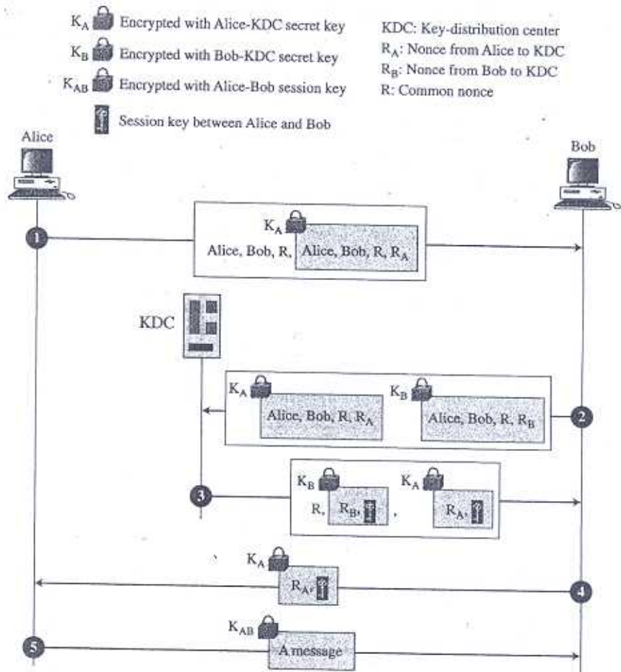
Figure 15.6 Otway-Rees protocol
