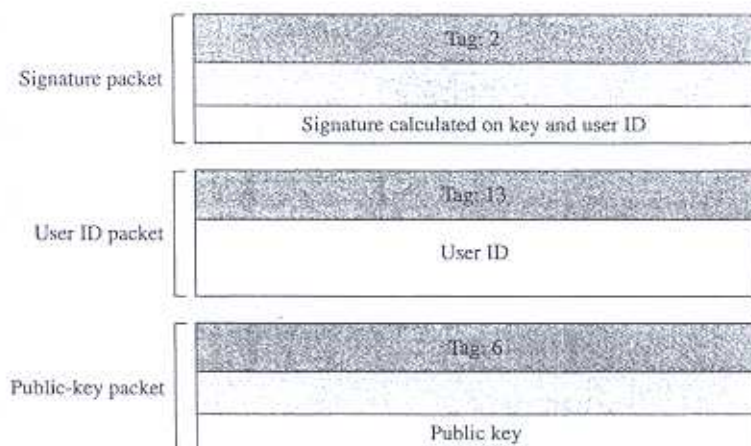
Figure 16.22 Certificate message
