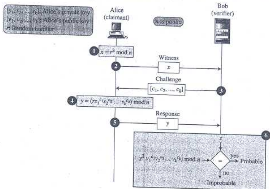
Figure 14.15 Feige-Fiat-Shamir protocol
