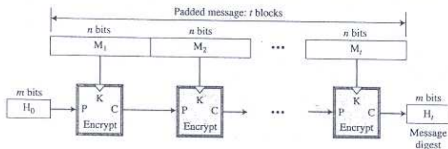
Figure 12.2 Rabin scheme
