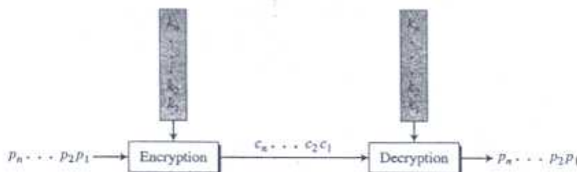
Figure 5.21 Stream cipher
