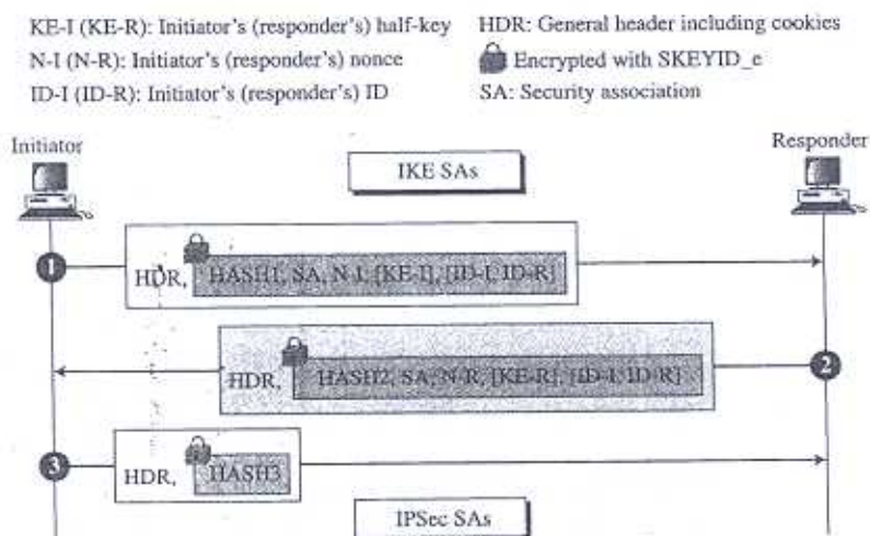
Figure 18.28 Quick mode
