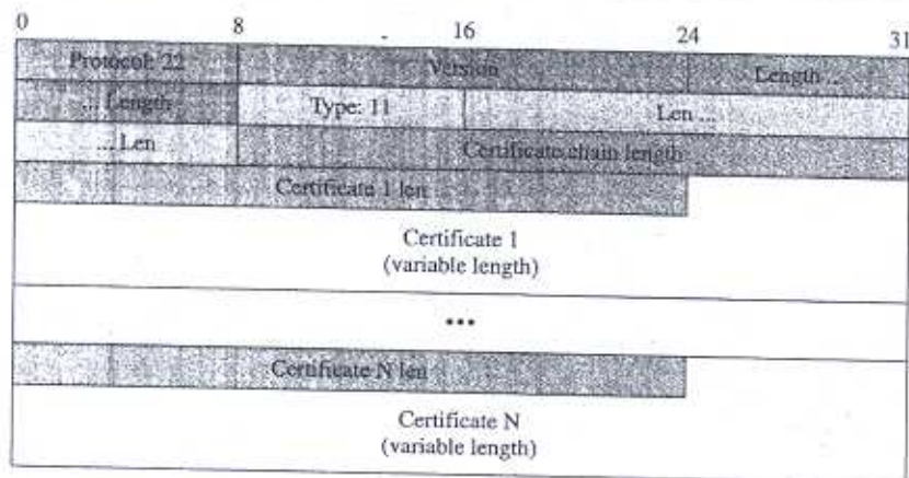
Figure 17.30 Certificate message
