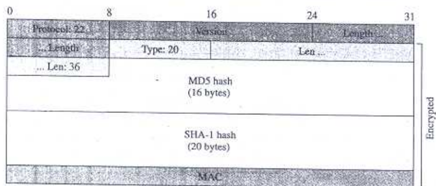
Figure 17.37 Finished message
