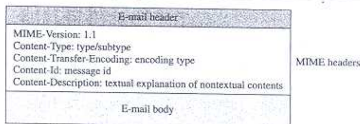
Figure 16.24 MIME header
