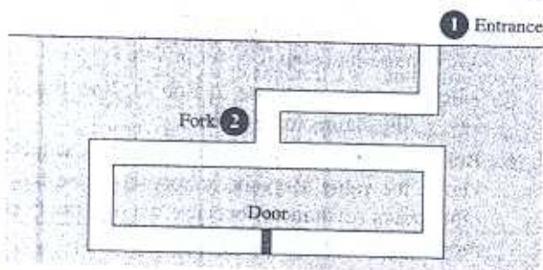
Figure 14.14 Cave example
