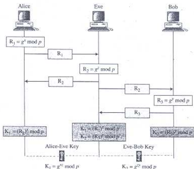
Figure 15.11 Man-in-the-middle attack
