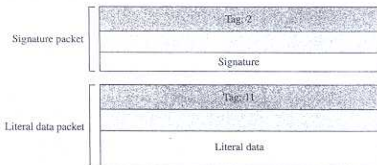
Figure 16.21 Signed message
