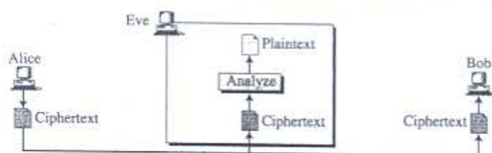
Figure 3.4 Ciphertext-only attack
