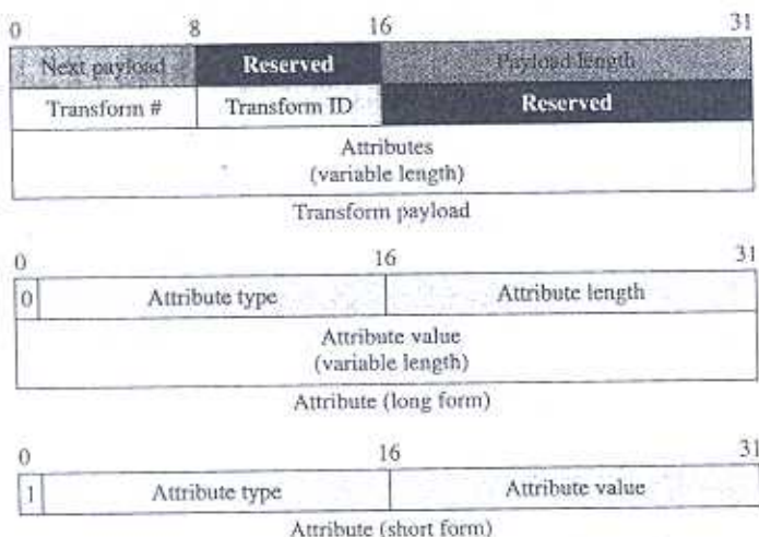
Figure 18.33 Transform payload
