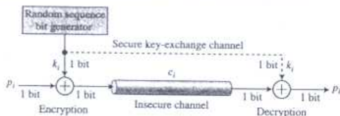
Figure 5.22 One-time pad
