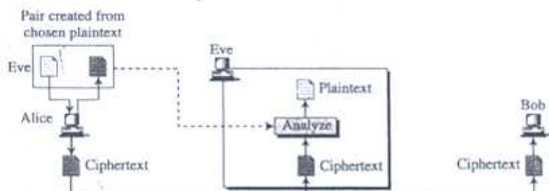
Figure 3.6 Chosen-plaintext attack
