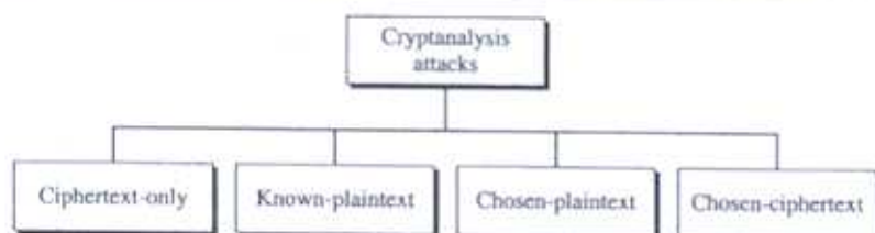
Figure 3.3 Cryptanalysis attacks
