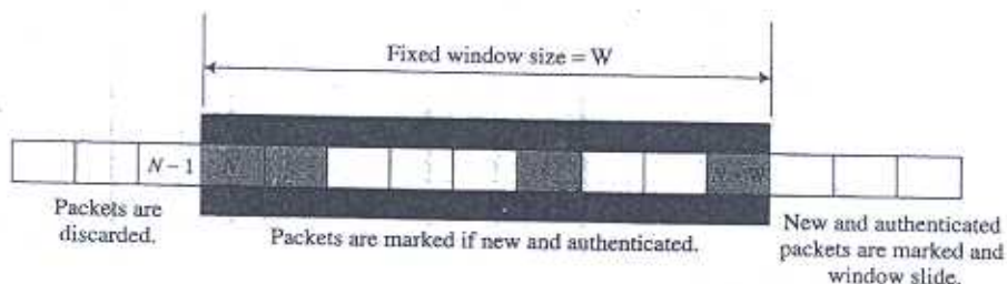
Figure 18.9 Replay window
