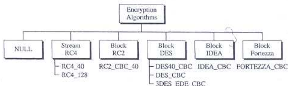
Figure 17.6 Encryption/decryption algorithms
