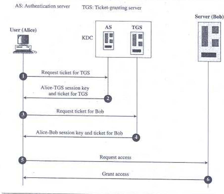
Figure 15.7 Kerberos servers
