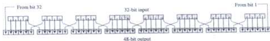
Figure 6.6 Expansion permutation
