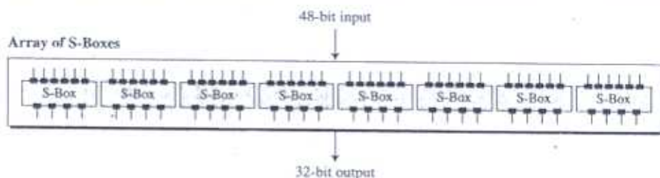
Figure 6.7 S-boxes
