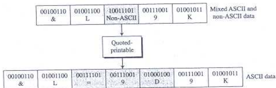
Figure 16.26 Quoted-printable
