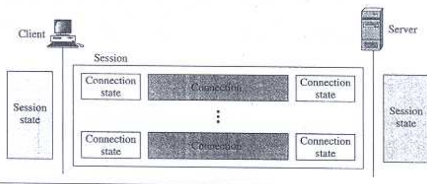
Figure 17.11 A session and connections
