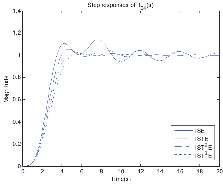
Figure 8.1 Step responses for j = 4
