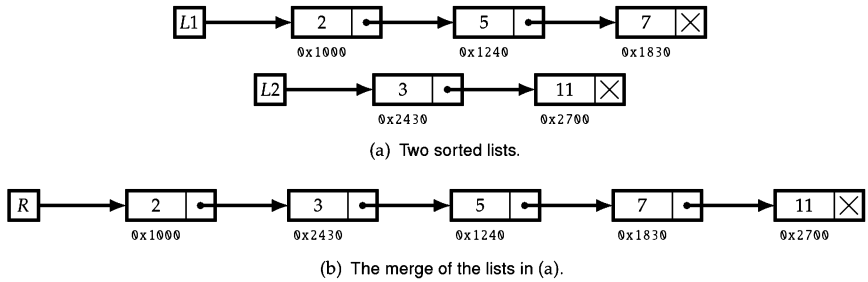
Figure 8.3: Merging sorted lists.
