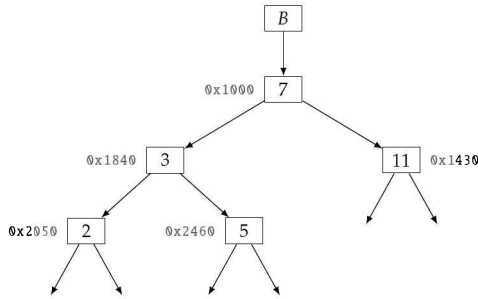
(a) A BST on five nodes—edges that do not terminate in nodes denote empty subtrees. The number in hex adjacent to each node represents its address in memory.
