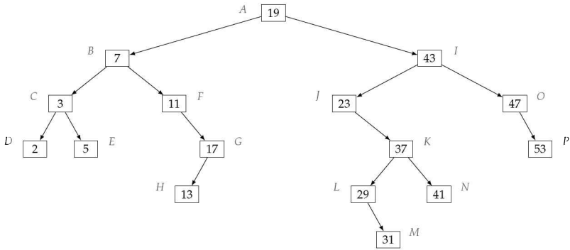
Figure 15.1: An example of a BST.
