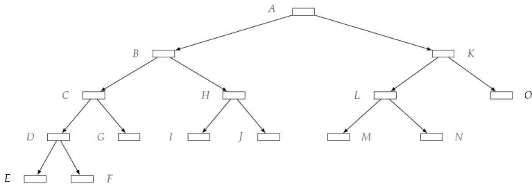
Figure 10.2: A height-balanced binary tree of height 4.
