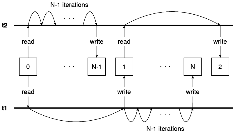
Figure 20.1: Worst-case schedule for two unsynchronized threads.
