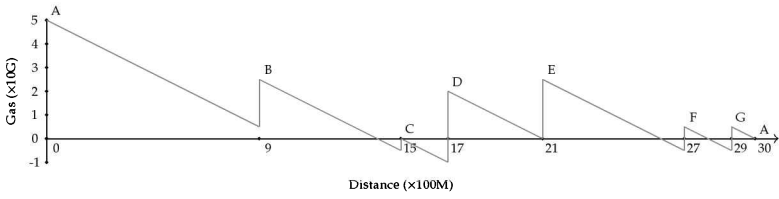
(a) Gas vs. distance, starting at A.
