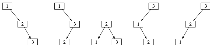
Figure 15.3: Five distinct BSTs for the traversal sequence \langle 1, 2, 3 \rangle .
