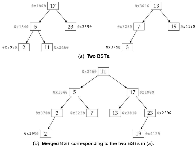
Figure 25.5: Example of merging two BSTs. The number in hex adjacent to each node represents its address in memory.
