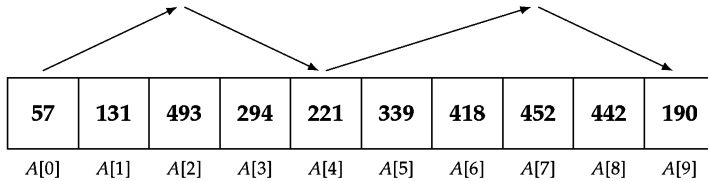
Figure 11.2: A 4-increasing-decreasing array.
