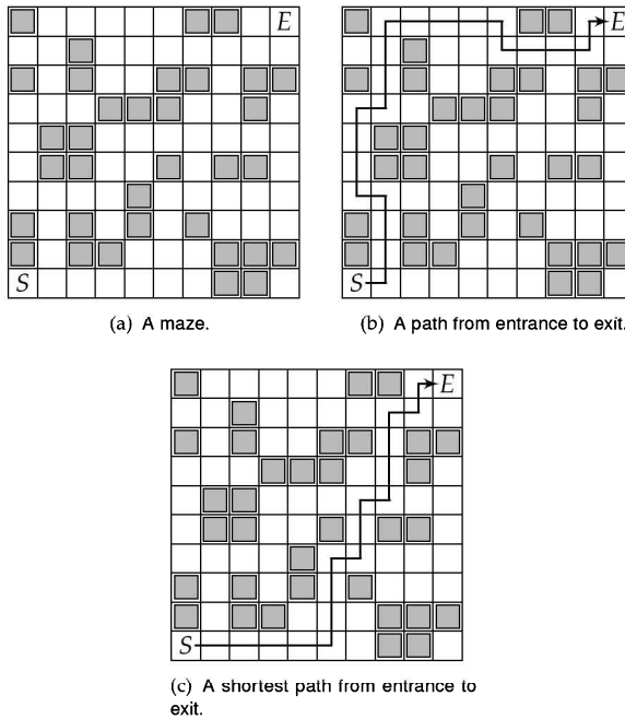
Figure 19.5: An instance of the maze search problem, with two solutions, where S and E denote the entrance and exit, respectively.
