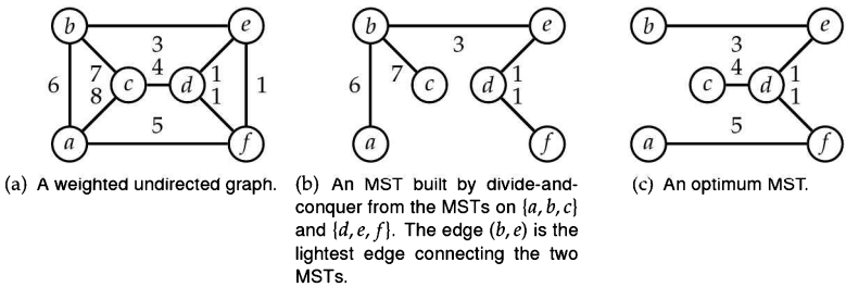
Figure 19.9: Divide-and-conquer applied to the MST problem is suboptimum—the MST in (b) has weight 18, but the MST in (c) has weight 14.
