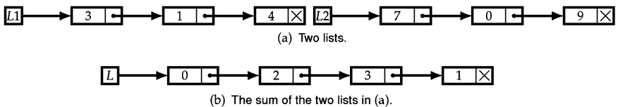
Figure 8.12: List-based interpretation of 413 + 907 = 1320 .
