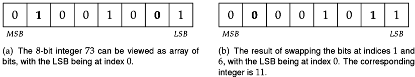
Figure 5.1: Example of swapping a pair of bits.
