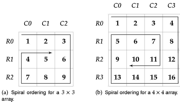
Figure 6.3: Spiral orderings. Column and row ids are specified above and to the left of the matrix, i.e., 1 is at entry (0, 0) .
