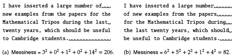
Figure 17.12: Two layouts for the same sequence of words; the line length L is 36.
