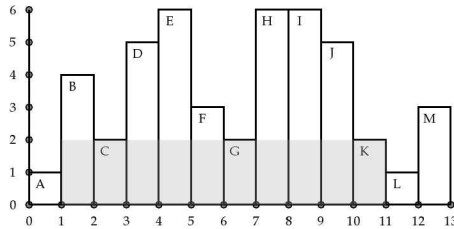
Figure 18.5: A collection of unit-width buildings, and the largest contained rectangle. The text label identifying the building is just below and to the right of its upper left-hand corner. The shaded area is the largest rectangle under the skyline. Its area is 2 \times (11 - 1) . Note that the tallest rectangle is from 7 to 9, and the widest rectangle is from 0 to 1, but neither of these are the largest rectangle under the skyline.
