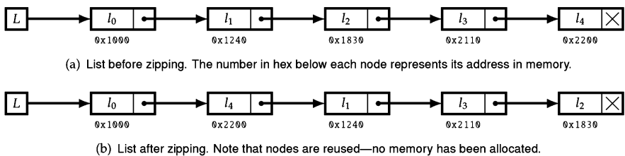
Figure 4.1: Zipping a list.
