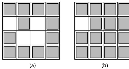
Figure 19.7: Three of the four white squares in (a) are enclosed , i.e., there is no path from any of them to the boundary that only passes through white squares. (b) shows the white squares that are not enclosed.
