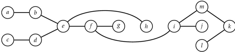
Figure 19.4: A tree.
