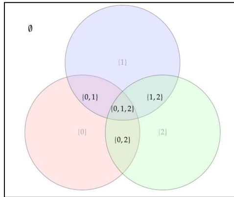
Figure 16.4: The power set of \{0, 1, 2\} is \{\emptyset, \{0\}, \{1\}, \{2\}, \{0, 1\}, \{1, 2\}, \{0, 2\}, \{0, 1, 2\}\} .
