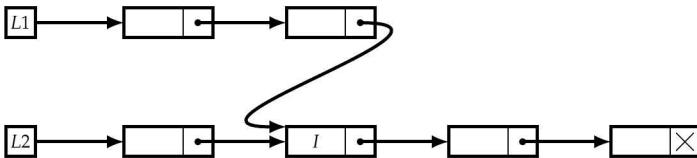
Figure 8.6: Example of overlapping lists.
