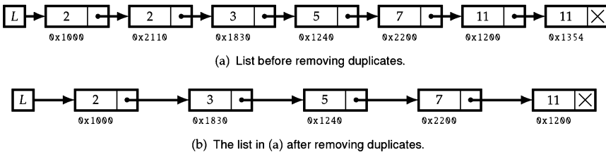
Figure 8.8: Example of duplicate removal.
