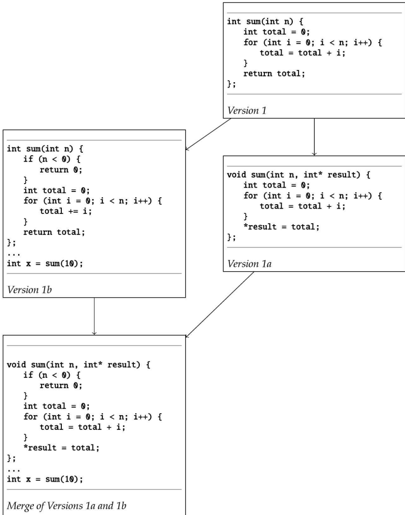
Figure 24.1: An example of a 3-way line based merge.
