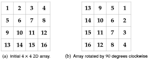
Figure 6.4: Example of 2D array rotation.
