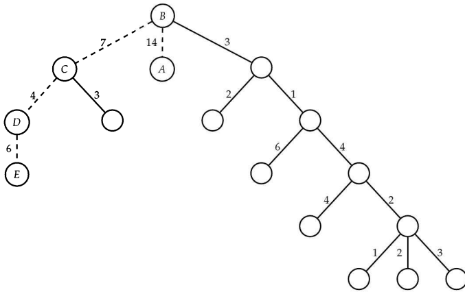
Figure 16.6: The diameter for the above tree is 31. The corresponding path is \langle A, B, C, D, E \rangle , which is depicted by the dashed edges.
