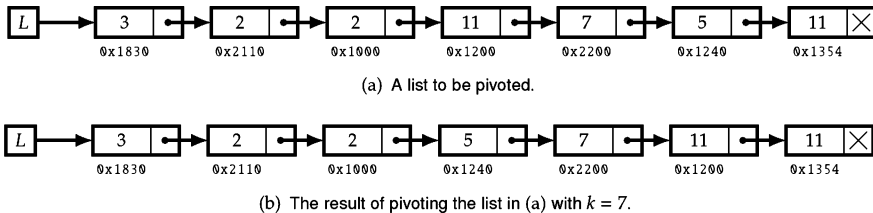
Figure 8.11: List pivoting.
