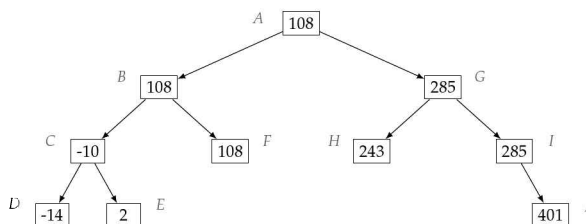
Figure 15.2: A BST with duplicate keys.
