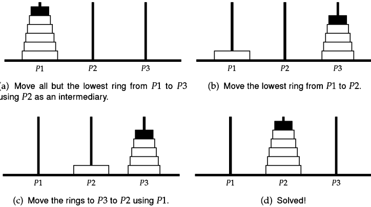
Figure 16.2: A recursive solution to the Tower of Hanoi for n = 6 .
