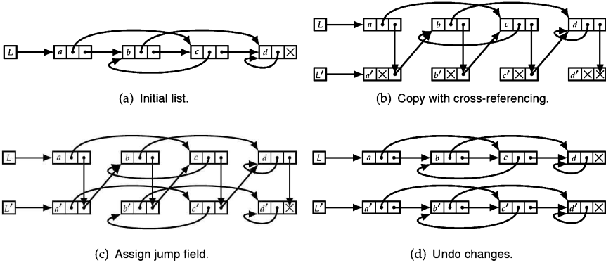
Figure 25.2: Duplicating a postings list.
