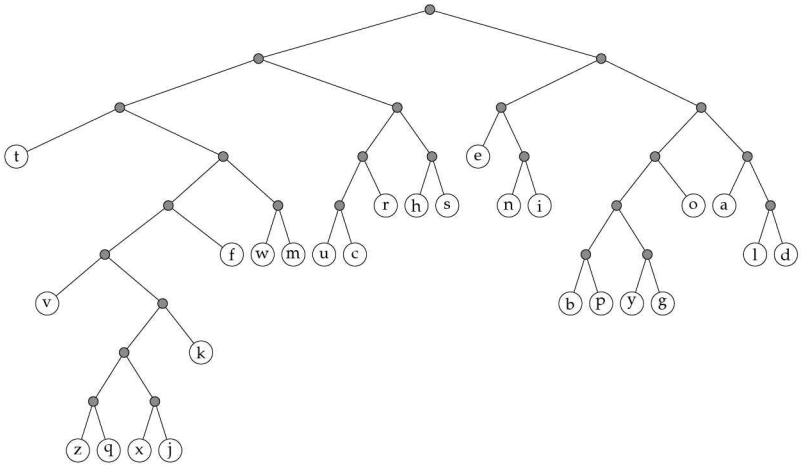
Figure 25.8: A Huffman tree for the English characters, assuming the frequencies given in Table 25.1 on Page 497.
