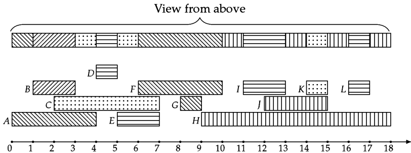
Figure 25.6: Instance of the view from above problem, with patterns used to denote colors. Letters label input line segments.
