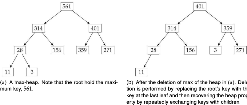
Figure 11.1: A max-heap and deletion on that max-heap.
