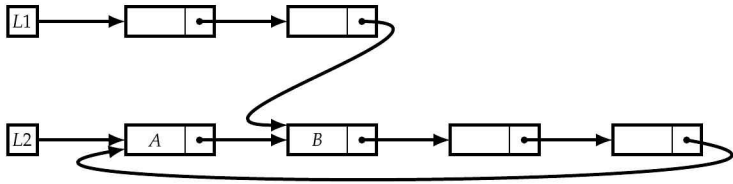
Figure 8.7: Overlapping lists.
