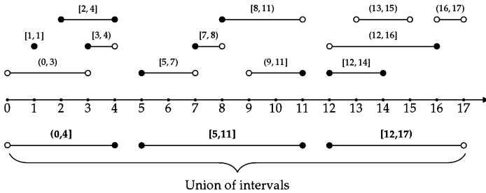
Figure 14.2: A set of intervals and their union.
