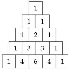
Figure 6.5: A Pascal triangle.
