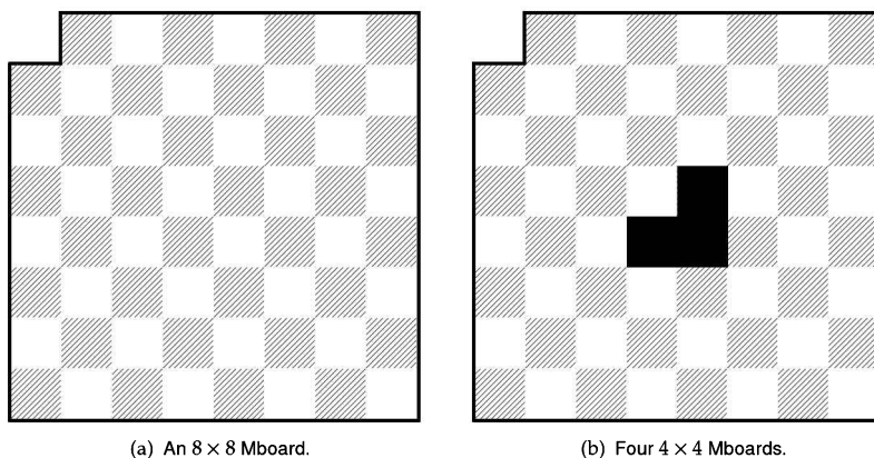
Figure 4.2: Mutilated chessboards.
