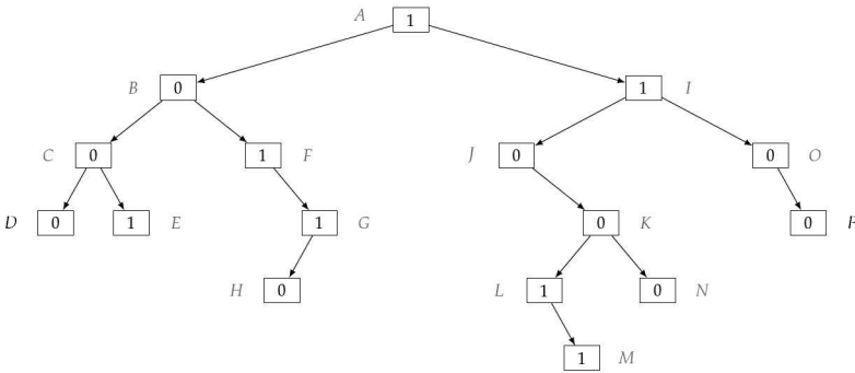
Figure 10.4: Binary tree encoding integers.
