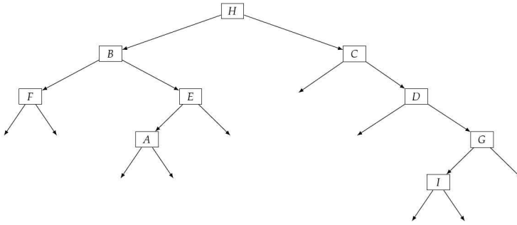
Figure 10.5: A binary tree—edges that do not terminate in nodes denote empty subtrees.
