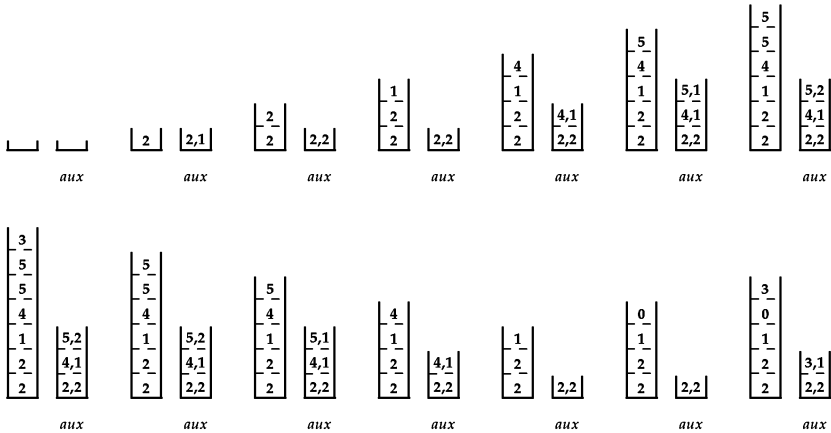
Figure 9.2: The primary and auxiliary stacks for the following operations: push 2, push 2, push 1, push 4, push 5, push 5, push 3, pop, pop, pop, pop, push 0, push 3. Both stacks are initially empty, and their progression is shown from left-to-right, then top-to-bottom. The top of the auxiliary stack holds the maximum element in the stack, and the number of times that element occurs in the stack. The auxiliary stack is denoted by aux .
