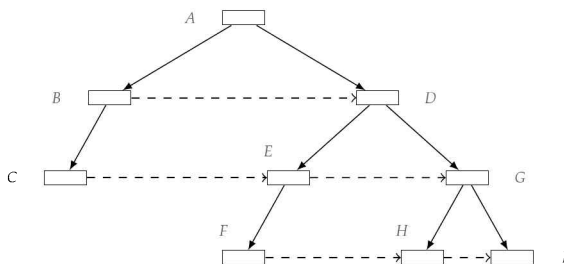
Figure 10.7: Assigning each node's level-next field to its right sibling in a general binary tree. A dashed arrow indicates the value held by the level-next field after the update.
