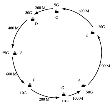
Figure 18.2: The length of the circular road is 3000 miles, and your vehicle gets 20 miles per gallon. The distance noted at each city is how far it is from the next city. For this configuration, we can begin with no gas at City D, and complete the circuit successfully, so D is an ample city.
