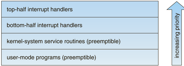
Figure 16.2 Interrupt protection levels.
