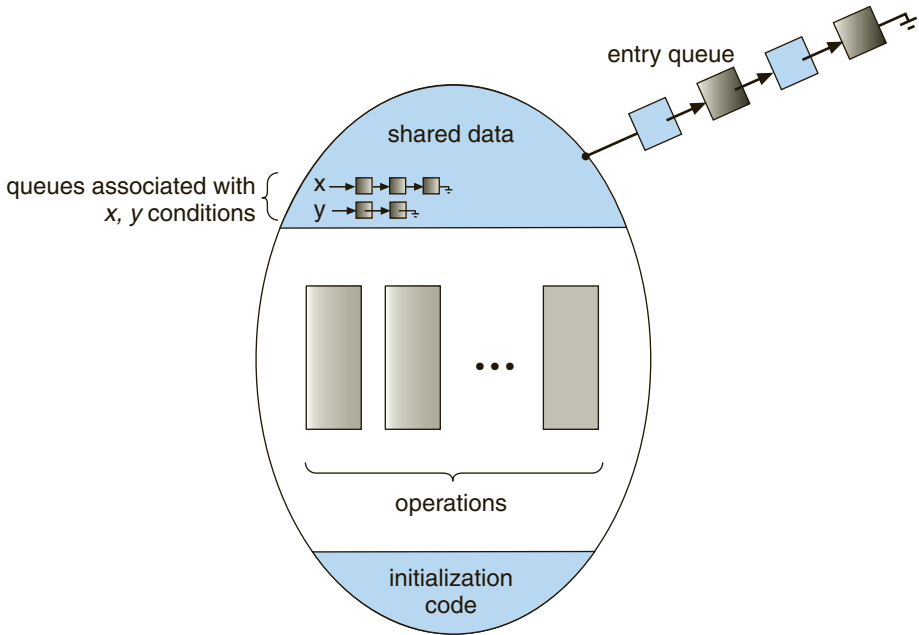
Figure 6.17 Monitor with condition variables.
