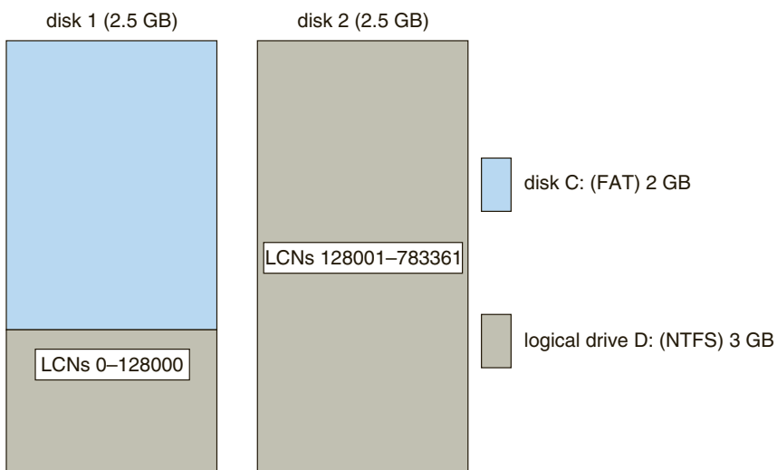
Figure 17.7 Volume set on two drives.
