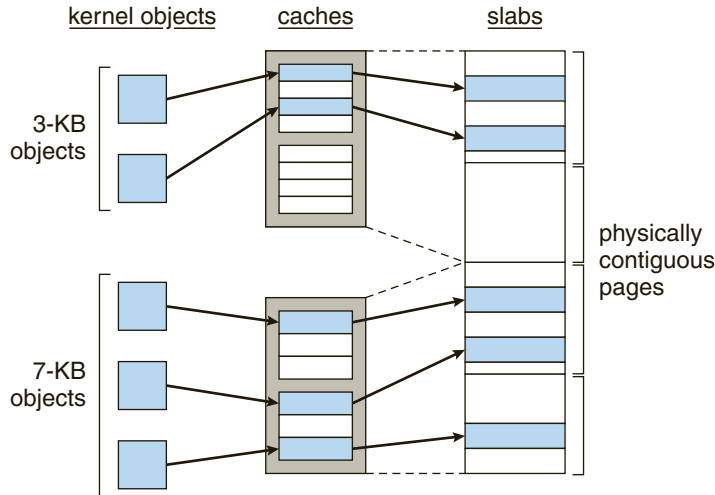
Figure 16.5 Slab allocator in Linux.
