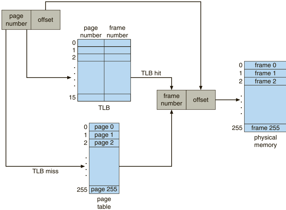
Figure 9.33 A representation of the address-translation process.
