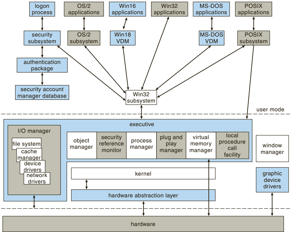
Figure 17.1 Windows block diagram.
