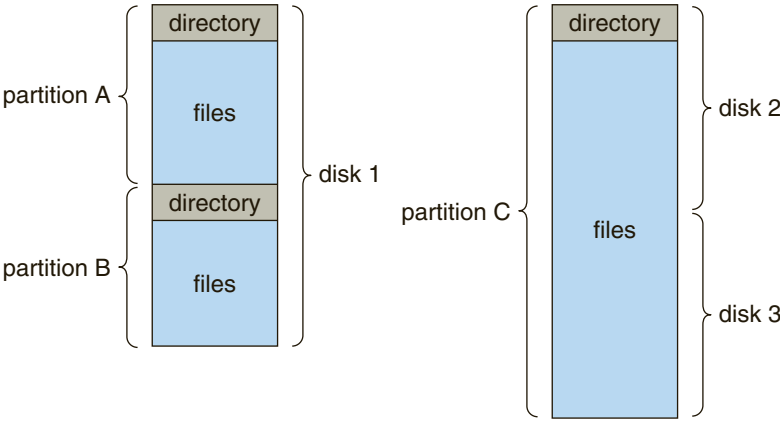
Figure 10.7 A typical file-system organization.
