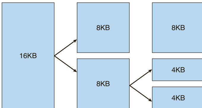
Figure 16.4 Splitting of memory in the buddy system.
