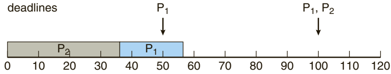
Figure 5.16 Scheduling of tasks when P_2 has a higher priority than P_1 .
