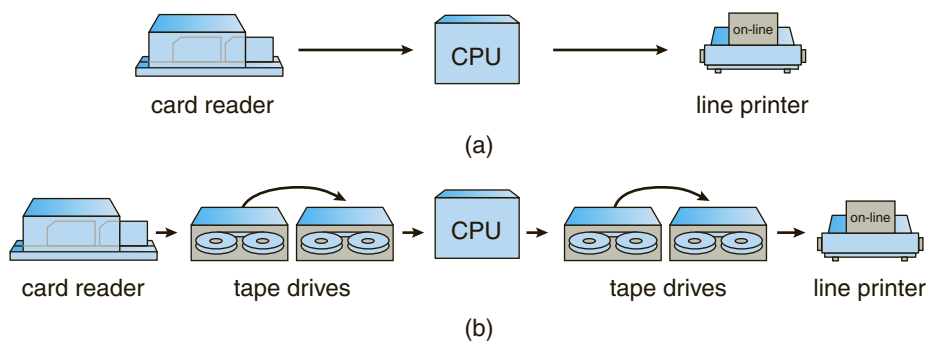
Figure 18.4 Operation of I/O devices (a) on-line and (b) off-line.
