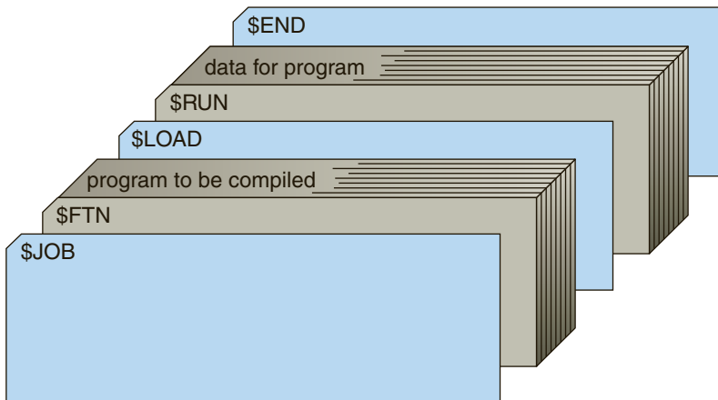
Figure 18.3 Card deck for a simple batch system.
