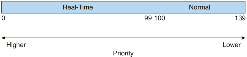
Figure 5.21 Scheduling priorities on a Linux system.
