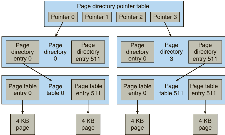
Figure 17.3 Page-table layout.
