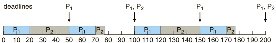
Figure 5.17 Rate-monotonic scheduling.
