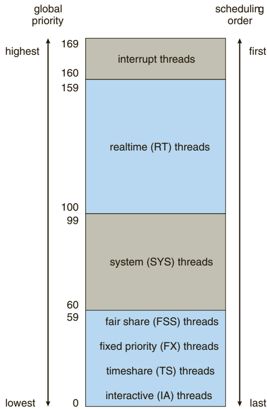
Figure 5.24 Solaris scheduling.
