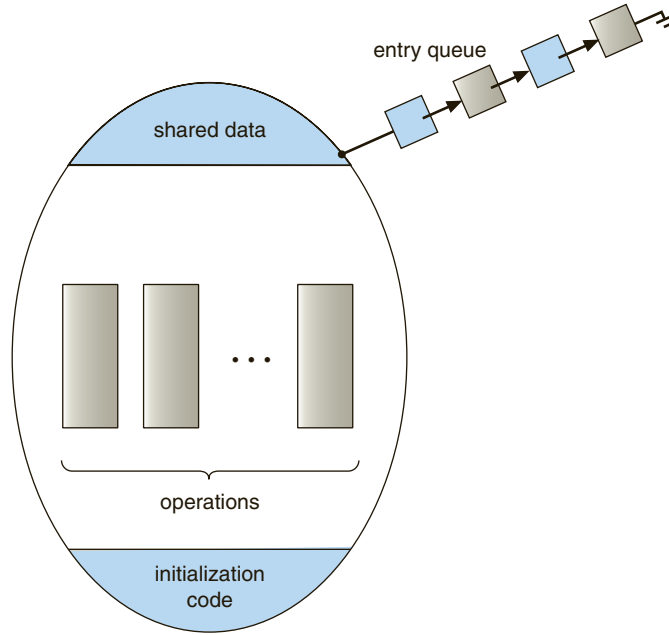
Figure 6.16 Schematic view of a monitor.
