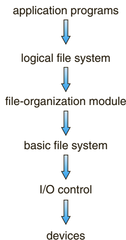
Figure 11.1 Layered file system.
