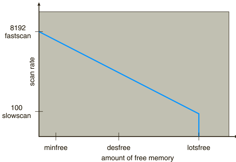
Figure 9.29 Solaris page scanner.
