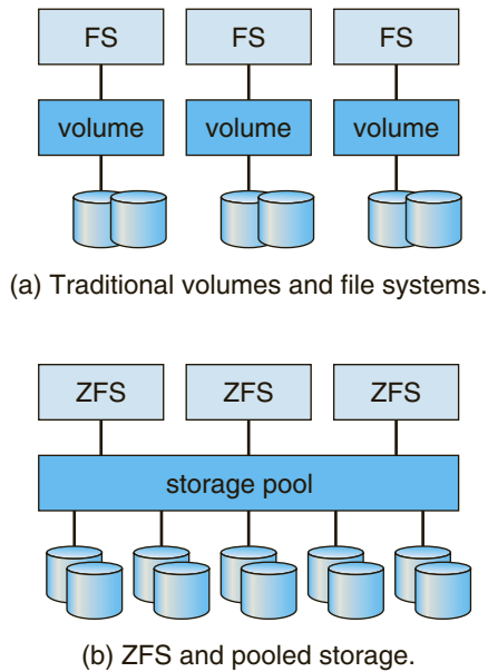
Figure 12.14 (a) Traditional volumes and file systems. (b) A ZFS pool and file systems.
