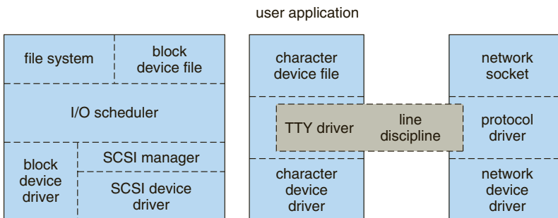
Figure 16.8 Device-driver block structure.
