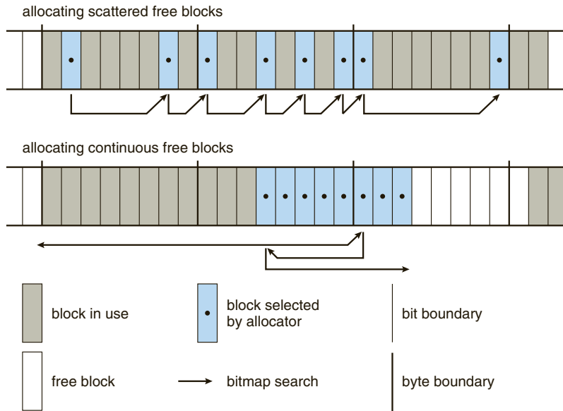
Figure 16.7 ext3 block-allocation policies.
