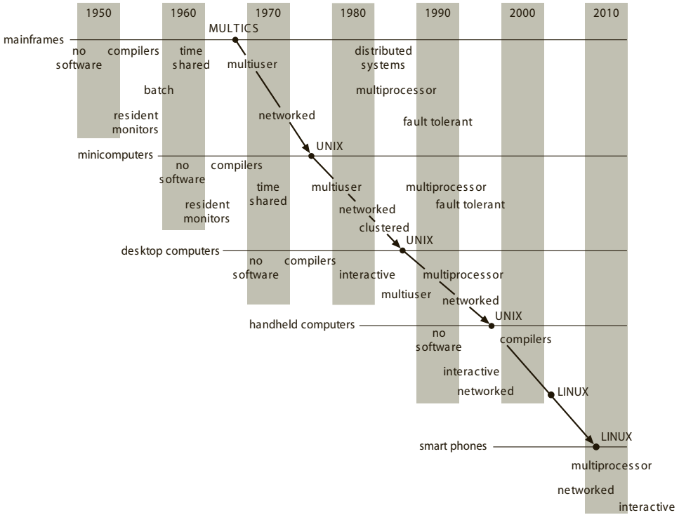
Figure 18.1 Migration of operating-system concepts and features.
