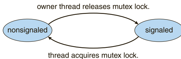
Figure 6.20 Mutex dispatcher object.
