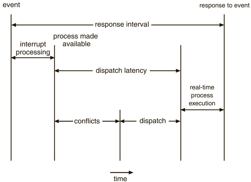
Figure 5.14 Dispatch latency.
