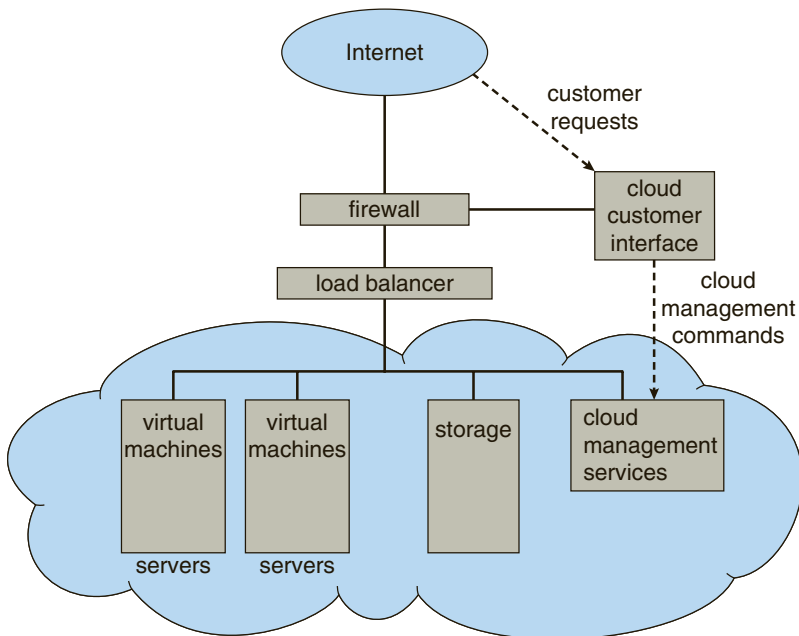
Figure 1.21 Cloud computing.
