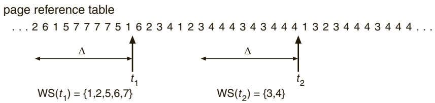
Figure 9.20 Working-set model.
