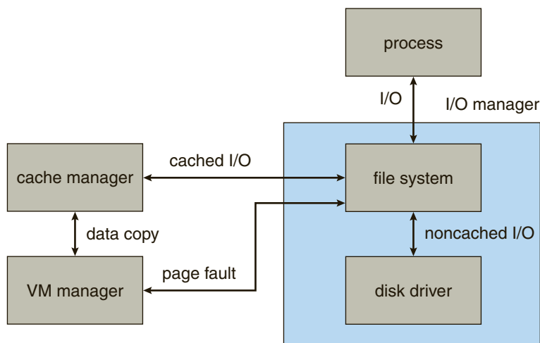
Figure 17.6 File I/O.
