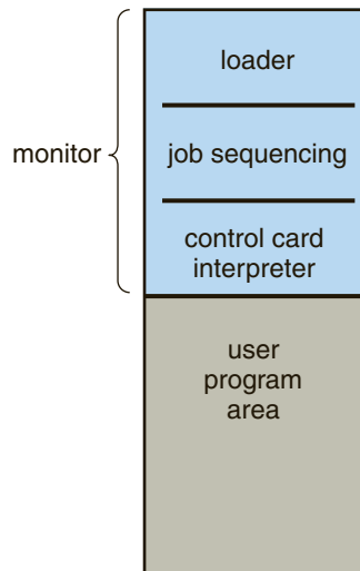
Figure 18.2 Memory layout for a resident monitor.
