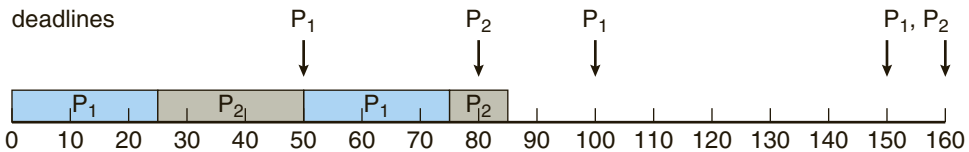
Figure 5.18 Missing deadlines with rate-monotonic scheduling.
