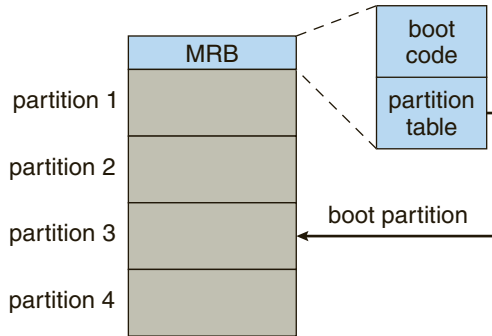
Figure 12.9 Booting from disk in Windows.
