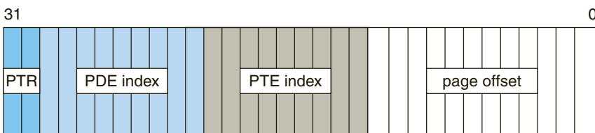
Figure 17.4 Virtual-to-physical address translation on IA-32.
