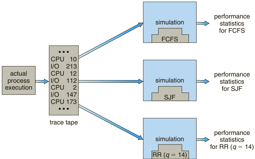
Figure 5.25 Evaluation of CPU schedulers by simulation.
