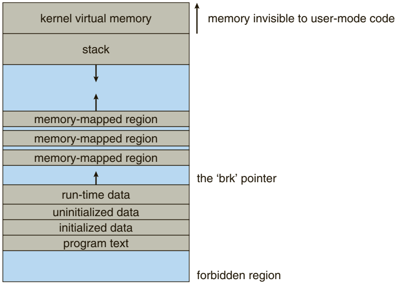
Figure 16.6 Memory layout for ELF programs.
