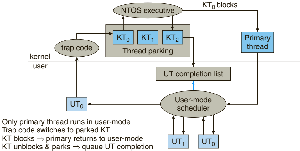
Figure 17.11 User-mode scheduling.
