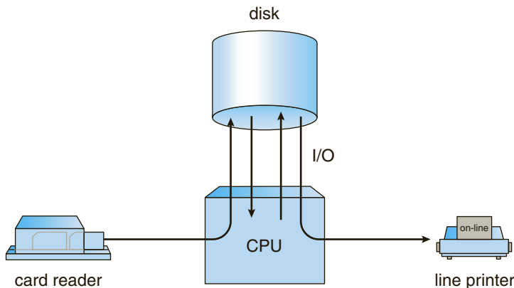
Figure 18.5 Spooling.
