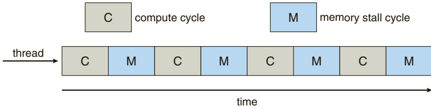
Figure 5.10 Memory stall.
