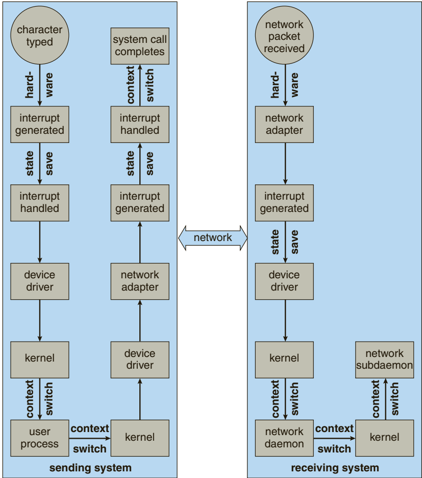
Figure 13.15 Intercomputer communications.
