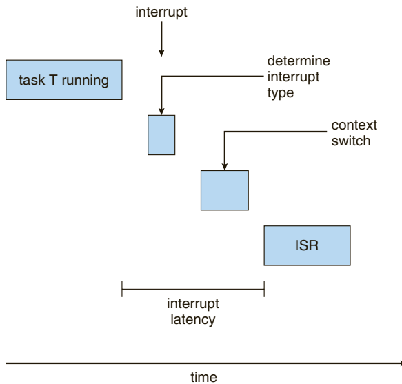
Figure 5.13 Interrupt latency.
