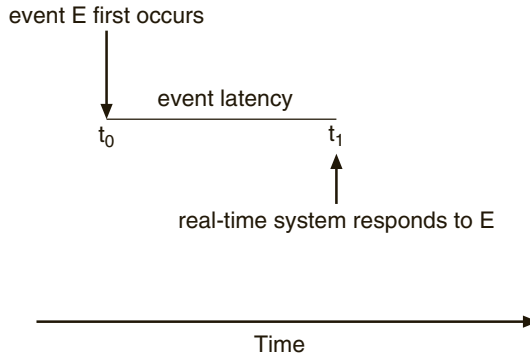
Figure 5.12 Event latency.
