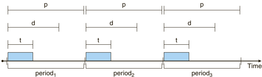
Figure 5.15 Periodic task.
