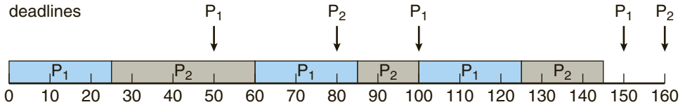
Figure 5.19 Earliest-deadline-first scheduling.
