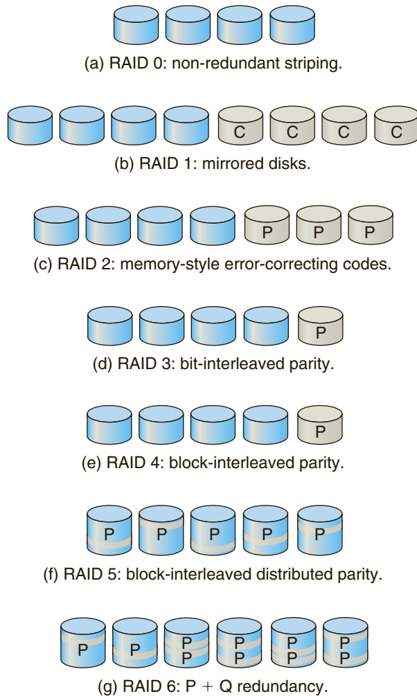
Figure 12.11 RAID levels.
