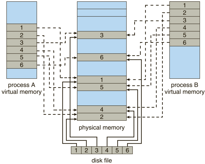
Figure 9.22 Memory-mapped files.
