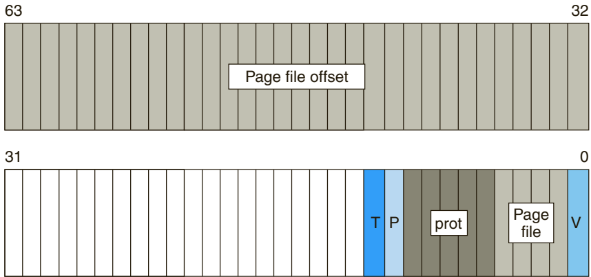
Figure 17.5 Page-file page-table entry. The valid bit is zero.
