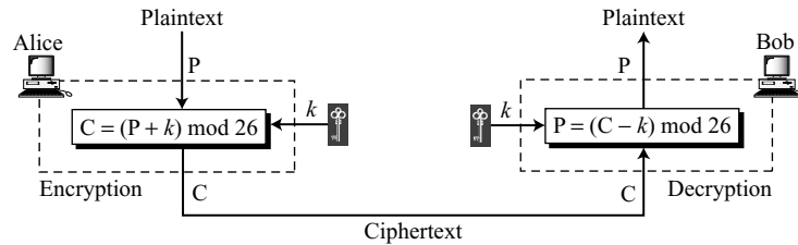
Figure 3.9 Additive cipher
