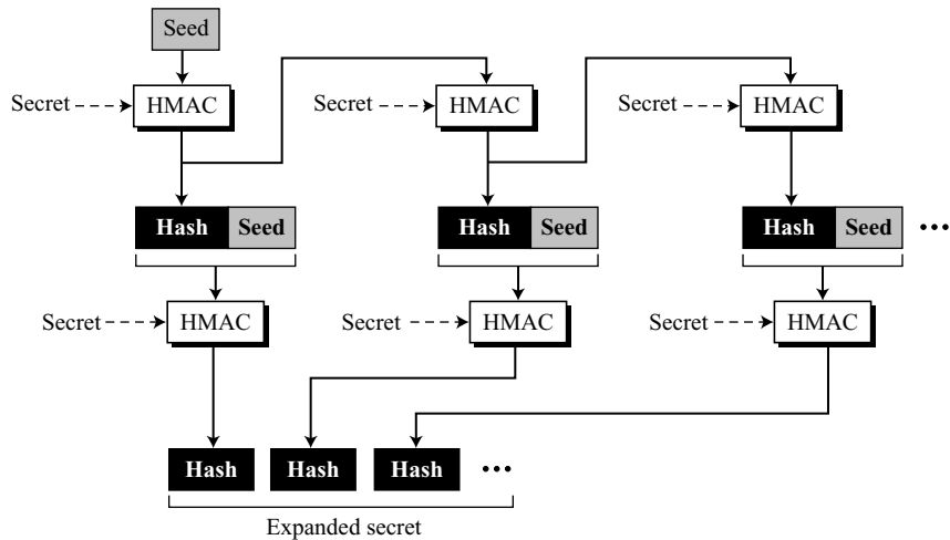
Figure 17.40 Data-expansion function
