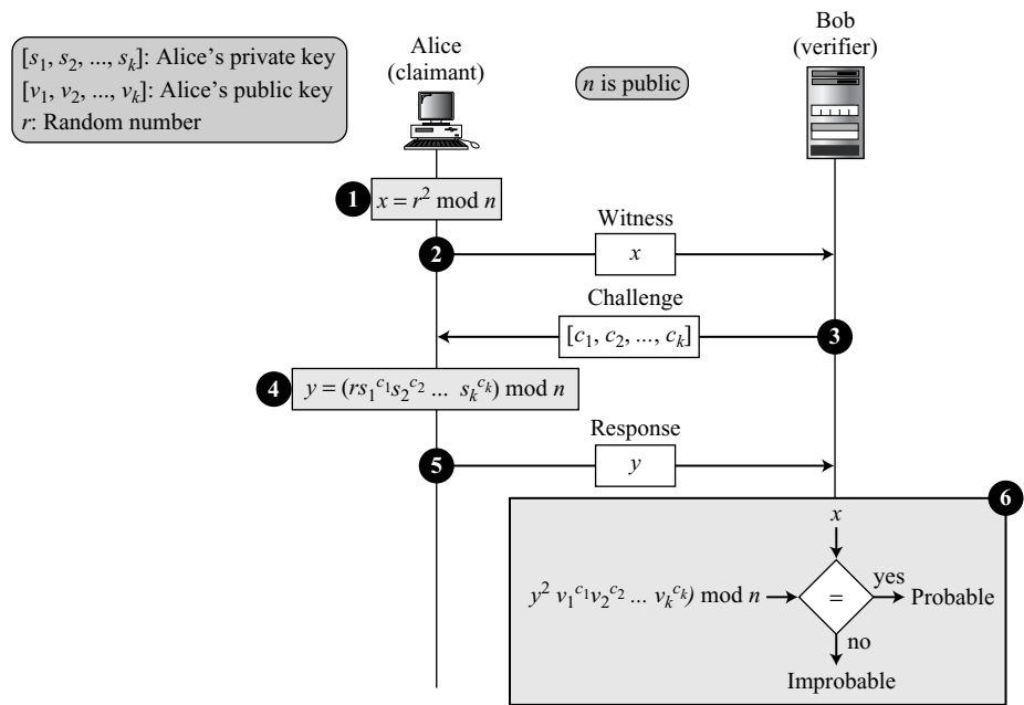
Figure 14.15 Feige-Fiat-Shamir protocol
