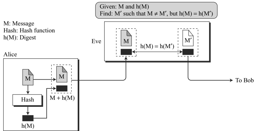
Figure 11.5 Second preimage
