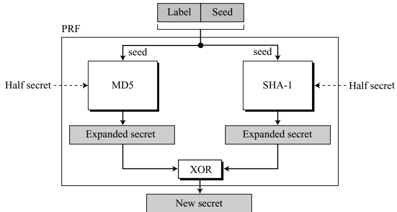
Figure 17.41 PRF
