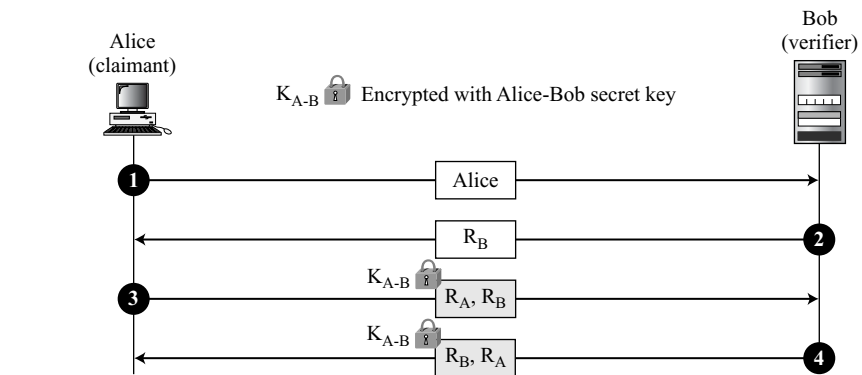
Figure 14.7 Bidirectional authentication
