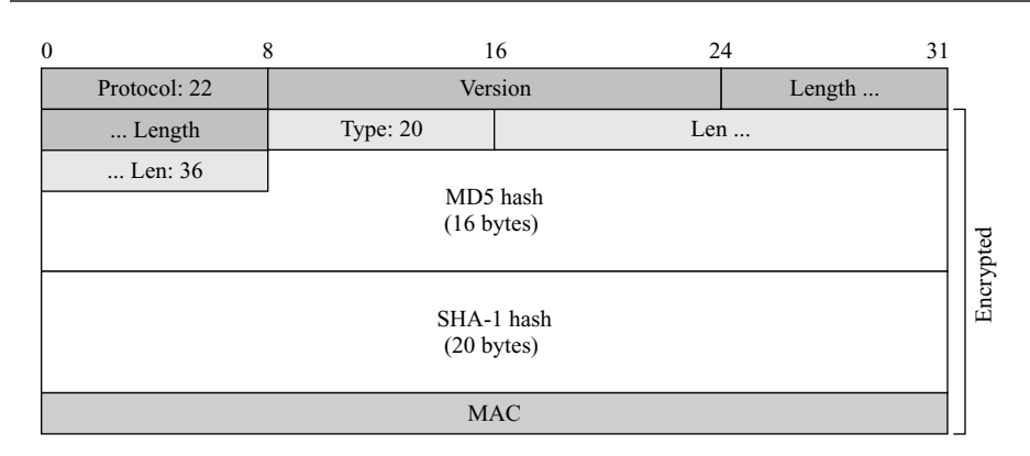
Figure 17.37 Finished message
