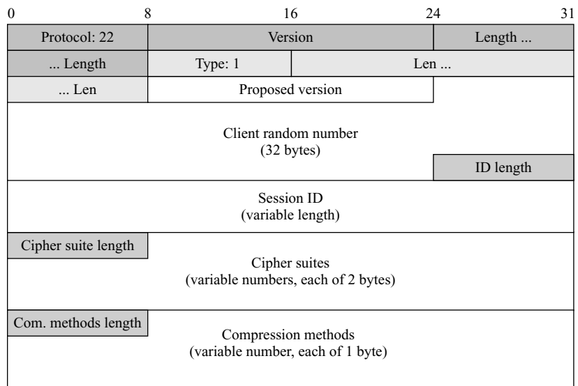
Figure 17.28 ClientHello message
