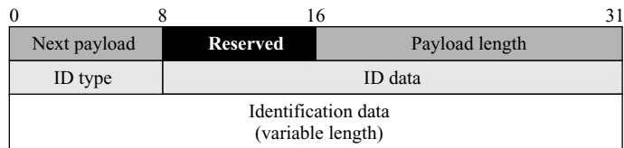
Figure 18.35 Identification payload
