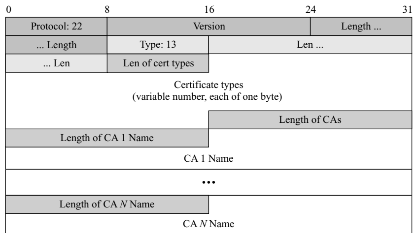
Figure 17.32 CertificateRequest message
