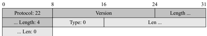
Figure 17.27 HelloRequest message
