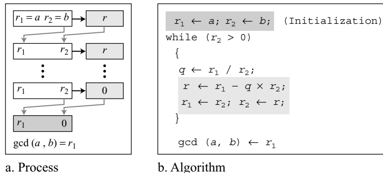
Figure 2.7 Euclidean algorithm
