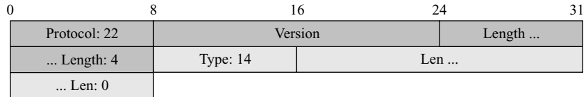
Figure 17.33 ServerHelloDone message
