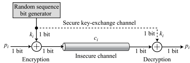
Figure 5.22 One-time pad
