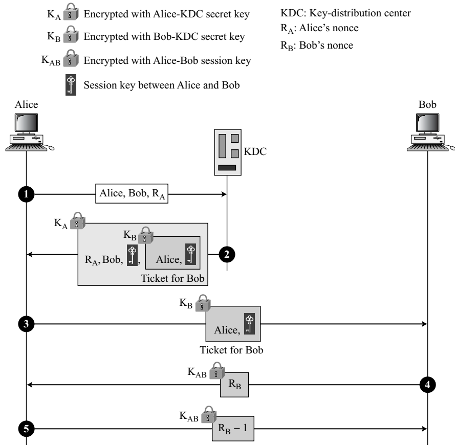
Figure 15.5 Needham-Schroeder protocol
