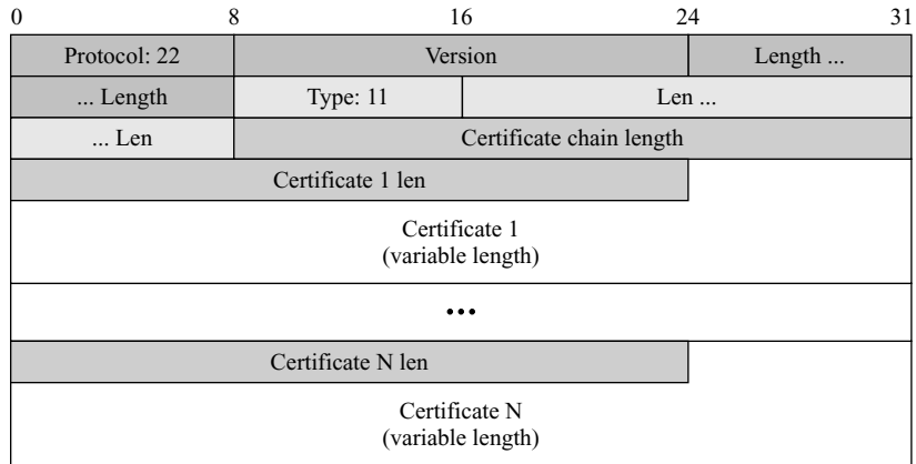
Figure 17.30 Certificate message
