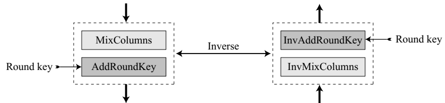
Figure 7.19 Invertibility of MixColumns and AddRoundKey combinations
