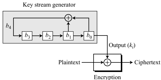
Figure 5.25 LFSR for Example 5.19
