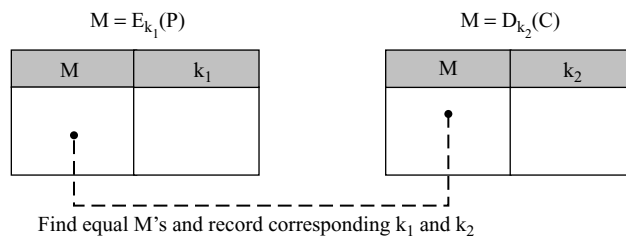
Figure 6.15 Tables for meet-in-the-middle attack
