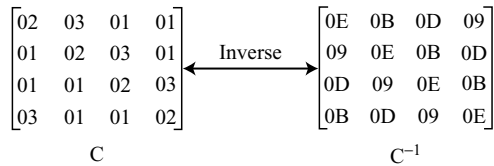
Figure 7.12 Constant matrices used by MixColumns and InvMixColumns
