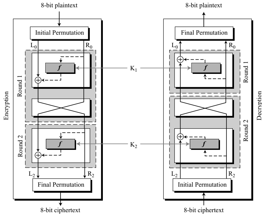
Figure O.9 S-DES cipher and reverse cipher
