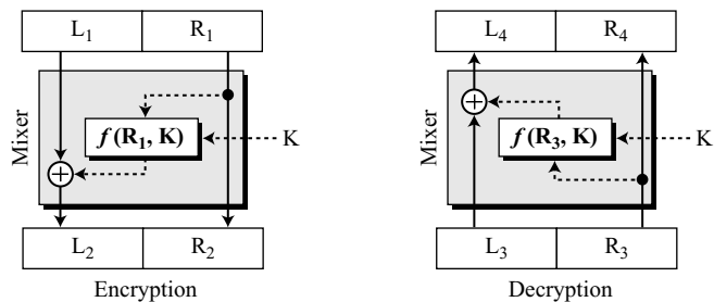
Figure 5.16 Improvement of the previous Feistel design
