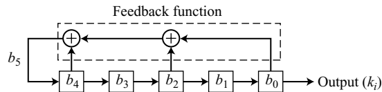
Figure 5.24 LFSR for Example 5.18
