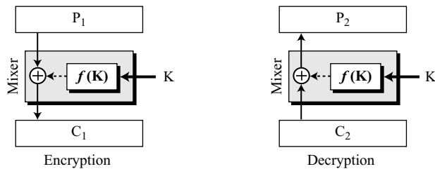
Figure 5.15 The first thought in Feistel cipher design
