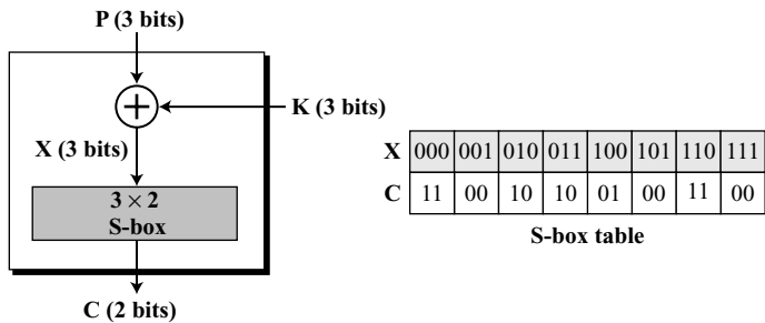
Figure 5.19 Diagram for Example 5.14
