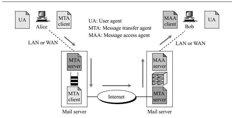
Figure 16.1 E-mail architecture
