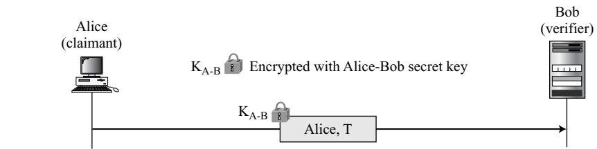
Figure 14.6 Timestamp challenge
