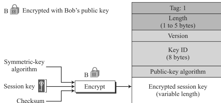
Figure 16.17 Session-key packet
