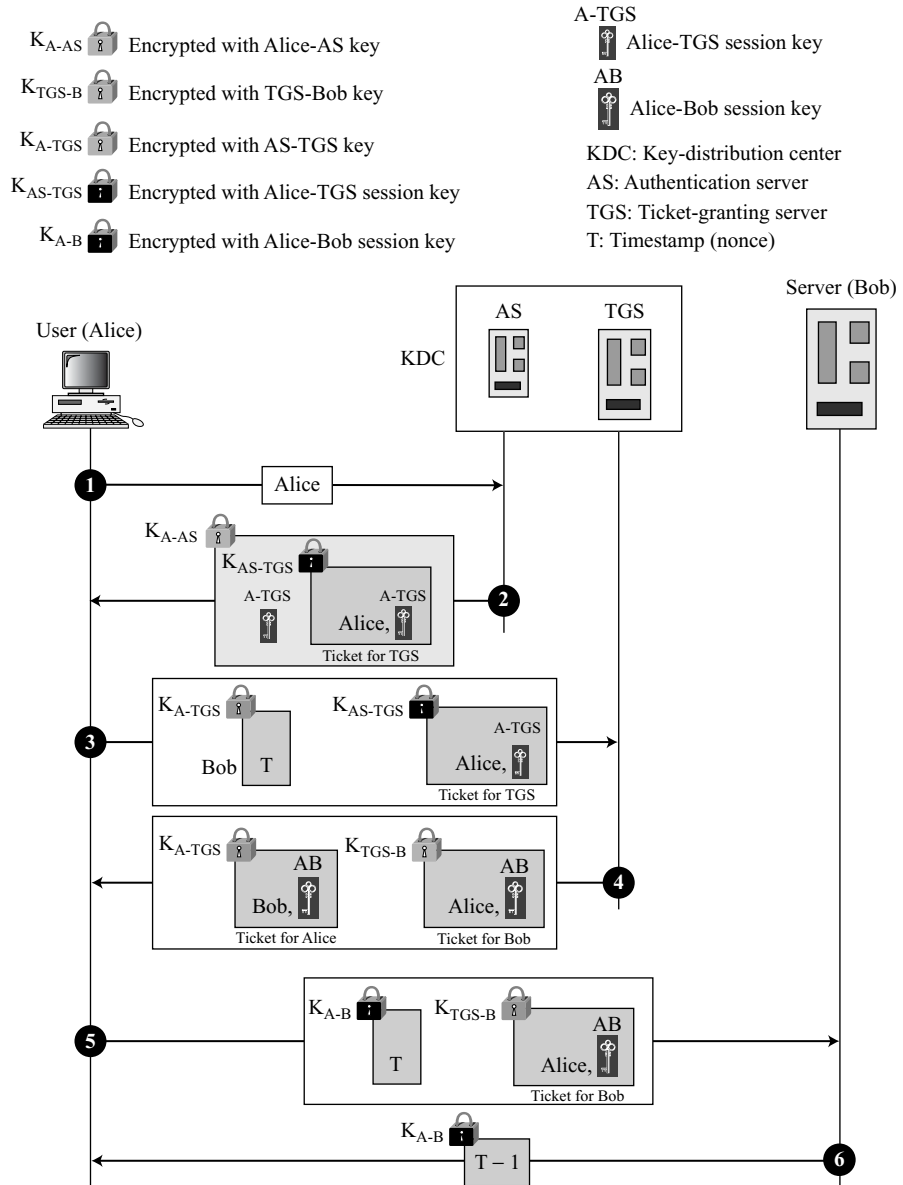
Figure 15.8 Kerberos example
