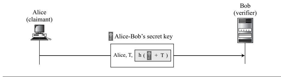
Figure 14.8 Keyed-hash function
