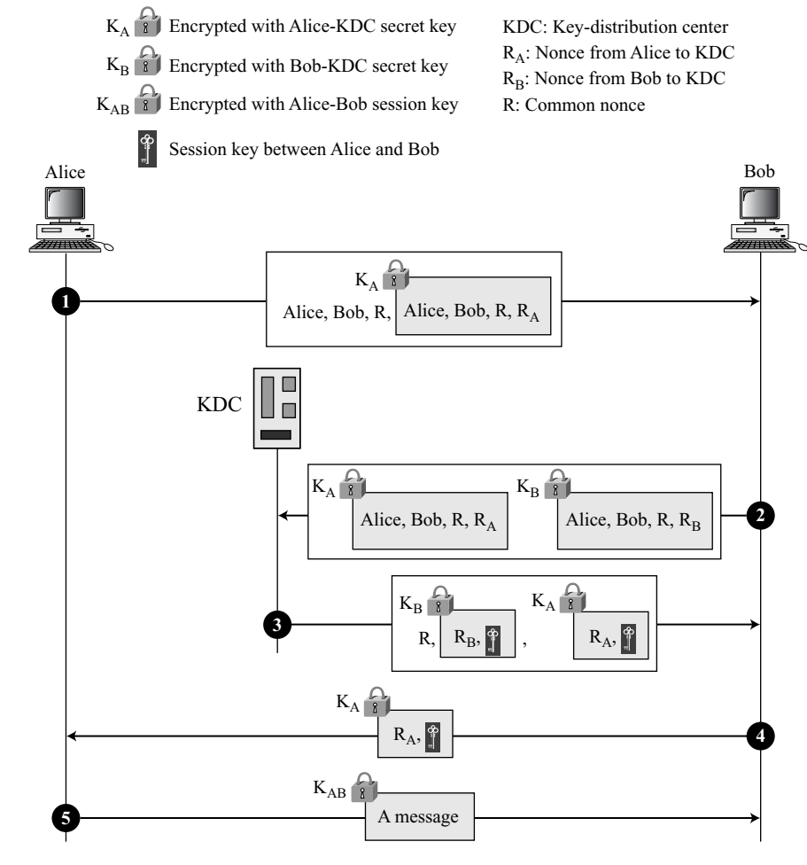
Figure 15.6 Otway-Rees protocol
