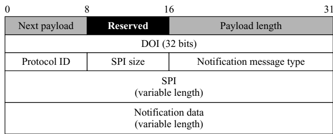
Figure 18.41 Notification payload
