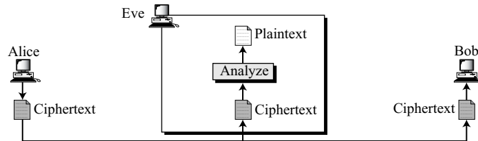
Figure 3.4 Ciphertext-only attack
