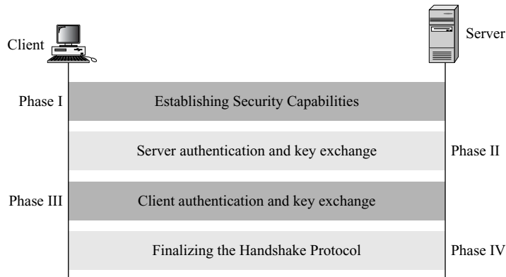
Figure 17.13 Handshake Protocol
