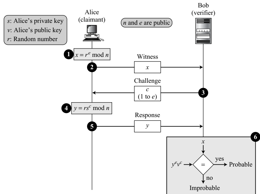
Figure 14.16 Guillou-Quisquater protocol
