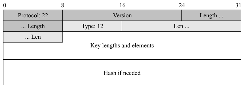
Figure 17.31 ServerKeyExchange message
