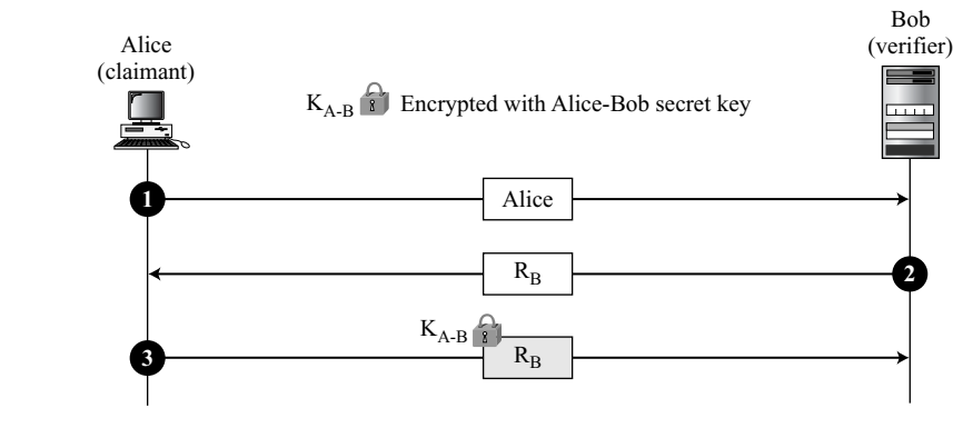
Figure 14.5 Nonce challenge
