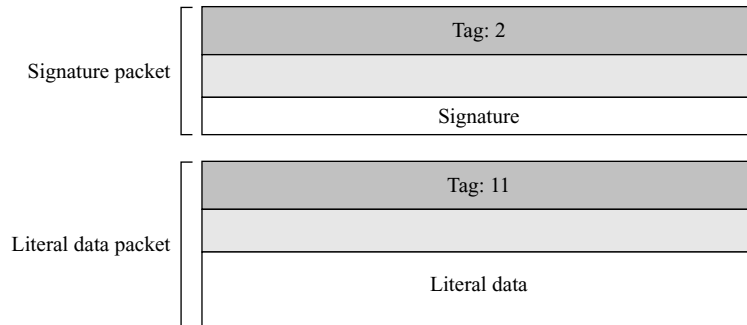
Figure 16.21 Signed message
