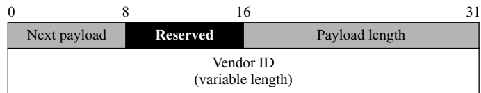
Figure 18.43 Vendor payload
