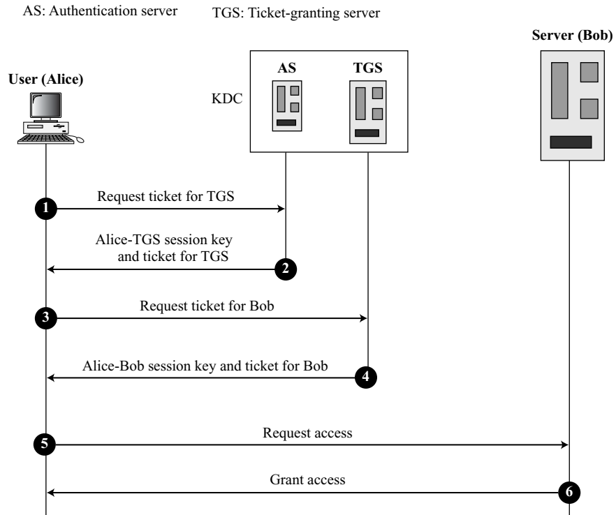
Figure 15.7 Kerberos servers
