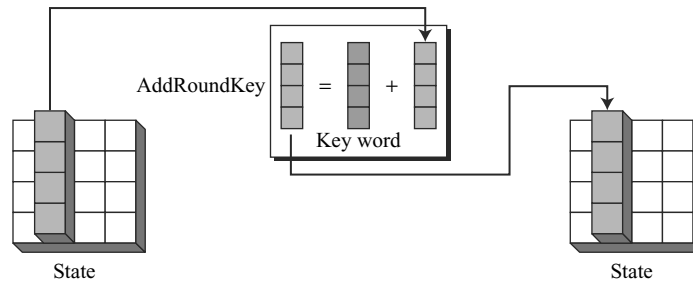
Figure 7.15 AddRoundKey transformation
