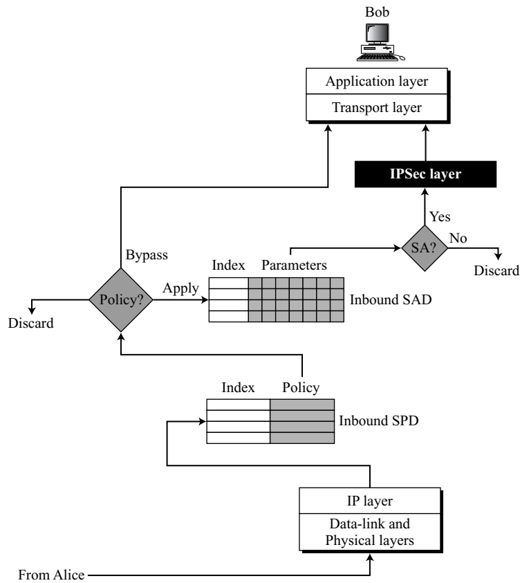
Figure 18.14 Inbound processing
