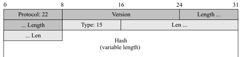
Figure 17.34 CertificateVerify message
