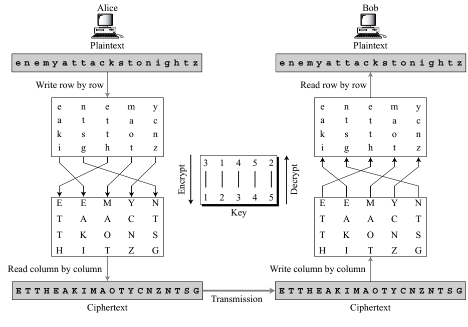
Figure 3.21 Example 3.27
