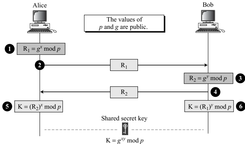
Figure 15.9 Diffie-Hellman method
