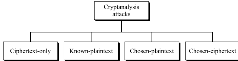
Figure 3.3 Cryptanalysis attacks
