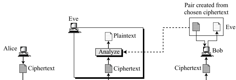
Figure 3.7 Chosen-ciphertext attack
