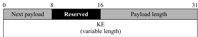
Figure 18.34 Key-exchange payload
