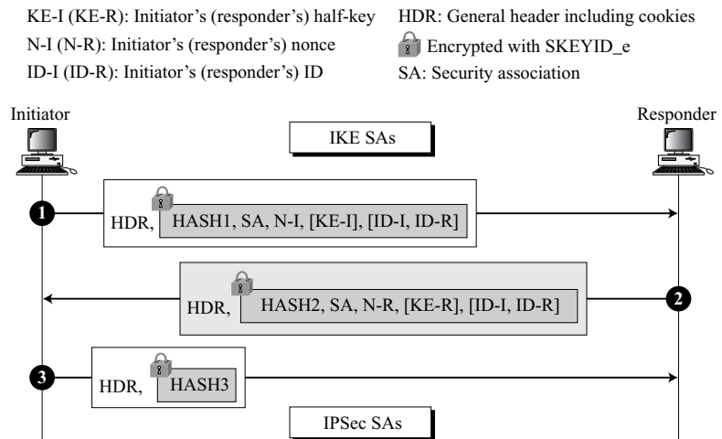
Figure 18.28 Quick mode
