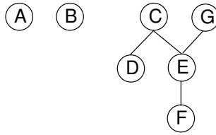
Figure 15.1 Illustration of using a poset to model our current knowledge of the relationships among a collection of objects. A directed acyclic graph (DAG) is used to draw the poset (assume all edges are directed downward). In this example, our knowledge is such that we don't know how A or B relate to any of the other objects. However, we know that both C and G are greater than E and F . Further, we know that C is greater than D , and that E is greater than F .
