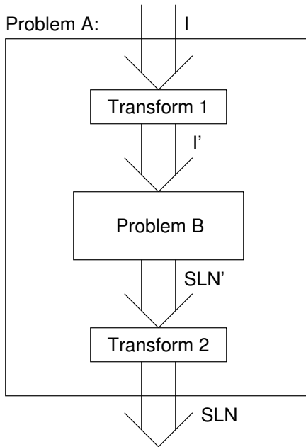
Figure 17.2 The general process for reduction shown as a “blackbox” diagram.
