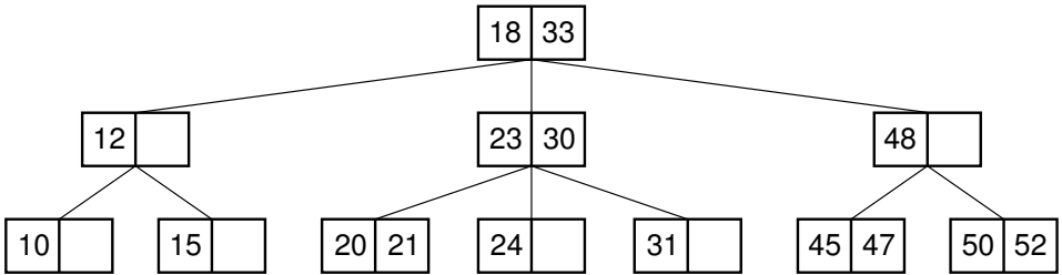
Figure 10.9 A 2-3 tree.
