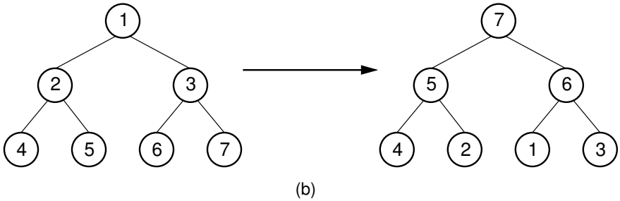
Figure 5.20 Two series of exchanges to build a max-heap. (a) This heap is built by a series of nine exchanges in the order (4-2), (4-1), (2-1), (5-2), (5-4), (6-3), (6-5), (7-5), (7-6). (b) This heap is built by a series of four exchanges in the order (5-2), (7-3), (7-1), (6-1).
